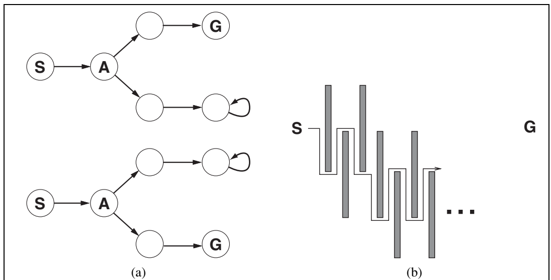
Figure 4.20 (a) Two state spaces that might lead an online search agent into a dead end. Any given agent will fail in at least one of these spaces. (b) A two-dimensional environment that can cause an online search agent to follow an arbitrarily inefficient route to the goal. Whichever choice the agent makes, the adversary blocks that route with another long, thin wall, so that the path followed is much longer than the best possible path.
