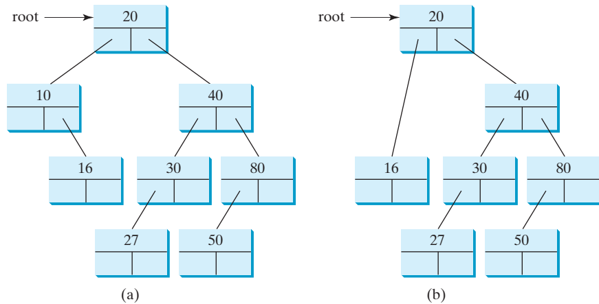
FIGURE 25.9 Case 1: Deleting node 10 from (a) results in (b).
