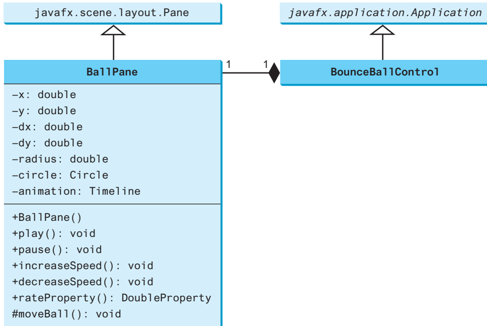
FIGURE 15.24 BounceBallControl1 contains BallPane .
