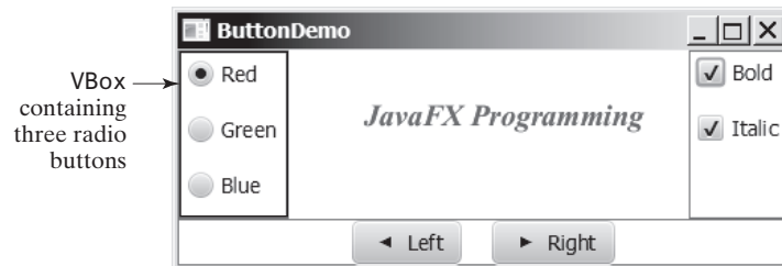
FIGURE 16.10 The program demonstrates using radio buttons. Source: Copyright © 1995–2016 Oracle and/or its affiliates. All rights reserved. Used with permission.
