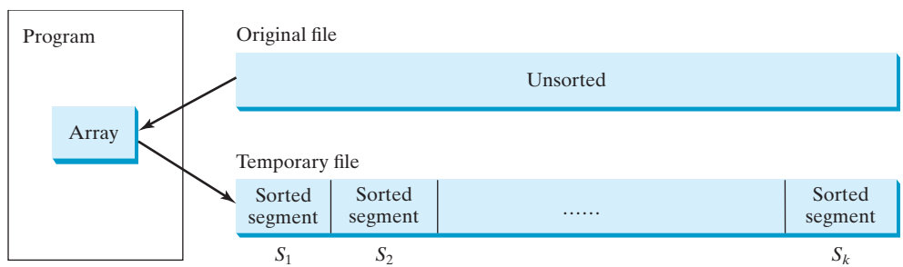
FIGURE 23.17 The original file is sorted in segments.
