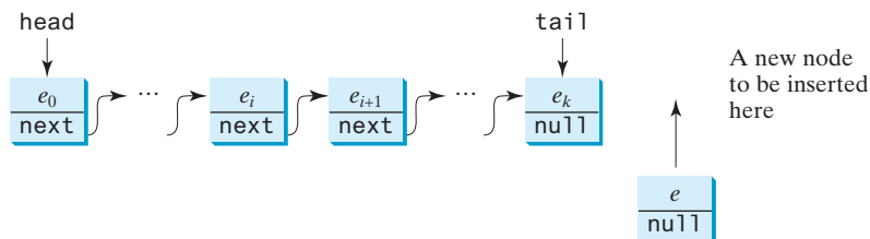
(a) Before a new node is inserted.
