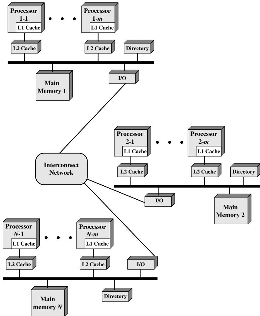
Figure 17.13 CC-NUMA Organization
