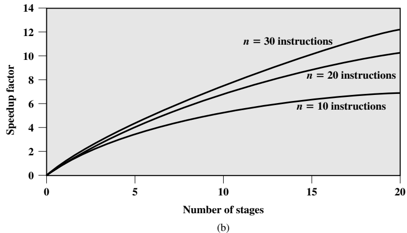
Figure 12.14 Speedup Factors with Instruction Pipelining
