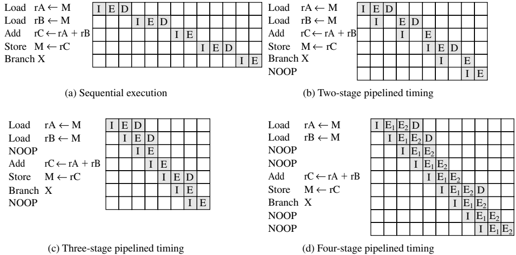
Figure 13.6 The Effects of Pipelining
