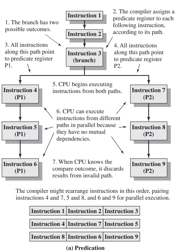
Figure 21.3 IA-64 Predication and Speculative Loading
