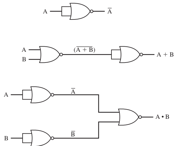
Figure 20.3 The Use of NOR Gates
