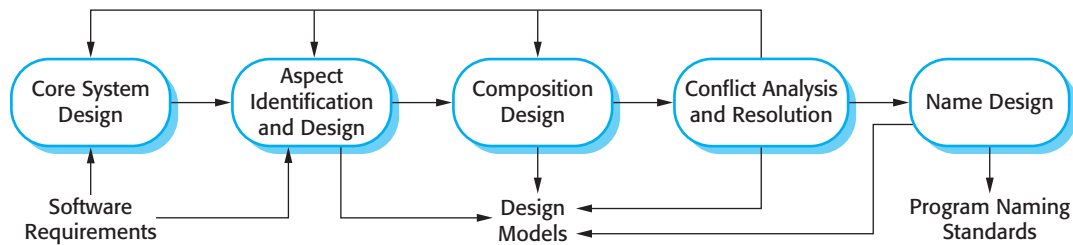
Figure 21.13 A generic aspect-oriented design process Developing an effective process for aspect-oriented design is essential if aspect-oriented design is to be accepted and used. I suggest that an aspect-oriented design process should include the activities shown in Figure 21.13. These activities are:
