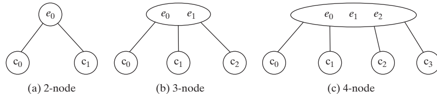
FIGURE 42.1 An interior node of a 2-4 tree has two, three, or four children.
