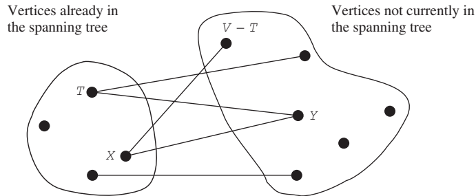
FIGURE 29.6 Find a vertex x in T that connects a vertex y in V - T with the smallest weight.
