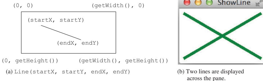
FIGURE 14.29 A Line object is created to display a line.
