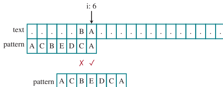
FIGURE 22.13 B does not match C. B first matches pattern[2] in the remaining part of the pattern from right to left, slide the pattern to align B in the text with pattern[2].
