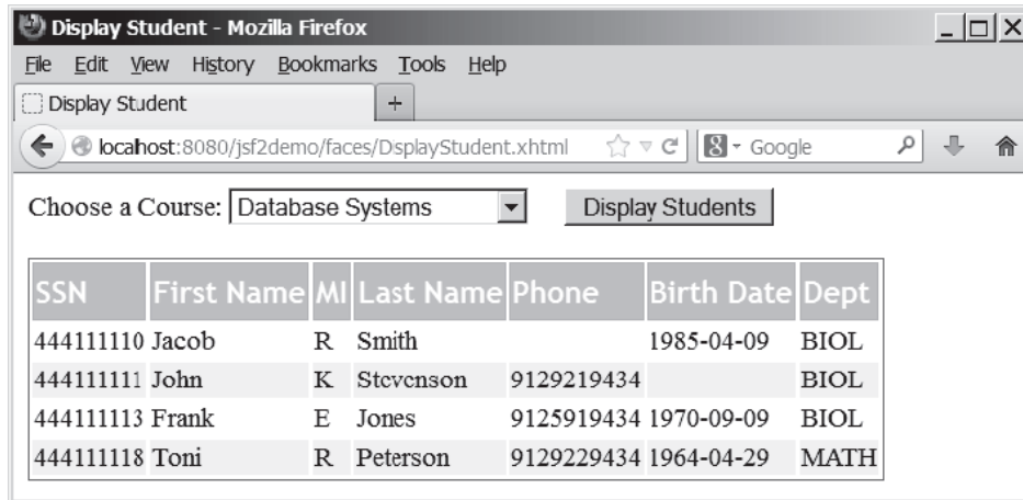
FIGURE 39.19 The table displays the students enrolled in the course.
