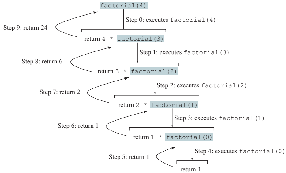
FIGURE 18.2 Invoking factorial(4) spawns recursive calls to factorial .
