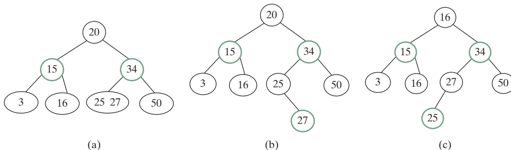
FIGURE 43.3 The conversion from a 2-4 tree to a red-black tree is not unique.
