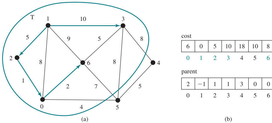
FIGURE 29.16 Now vertices \{1, 2, 0, 6, 3\} are in set T .
