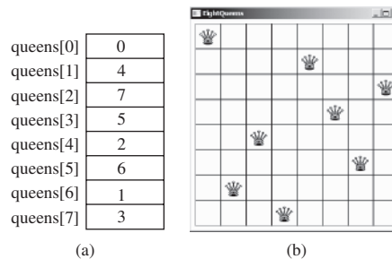
FIGURE 22.6 queens[i] denotes the position of the queen in row i . Source: Copyright © 1995–2016 Oracle and/or its affiliates. All rights reserved. Used with permission.
