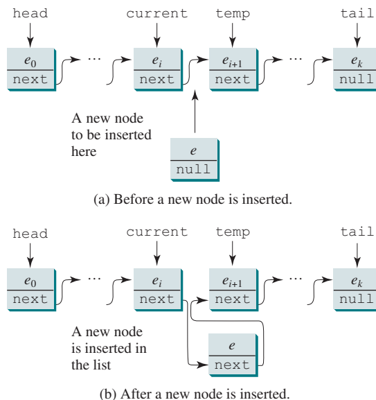
FIGURE 24.14 A new element is inserted in the middle of the list.
