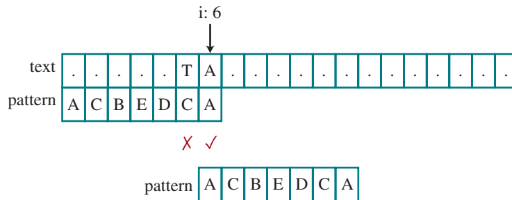
FIGURE 22.12 Since T is not in the remaining of the pattern, slide the pattern passing T and start the next test.
