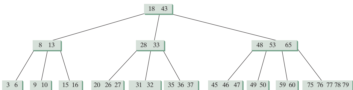
FIGURE 42.16 In a B-tree of order 6, each node except the root may contain between 2 and 5 keys.
