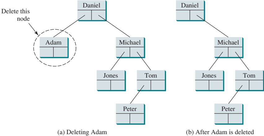
FIGURE 25.14 Deleting Adam falls into Case 1.
