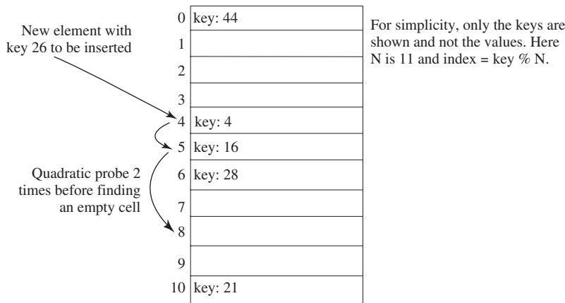
FIGURE 27.4 Quadratic probing increases the next index in the sequence by j^2 for j = 1, 2, 3, \dots
