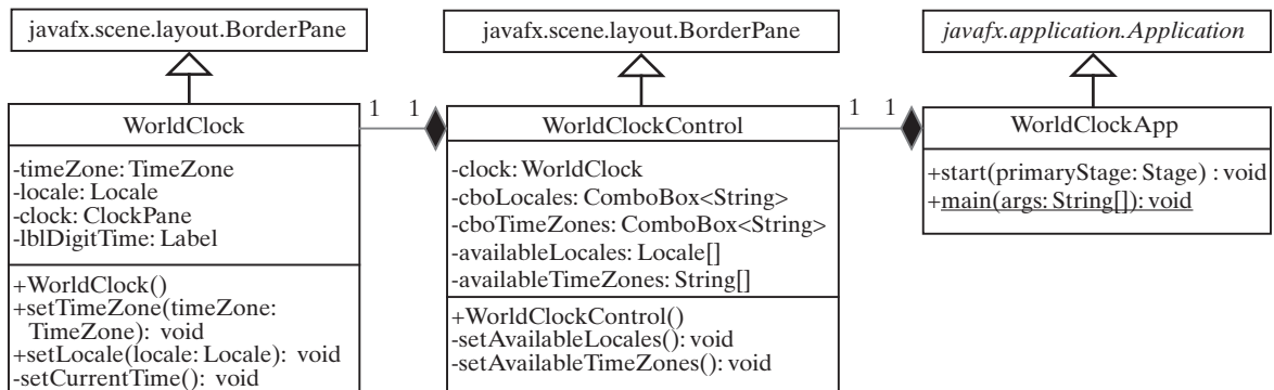
FIGURE 36.5 WorldClockApp contains WorldClockControl , and WorldClockControl contains WorldClock .
