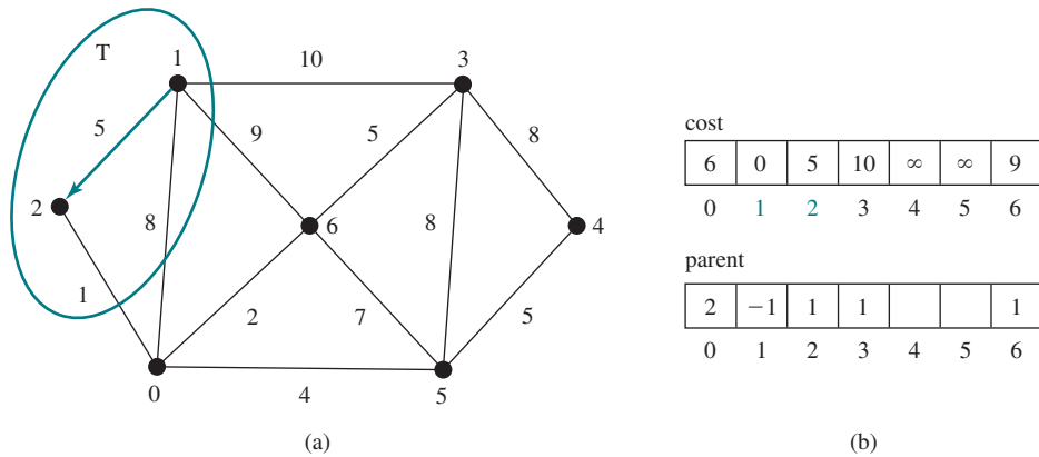
FIGURE 29.13 Now vertices 1 and 2 are in set T.
