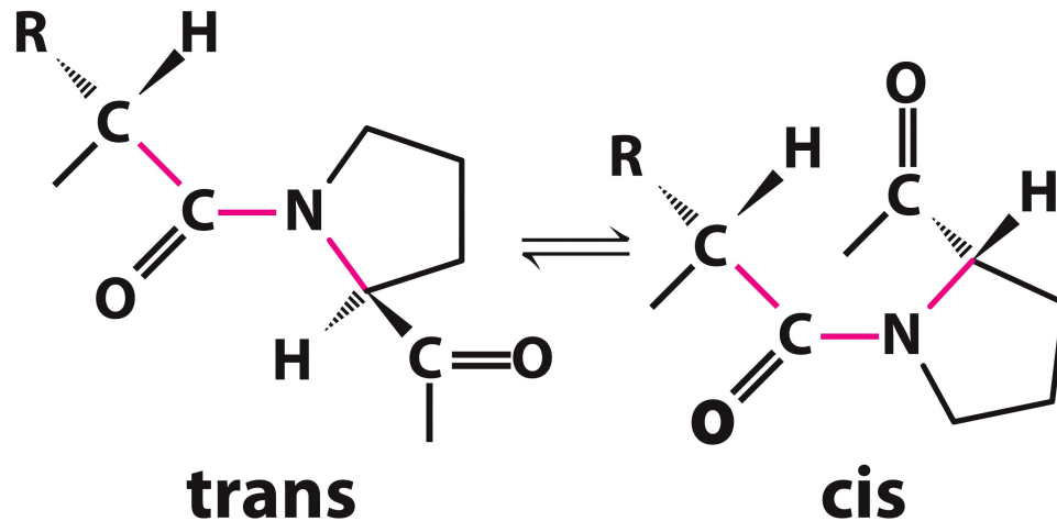
Proline isomers
