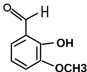
Vanillin
