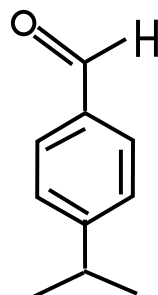
Cuminaldehyde
