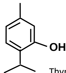
Thymol
