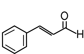
Cinnamaldehyde
