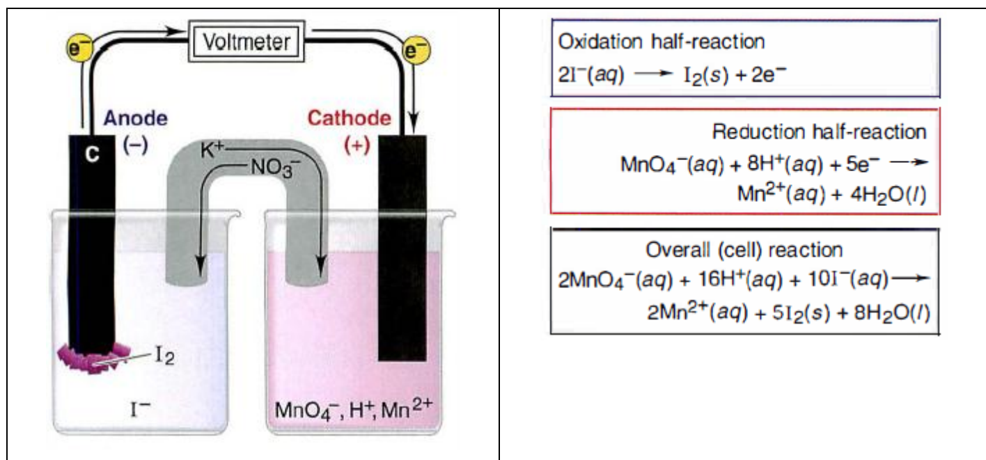
Figure 21.6 A voltaic cell using inactive electrodes. The reaction between \text{I}^- and \text{MnO}_4^- in acidic solution does not have species that can be used as electrodes, so inactive graphite (C) electrodes are used.
