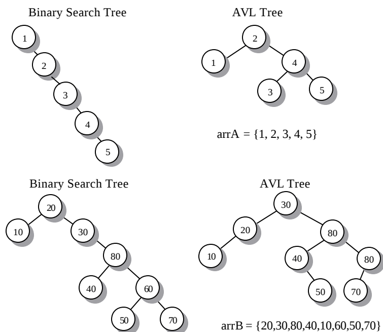
FIGURE 1 Equivalent Binary Search and AVL Trees
