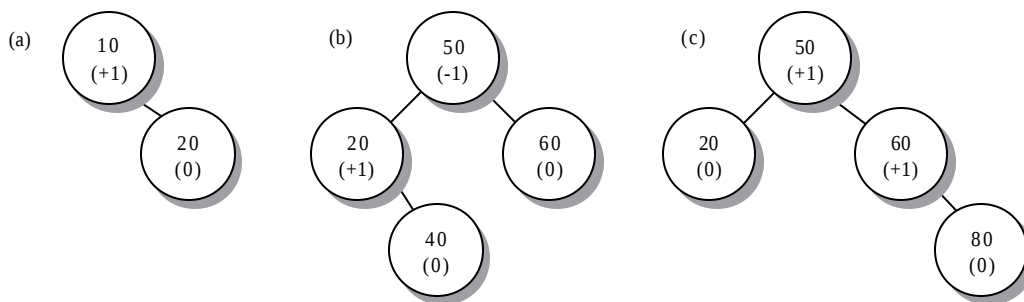
FIGURE 2 AVL trees with balance-factor of each node in parentheses
