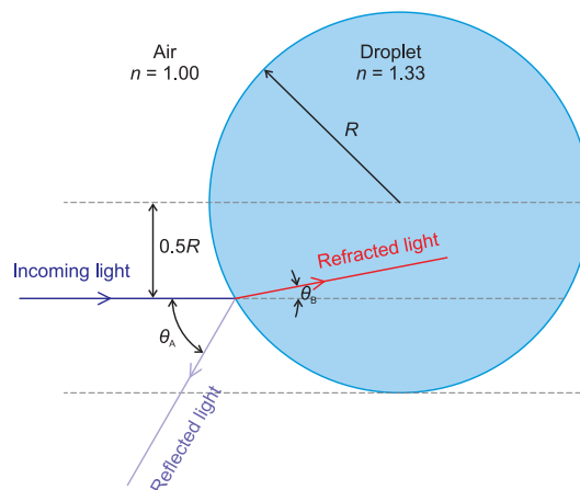
Figure 29.4 A beam of light hits a spherical water droplet.
