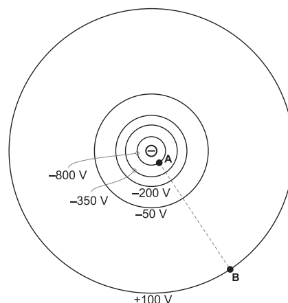
Figure 25.3 Equipotentials around an isolated point charge.
