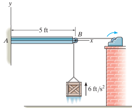
Prob. 13–40
