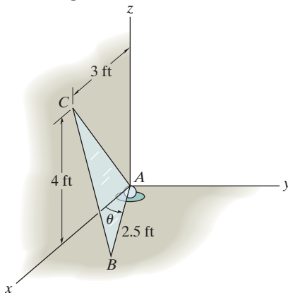
Probs. 20–35/36
