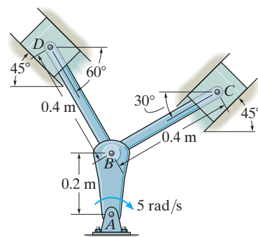
Probs. 16–102/103
