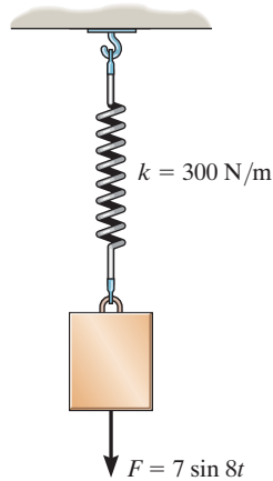
Prob. 22–47
