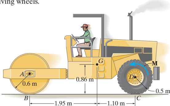
Prob. 19–30
