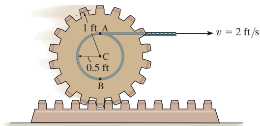
Probs. 16–56/57
