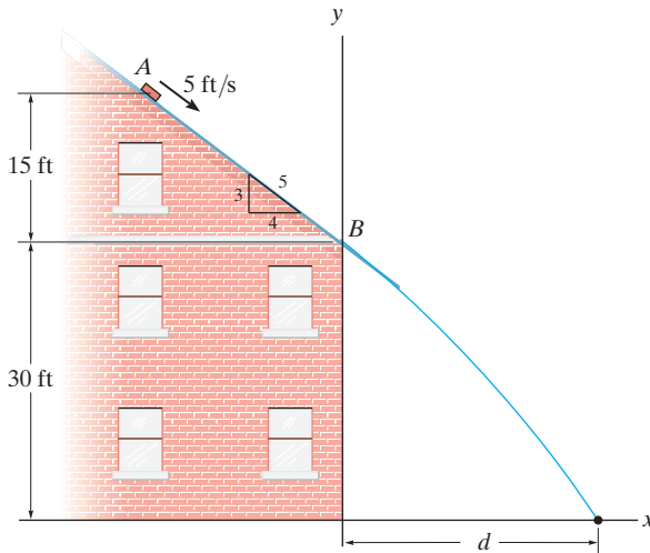
Prob. 14–27
