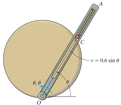
Probs. 13–107/108
