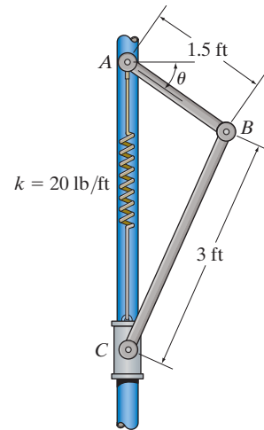
Prob. 18-56
