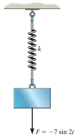
Prob. 22–45
