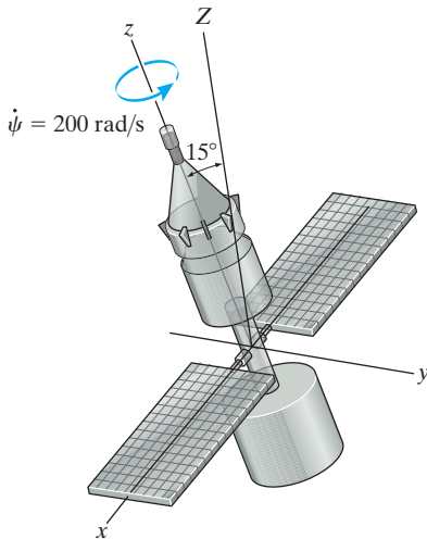
Prob. 21-79
