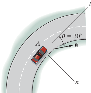
Prob. 12–116
