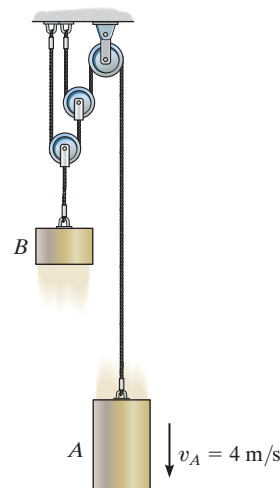
Prob. 12–203
