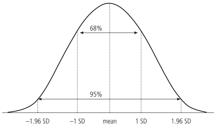
Figure 4.3. The normal distribution curve
