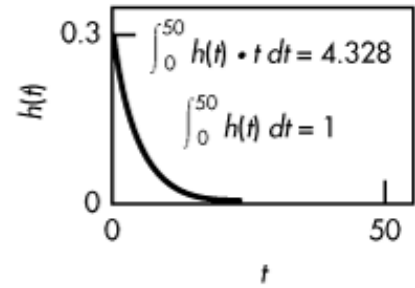
C. Tracer exit rate after normalization
