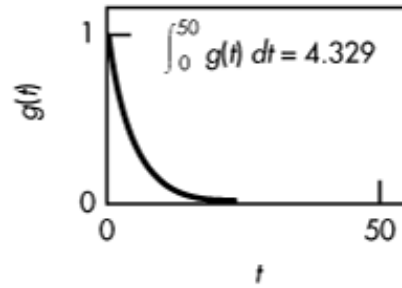
B. Tracer in tank after normalization
