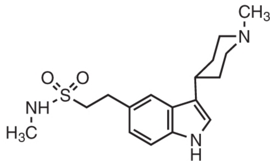
Naratriptan
