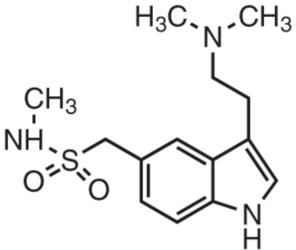
Sumatriptan
