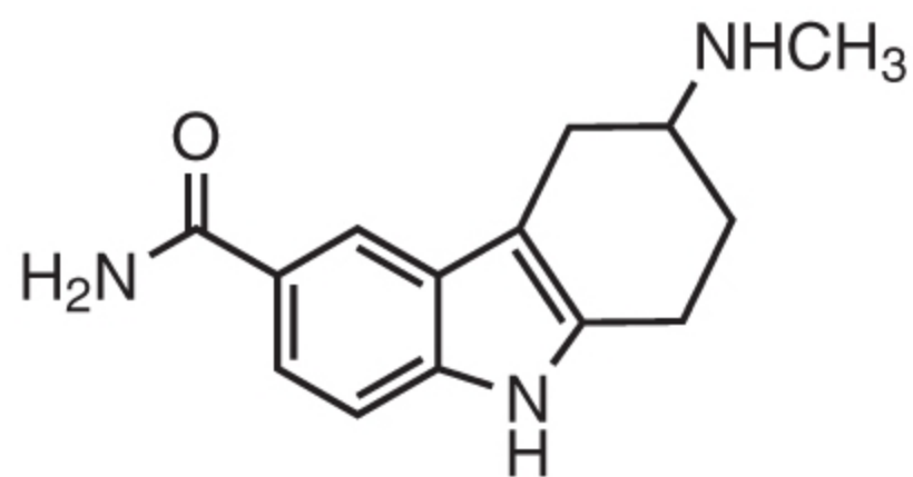
Frovatriptan
