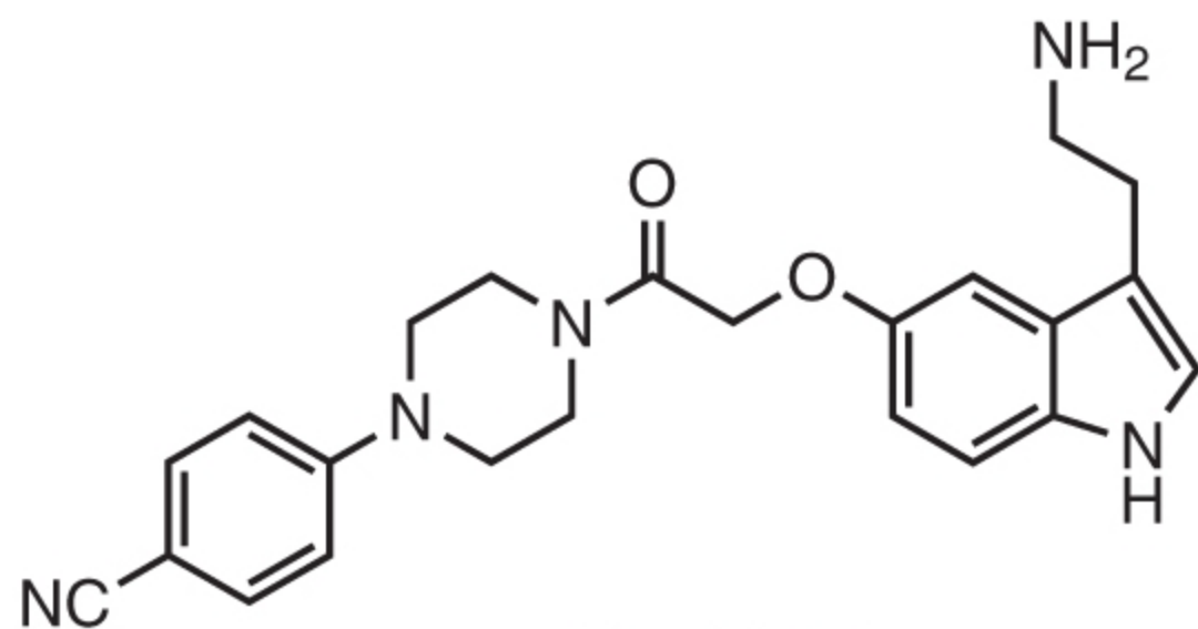
Donitriptan
