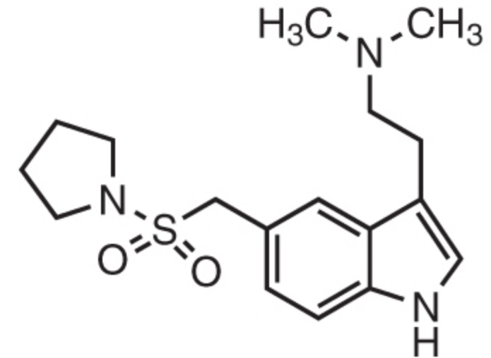
Almotriptan
