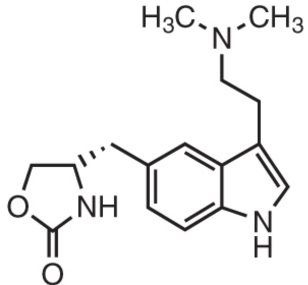
Zolmitriptan
