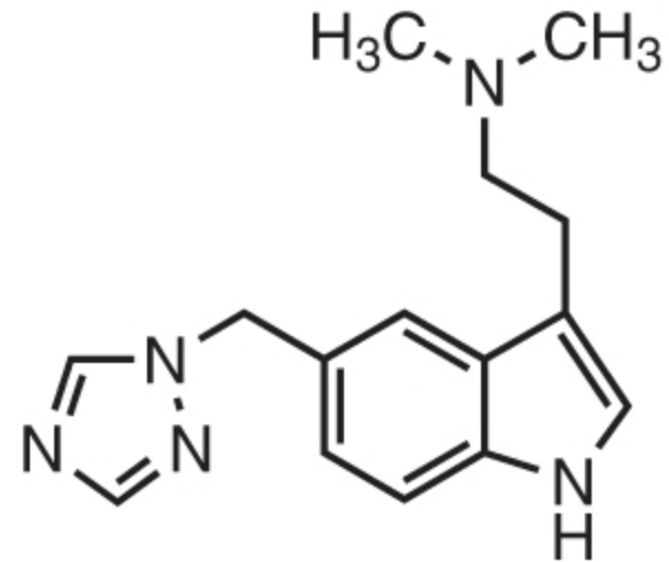
Rizatriptan
