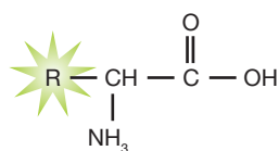
FIGURE 3.1 Generic amino acid structure.
