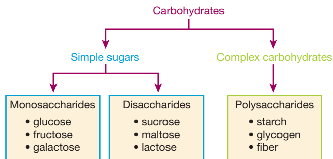
■ FIGURE 2.1 Carbohydrate classifications.
