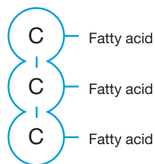
■ FIGURE 4.1 Generic triglyceride molecule.
