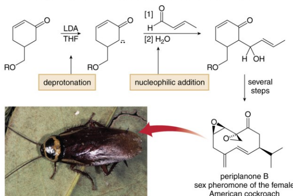
Figure 24.4 A directed aldol reaction in the synthesis of periplanone B
