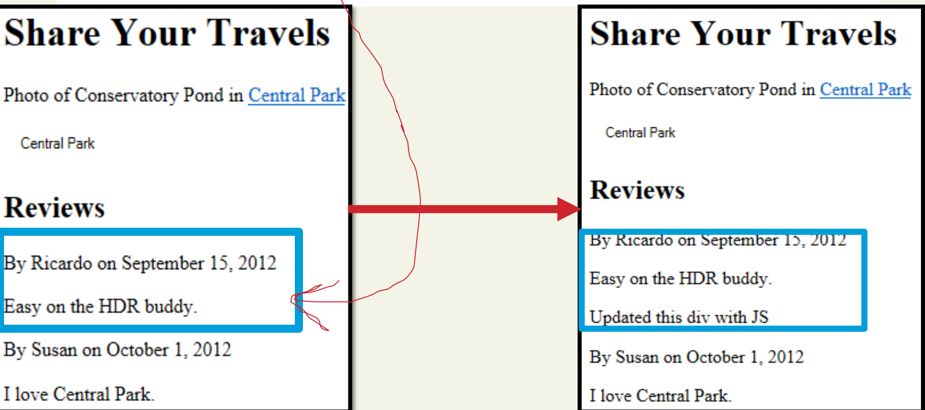
LISTING 6.8 Changing the HTML using innerHTML
