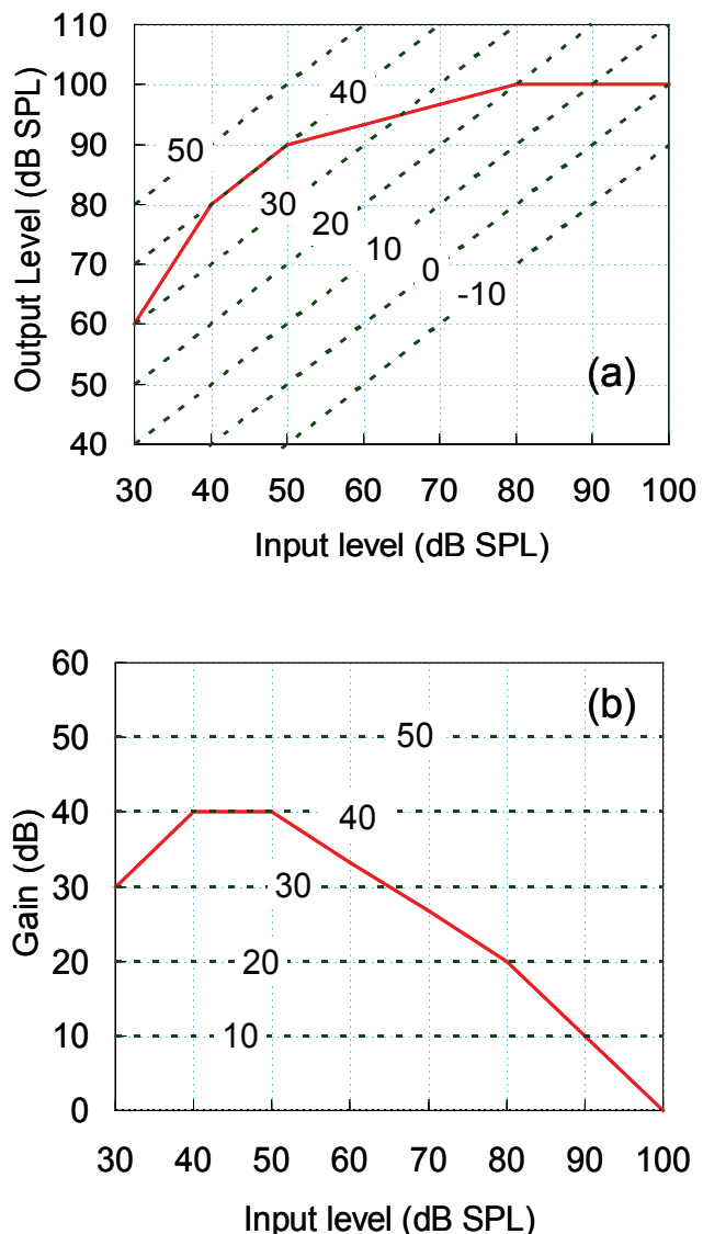
Figure 4.6 (a) Input-output diagram of a non-linear hearing aid at 2 kHz (solid red line) and lines of constant gain (dotted lines). (b) Gain-input diagram of the same amplification characteristics.
