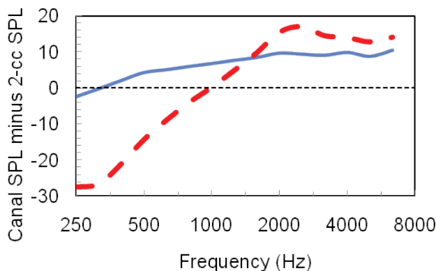
Figure 4.8 RECD: SPL generated in the average adult real ear canal minus SPL generated in an HA1 2-cc coupler. Data for the occluded ear (solid line) are averaged across three experiments. 1277, 1283, 1286 Data for the open canal fitting (dashed line) were measured in KEMAR relative to the SPL in an HA1 2-cc coupler.
