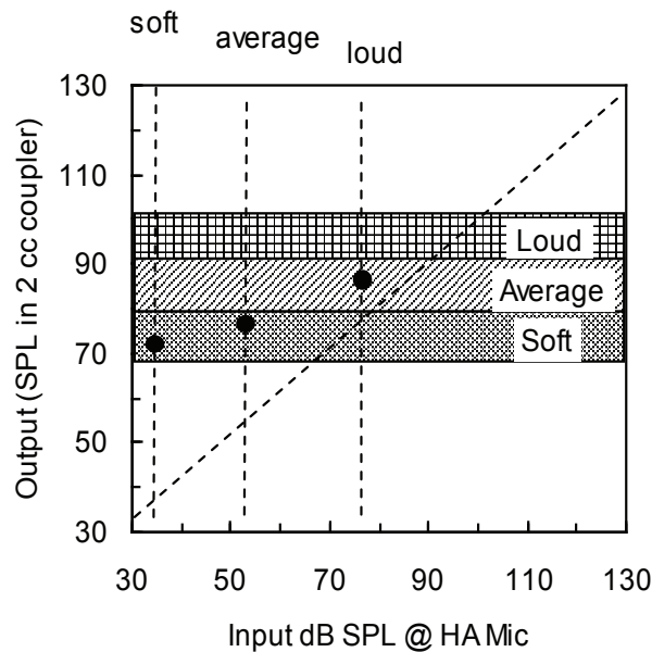
Figure 10.7 An example of the three-point I-O curve, for a frequency of 2 kHz, prescribed by the VIOLA software on the basis of the IHAFF procedure.
