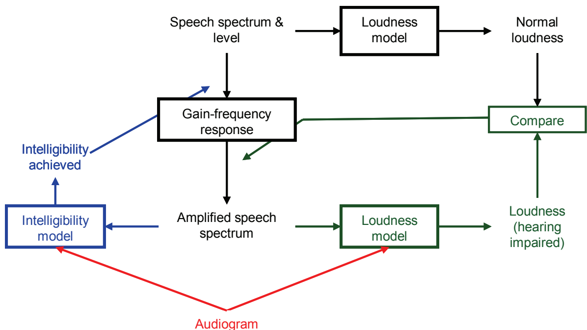
Figure 10.11 The NAL-NL derivation process. The loop on the left (shown in blue) varies the gain-frequency response to maximize speech intelligibility, but subject to the overall loudness not exceeding that for a normal-hearing person listening to the same speech, as calculated by the loop on the right (shown in green). We can think of this as the left loop turning up the gain one frequency at a time, but the right loop turning down the volume control whenever the overall loudness is greater than normal. Both the intelligibility model and the loudness model are adjusted to match the audiogram for which the gain-frequency response is being calculated.
