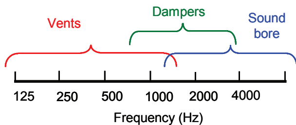
Figure 5.8 Frequency regions affected by each of the components of the hearing aid coupling system.
