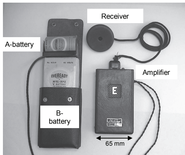
Figure 1.13 A relatively late vacuum tube hearing aid, with its two separate batteries.
