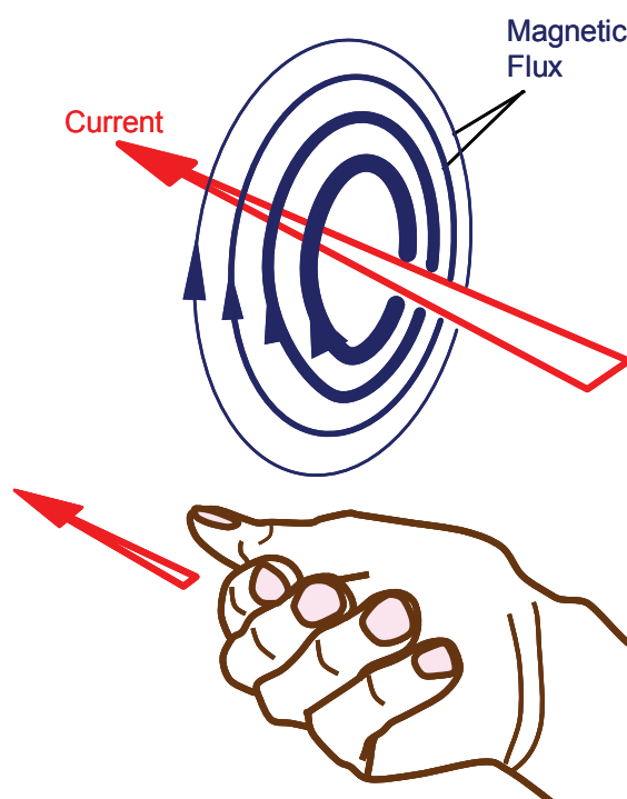
Figure 3.4 Lines of magnetic flux flowing around a conductor carrying a current and the right hand rule showing how the curled fingers help to visualise the direction of the magnetic field caused by current flowing in the direction in which the thumb points.
