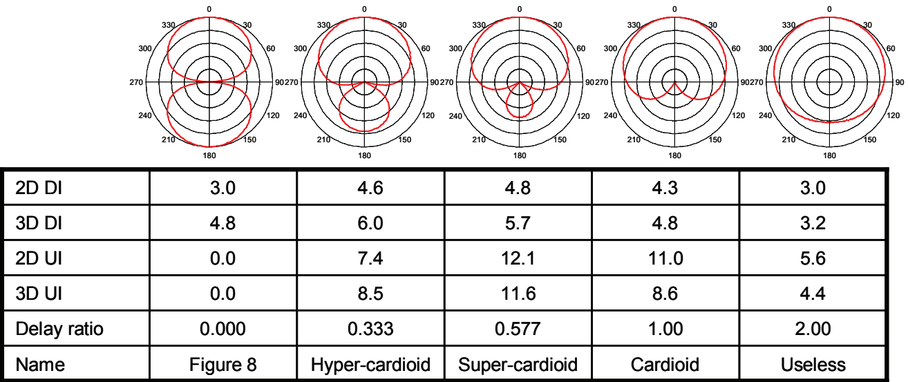
Figure 7.2 Theoretical polar sensitivity patterns of subtractive first-order directional microphones when not mounted on the head for various values of the ratio of internal delay to external delay. The table shows the 2D and 3D DIs, and the 2D and 3D unidirectional index, for each pattern. Each concentric circle represents a 5 dB change in sensitivity.
