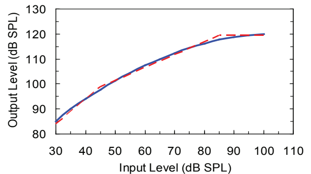
Figure 6.6 Input-output characteristics corresponding to curvilinear compression (blue solid line) and a fixed compression ratio combined with compression limiting (red dashed line).
