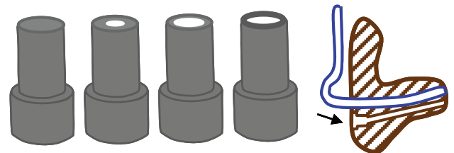
Figure 5.10 The inserts (larger than life-size) from a vent insert system, and the earmold and vent receptacle (approximately life-size) into which they fit. Positive Venting Valve (PVV) and Select-A-Vent (SAV) are two such systems commercially available.
