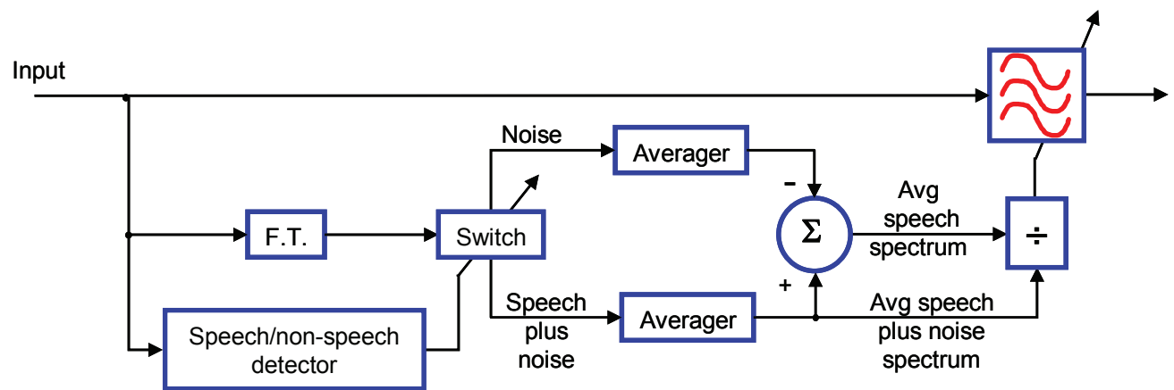
Figure 8.2 A Wiener Filter incorporating a Fourier Transform (F.T.) to calculate the spectrum of the combined speech and noise. A speech/non-speech detector classifies the spectrum as noise or speech plus noise, and thus enables the average spectral power of the speech to be estimated.
