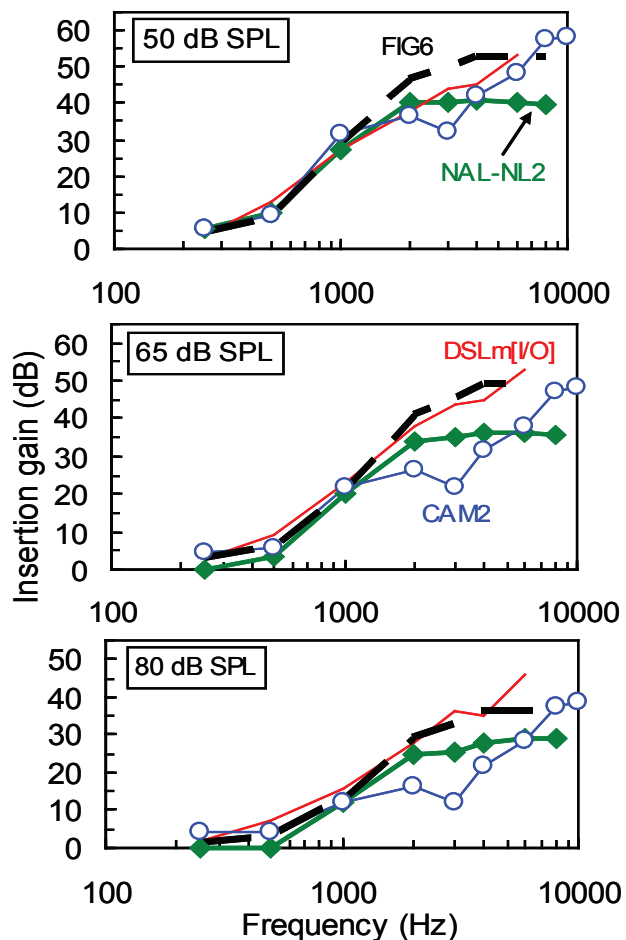
Figure 10.13 Same as Figure 10.12, except it is for the sloping hearing loss shown in Figure 10.4.
