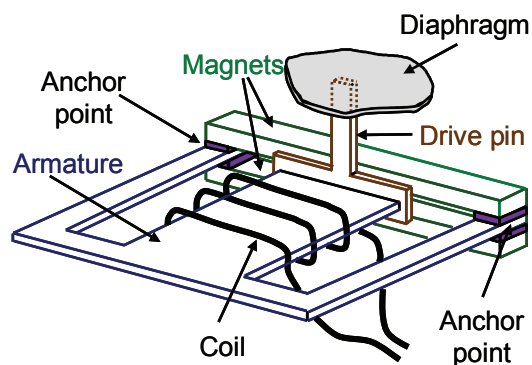
Figure 2.18 Principle of operation of the moving coil receiver.
