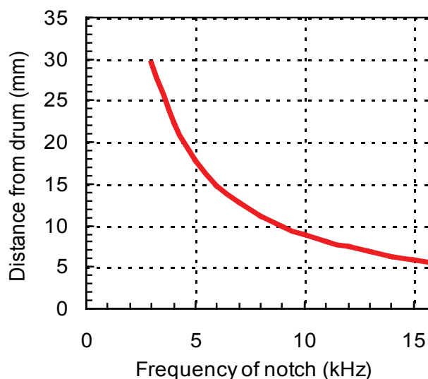
Figure 4.13 Distance from the eardrum at which SPL in the ear canal will be a minimum.
