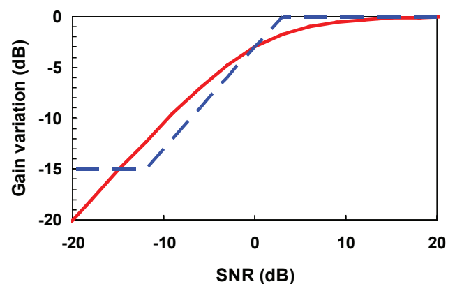
Figure 8.3 Attenuation provided by noise reduction systems for different SNRs. Solid line shows the Wiener Filter gain reduction of equation 8.2, and the dashed line shows the type of straight-line approximation used in many hearing aids.
