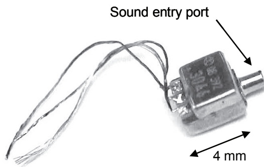
Figure 2.3 An electret microphone.
