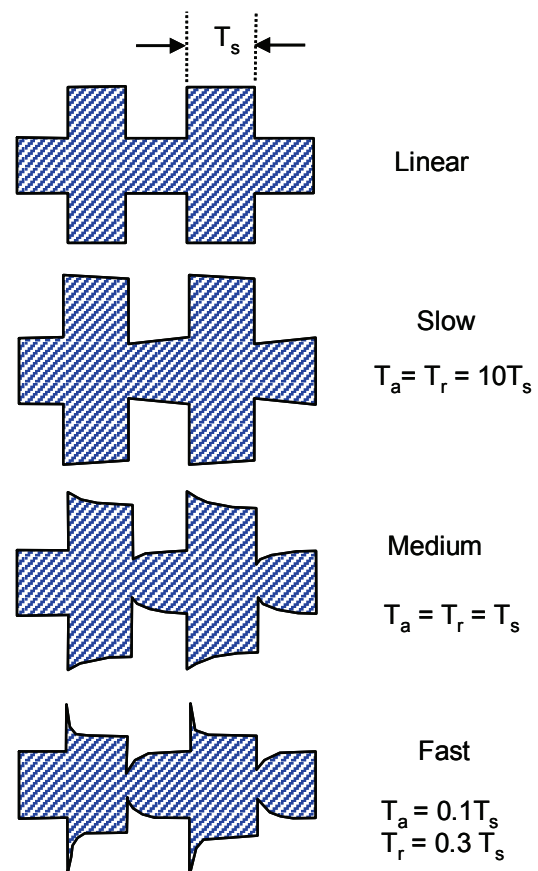
Figure 6.3 Envelopes for the output signal coming from a linear amplifier and compression amplifiers with different attack times ( T_a ), and release times ( T_r ) compared to the duration of each syllable ( T_s ) in the signal.
