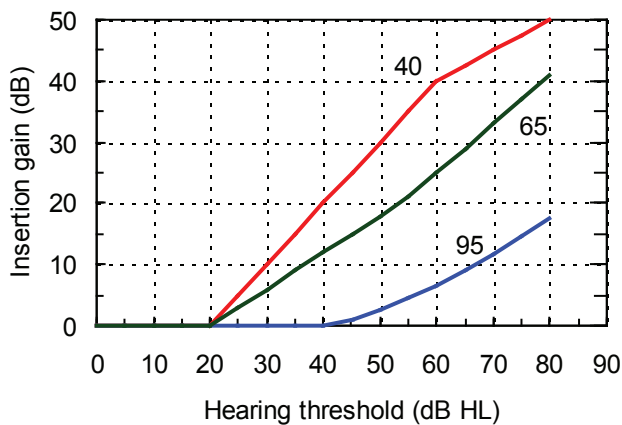
Figure 10.8 Insertion gain prescribed by the FIG6 method at any frequency as a function of hearing threshold, for each of the three input levels 40, 65, and 95 dB SPL.
