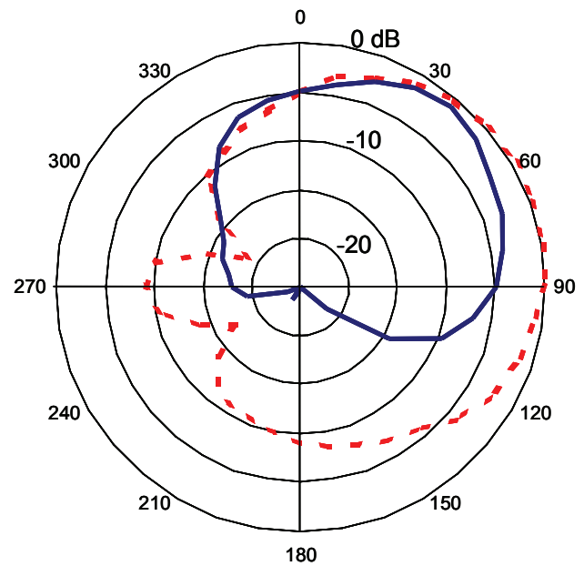
Figure 7.3 Polar directivity pattern, measured at 2 kHz, of an omni-directional microphone on the head (dashed line), and a cardioid directional microphone on the head (solid line), both in a BTE hearing aid. Data adapted from Knowles TB21. Each concentric circle represents a 5 dB change in sensitivity.
