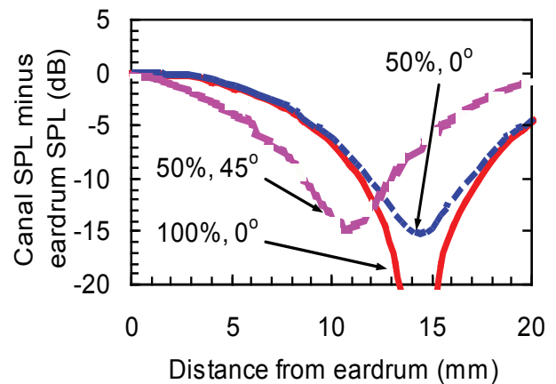
Figure 4.12 Calculated pattern of SPL in the ear canal versus distance from the eardrum at a frequency of 6 kHz. The red solid curve is for total reflection from the eardrum with no phase shift at the drum. As examples of the change in pattern caused by less than perfect reflection of sound, the blue dashed line is for 50% power reflected from the drum with no phase shift, and the pink speckled line is for 50% reflected with a 45 degree phase shift at the drum. There is significant inter-person variation in reflectance from the eardrum. 1865a
