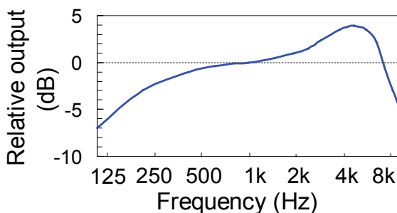
Figure 2.5 Frequency response of a typical electret microphone with tubing on its input port.
