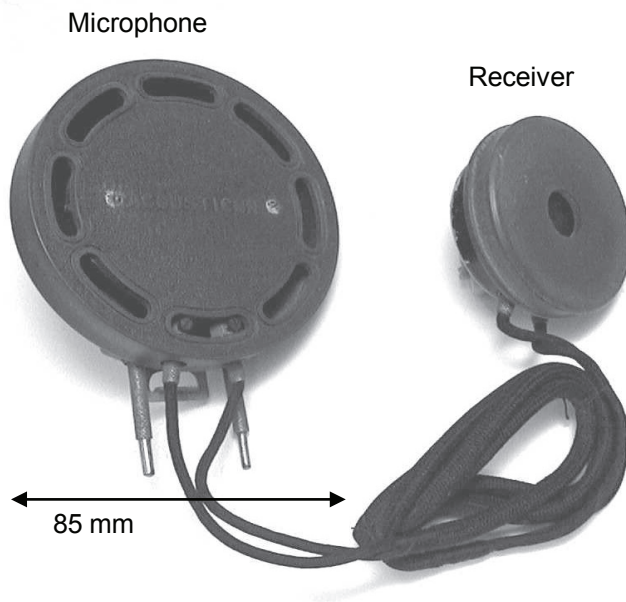
Figure 1.12 A carbon aid (The Acousticon) without its battery.
