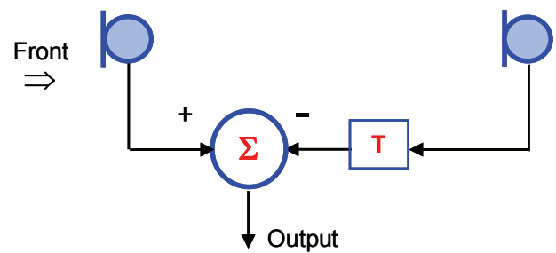
Figure 7.1 Block diagram of a subtractive directional microphone comprised of either a single microphone with two ports, or two separate microphones with one port each. The negative sign next to one of the inputs of the summer indicates that the two signals are subtracted.
