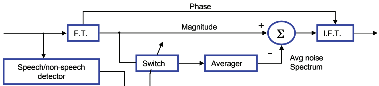
Figure 8.5 A Spectral Subtraction noise reduction system incorporating a Fourier Transform to calculate the power spectrum, a speech/non-speech detector to enable the average spectral power of the noise to be estimated, and an Inverse Fourier Transform to turn the corrected spectrum back into a waveform.
