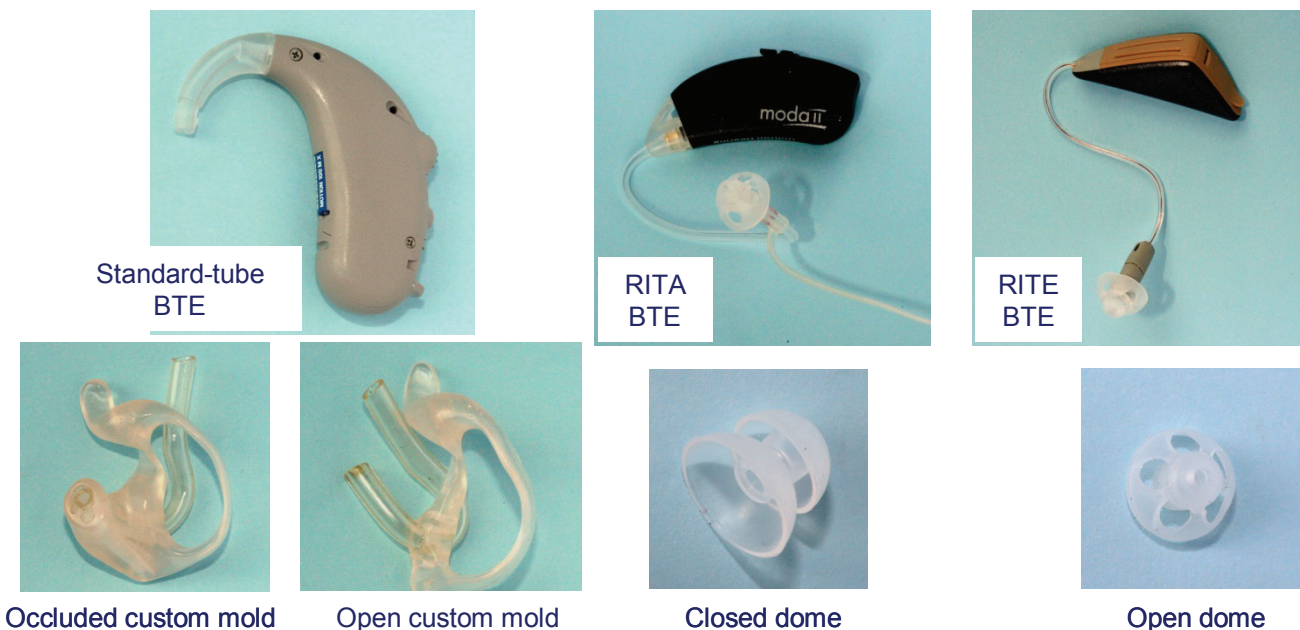
Figure 1.7 BTE hearing aids and ear fittings. The standard-tube BTE in the top left can be attached to an open or occluded custom mold. The RITA BTE and the RITE BTE can be attached to custom molds or to pre-formed canal fittings that can be either open or occluded.
