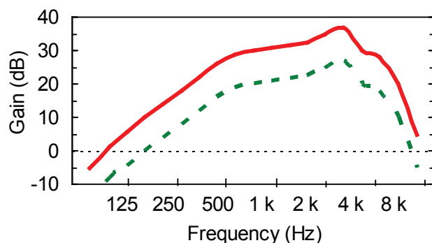
Figure 1.5 Gain-frequency response of an in-the-ear hearing aid at maximum volume control position (solid red line) and reduced volume control position (broken green line).
