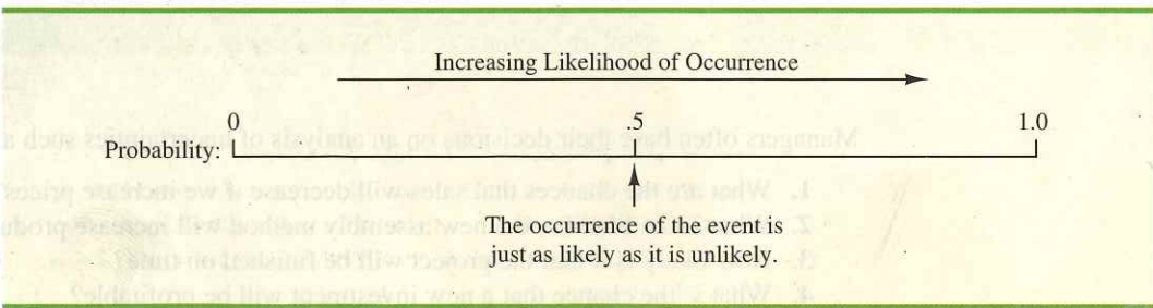
FIGURE 4.1 PROBABILITY AS A NUMERICAL MEASURE OF THE LIKELIHOOD OF AN EVENT OCCURRING
