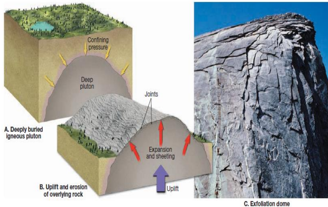
C. Exfoliation dome
