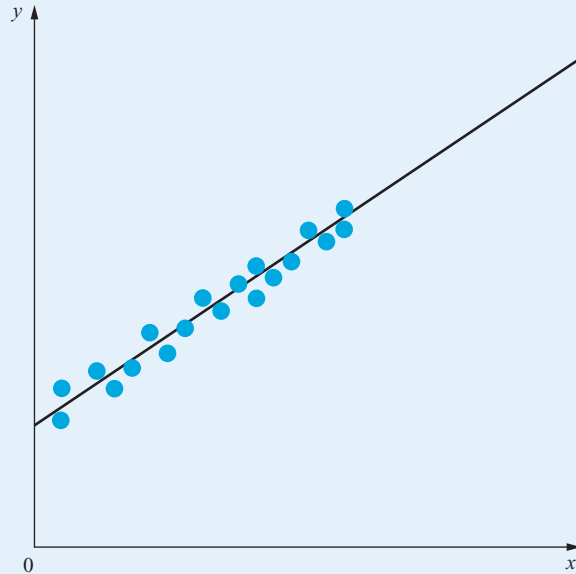
Figure 3.10 Effect on the standard errors of x_t^2 small
