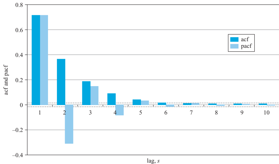
Figure 6.8 Sample autocorrelation and partial autocorrelation functions for an ARMA(1, 1) model: y_t = 0.5y_{t-1} + 0.5u_{t-1} + u_t
