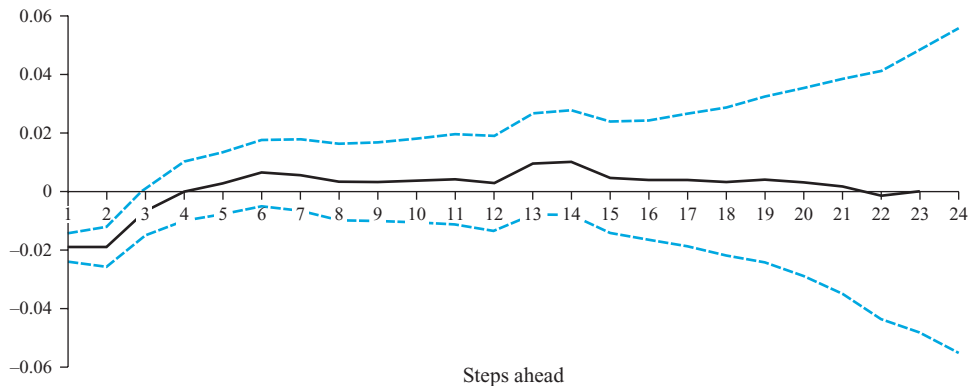
Figure 7.2 Impulse responses and standard error bands for innovations in the dividend yields
