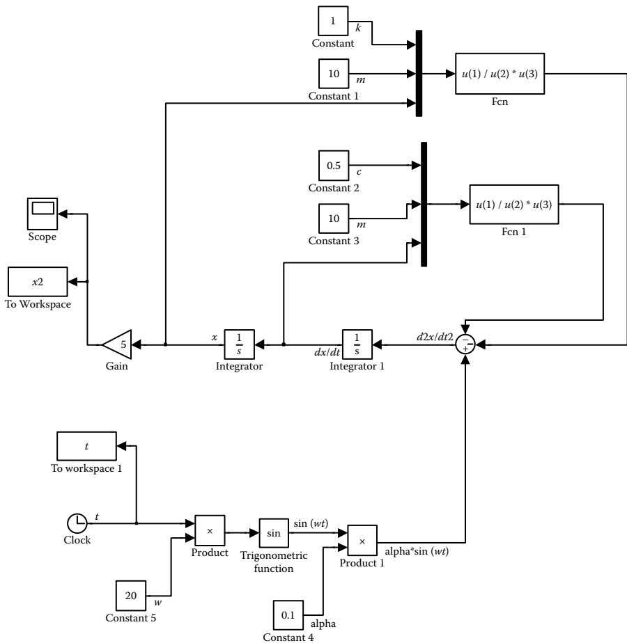
Figure 7.15 Block diagram for solving Equation (7.3).
