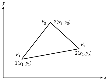
Figure 13.2 Linear triangular scalar field element.
