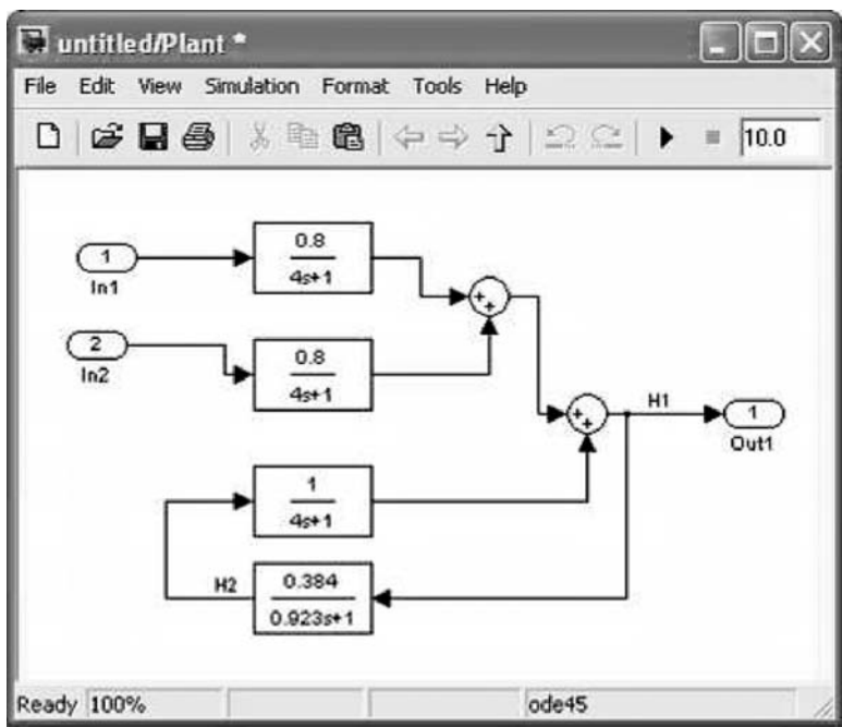
Figure 14.37 Simulink description of the plant. (From MATLAB. With permission.)
