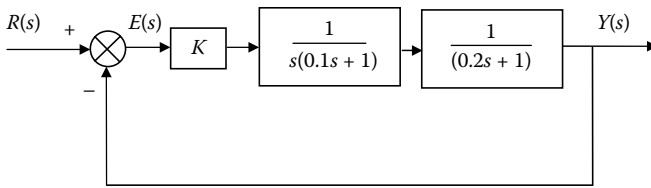
Figure P14.1 Block diagram for Project 14.1.
