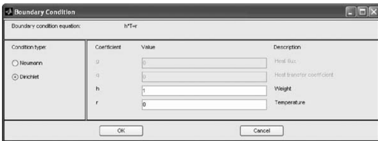
Figure 13.61 Input r = 0 to specify the temperature of 50^\circ\text{C} along this edge. (From MATLAB. With permission.)
