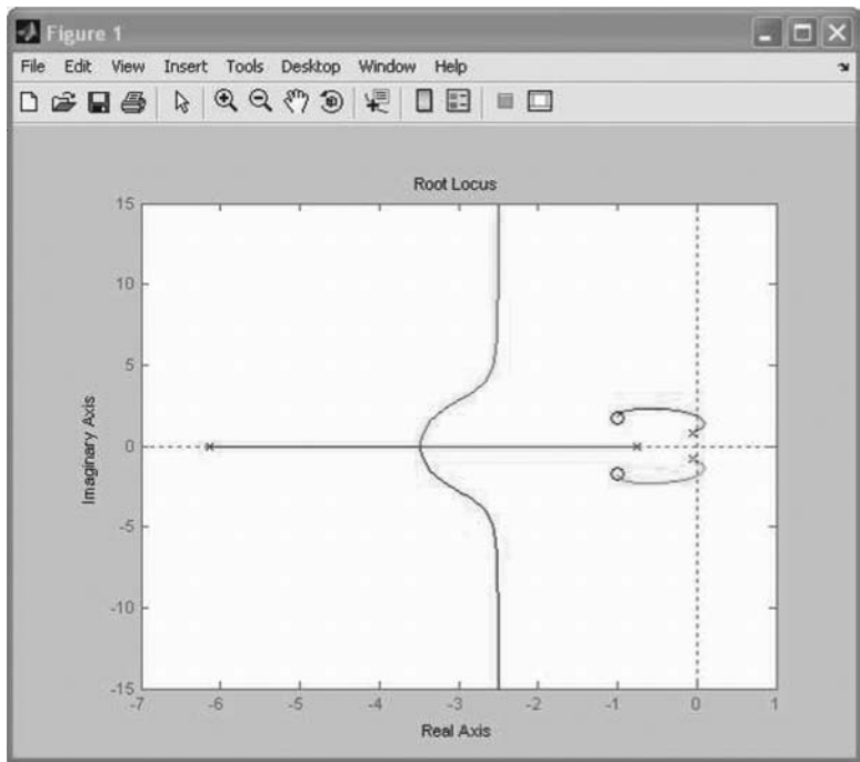
Figure 14.16 Root locus plot of the above closed-loop transfer function. (From MATLAB. With permission.) (See color insert following page 334.)
