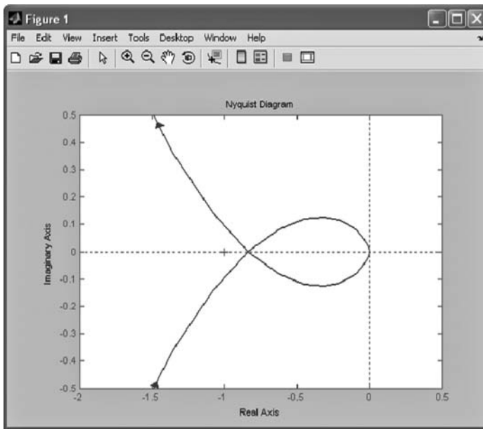
Figure 14.19 Modified Nyquist plot of L(s) . (From MATLAB. With permission.)
