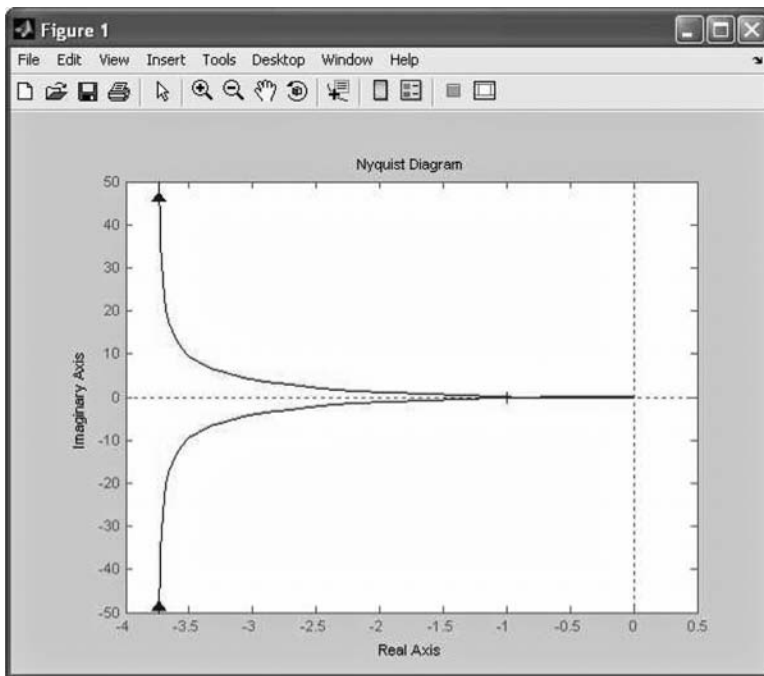
Figure 14.18 Nyquist plot of L(s) defined by Equation (14.36). (From MATLAB. With permission.)
