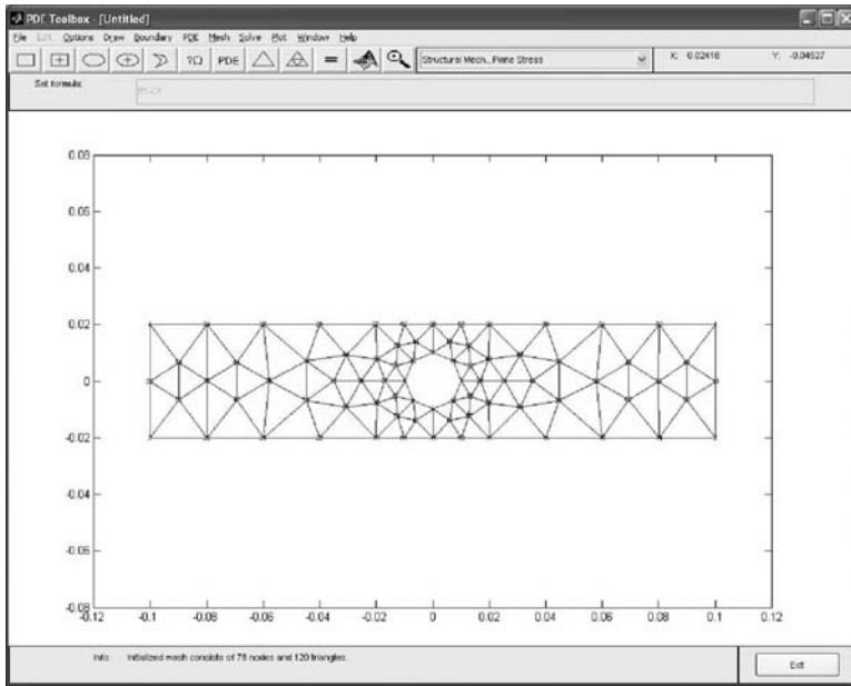
Figure 13.28 Initial mesh with node number. (From MATLAB. With permission.)
