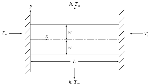
Figure 13.57 Geometry and boundary condition for Example 13.4.
