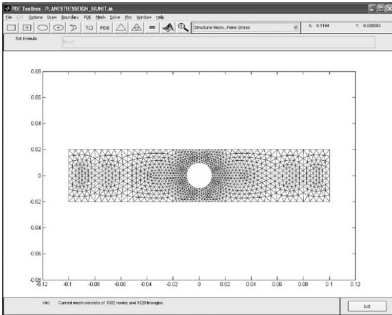
Figure 13.40 Refined mesh. (From MATLAB. With permission.)
