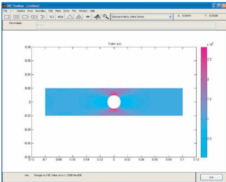
Figure 13.36 Contour plot of normal stress \sigma_{xx} . (From MATLAB. With permission.)
