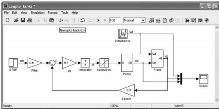
Figure 14.44 Simulation block diagram of the modified model with disturbance. (From MATLAB. With permission.)
