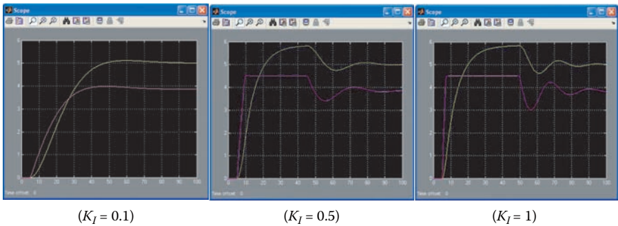
Figure 14.43 Simulation results of the modified model. (From MATLAB. With permission.)
