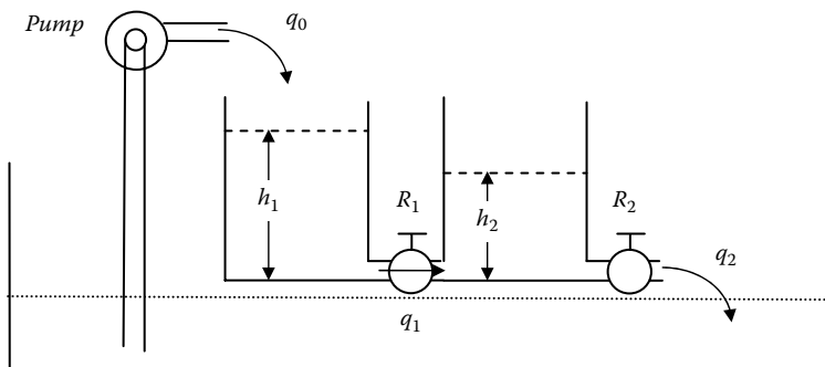
Figure 14.5 Coupled tanks.
