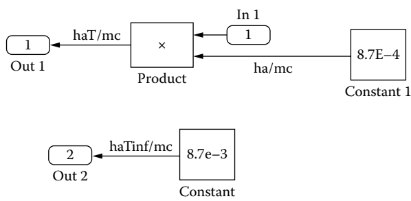
Figure 7.10 Sketch of subsystem.
