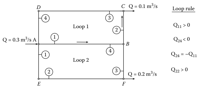
Figure 11.2 Loop rule for pipe network.
