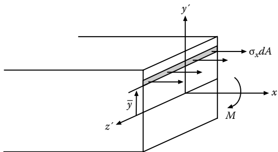
Figure A.1b Stress at beam section.
