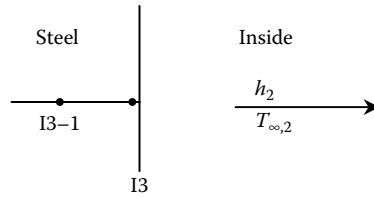
Figure P10.7e Steel-inside air interface.
