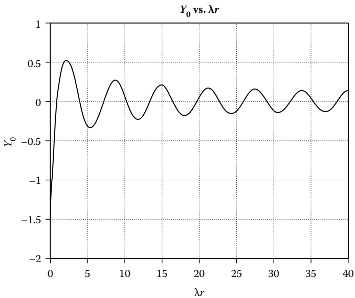
Figure 10.6 The plot of Y_0 vs. \lambda r .
