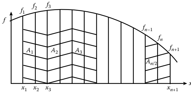
Figure 5.2 Integration areas.
