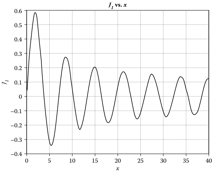
Figure P4.8b Plot of J_1(x) function.
