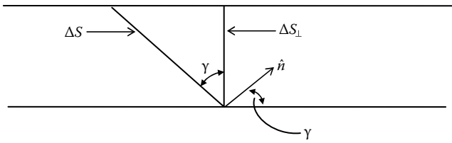
Figure B.1c Relation between \Delta S and \Delta S_{\perp} .
