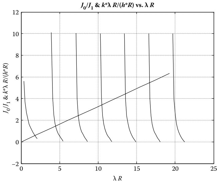
Figure 10.8 The plot of J_0/J_1 and \lambda Rk/hR vs. \lambda R .
