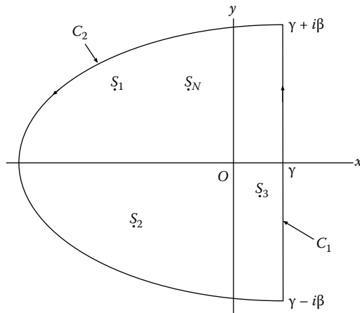
Figure 12.9 Region enclosing several poles.
