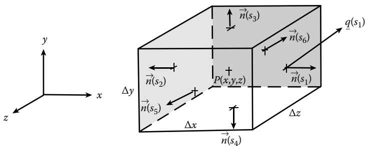
Figure B.2a Infinitesimal volume in Cartesian coordinates.
