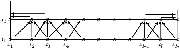
Figure 10.11 The order of calculations and marching in time.
