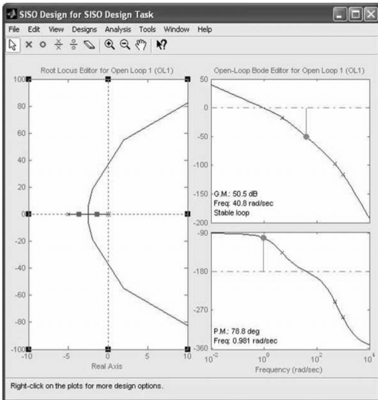
Figure 14.33 Root locus of the system. (From MATLAB. With permission.)
