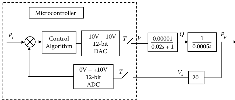
Figure 14.64 Block diagram of a position sampled data control system.
