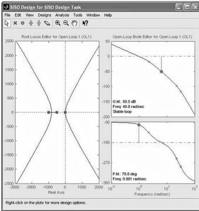
Figure 14.28 Plots initially displayed by SISOTool for the example. (From MATLAB. With permission.)
