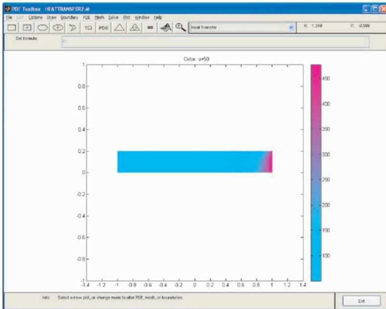
Figure 13.67 Contour plot of the temperature field after adding 50°C to the solutions shown in Figure 13.65. (From MATLAB. With permission.)
