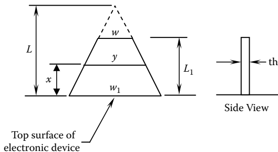
Figure P6.8 Fin attached to an electronic device.
