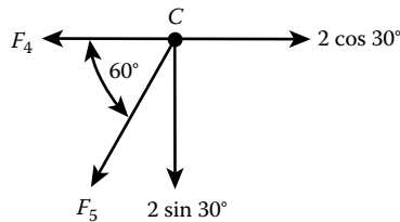
Figure 3.5 Internal forces at Joint C.
