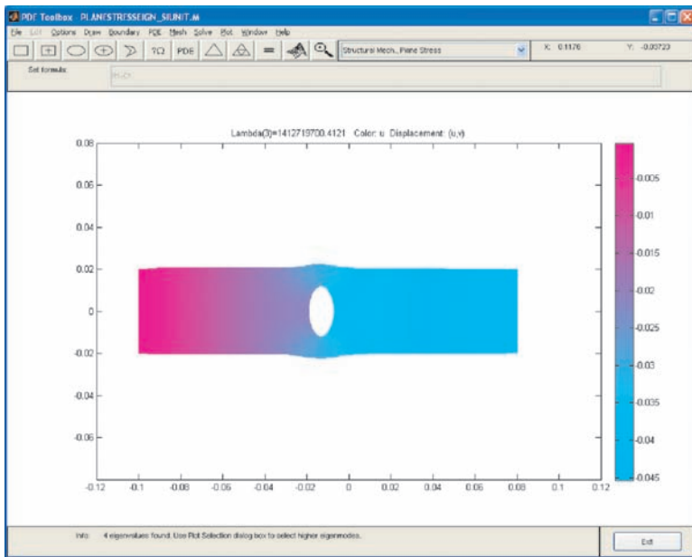
Figure 13.44 The third vibration mode for the third lowest natural frequency. (From MATLAB. With permission.)
