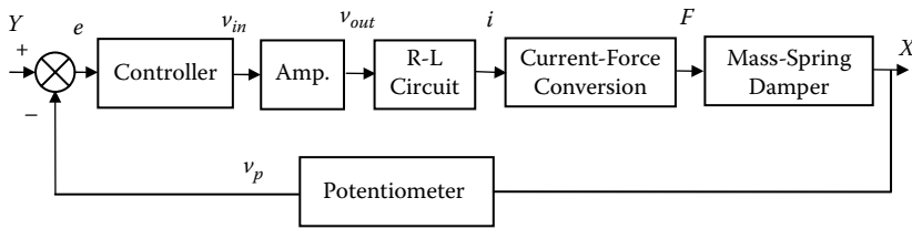
Figure 14.23 Schematic block diagram of the system shown in Figure 14.22.
