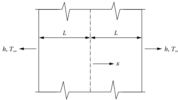
Figure 10.3 A thick bar suddenly immersed in a liquid.
