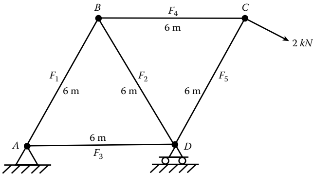
Figure 3.1 Simple truss.
