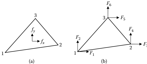
Figure 13.7 (a) Body forces acting on an element. (b) Equivalent nodal force at each node due to the body forces.
