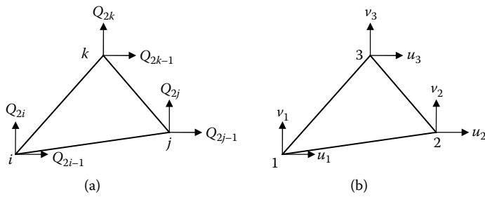
Figure 13.6 (a) Global displacement components for an element with node numbers i, j , and k . (b) Corresponding displacement components in a local element, where local node numbers 1, 2, and 3 are corresponding to global node numbers i, j , and k , respectively.
