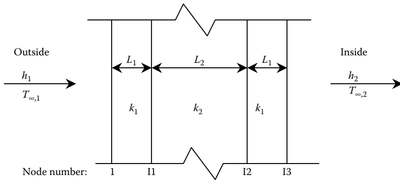
Figure P10.7a Wall geometry.
