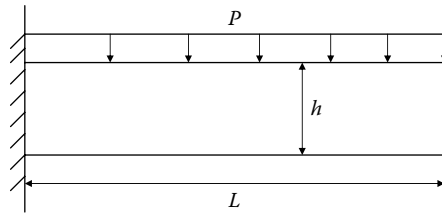
Figure P13.1 Geometry of a cantilevered beam for Project 13.1.
