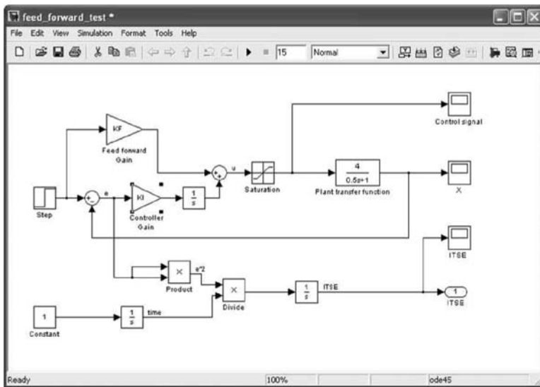
Figure 14.48 Simulink program for the system in Figure 14.47 with ITSE. (From MATLAB. With permission.)
