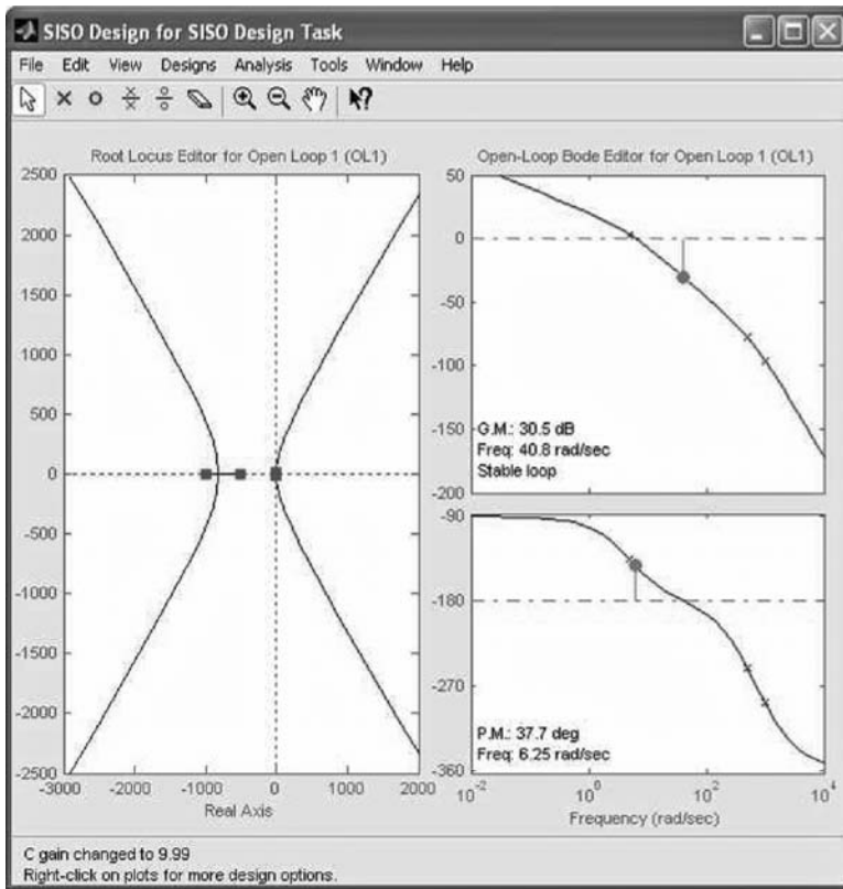
Figure 14.31 Bode diagram of the system after modification of the GM . (From MATLAB. With permission.)
