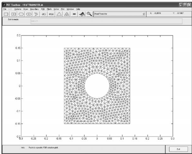
Figure 13.52 Refined mesh. (From MATLAB. With permission.)
