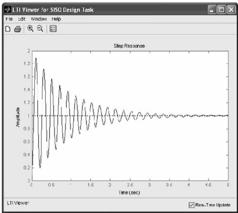
Figure 14.34 Response of the system in Figure 14.33 to a unit step. (From MATLAB. With permission.)
