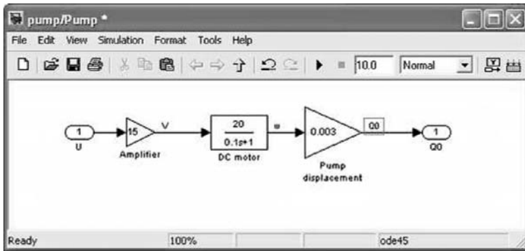
Figure 14.39 Simulink description of the pump unit. (From MATLAB. With permission.)
