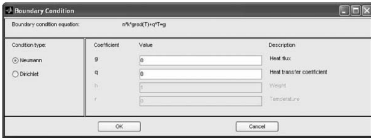
Figure 13.49 Boundary condition window for input of the Neumann boundary condition to specify the insulated edges. (From MATLAB. With permission.)
