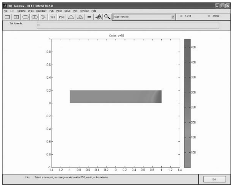
Figure 13.67 Contour plot of the temperature field after adding 50°C to the solutions shown in Figure 13.65. (From MATLAB. With permission.) (See color insert.)
