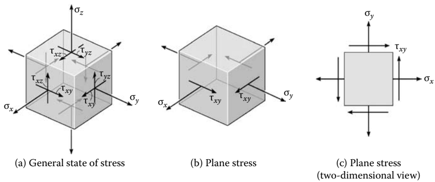
Figure 13.1 Illustration of stress at a point in a body.
