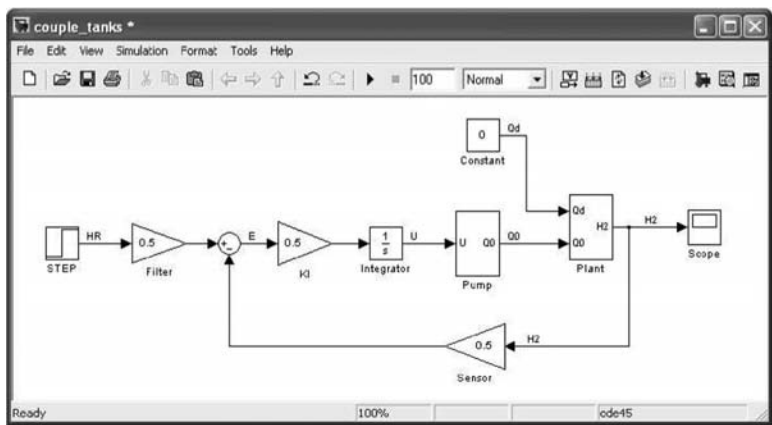
Figure 14.40 Complete Simulink block diagram. (From MATLAB. With permission.)
