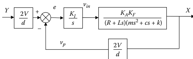
Figure 14.25 Modified block diagram of the system shown in Figure 14.22.
