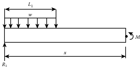
Figure 6.4 Sketch indicating internal moment at section x , where L_1 < x \leq L_2 .
