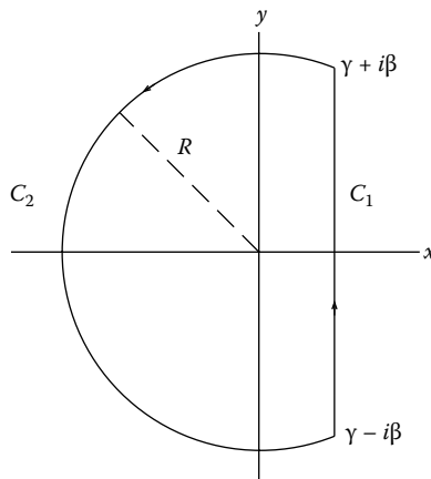
Figure 12.8 Region in the complex plane for determining f(t) .
