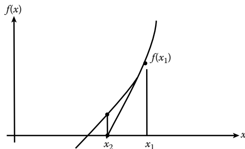
Figure 4.3 Predicting root in the Newton–Raphson Method.
