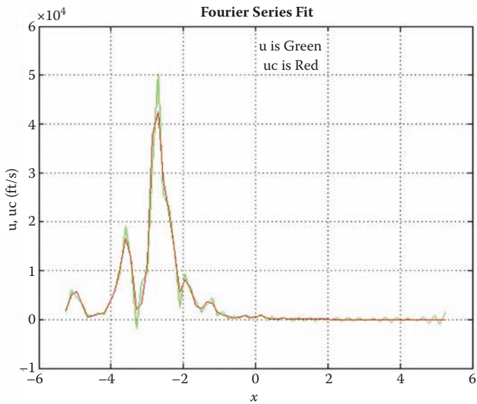
Figure 8.4 Fourier series fit of the data.
