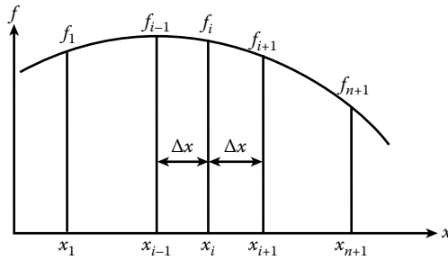
Figure 5.1 Arbitrary three points on the curve f(x) .
