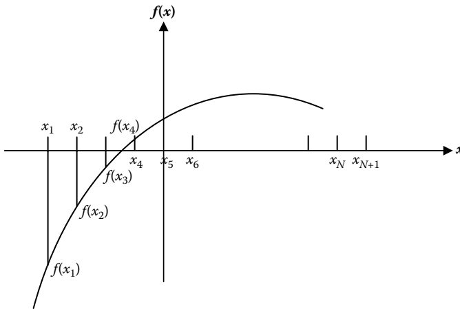
Figure 4.1 Selecting the interval in which a root lies.
