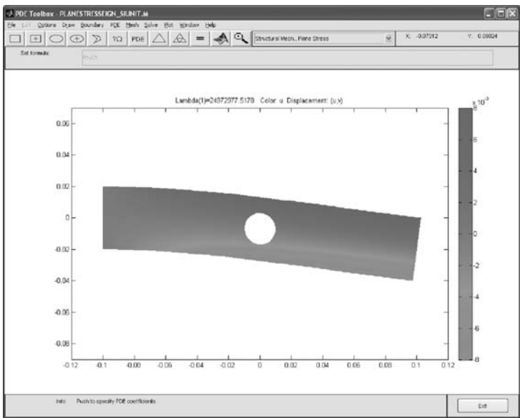
Figure 13.42 The first vibration mode for the lowest natural frequency. (From MATLAB. With permission.) (See color insert.)
