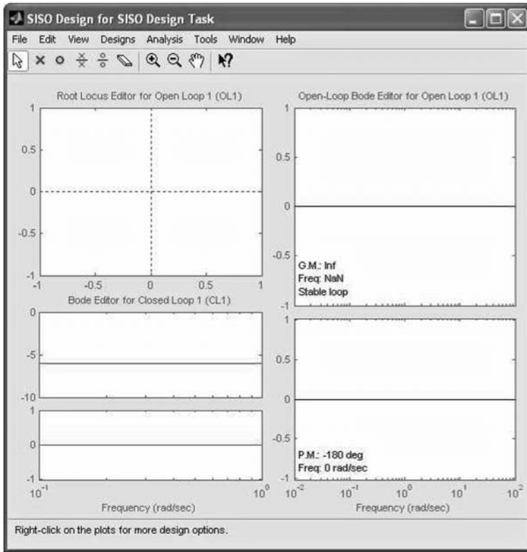
Figure 14.27 Plots initially displayed by SISOTool . (From MATLAB. With permission.)
