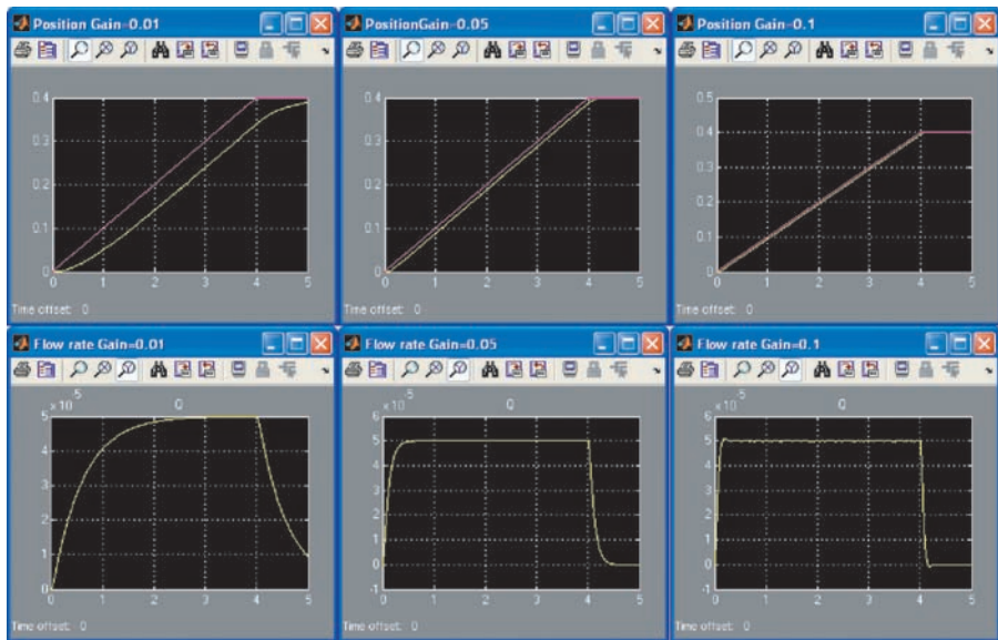
Figure 14.69 Simulation results for different controller gains ( T = 0.01 second): (a) gain = 0.01; (b) gain = 0.05; (c) gain = 0.1. (From MATLAB. With permission.)
