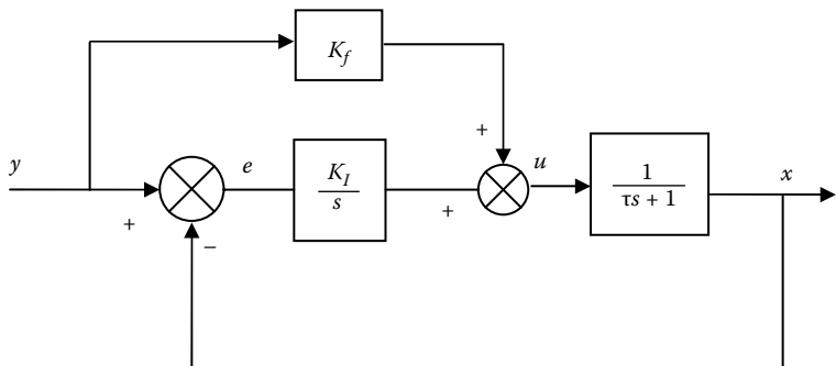
Figure 14.47 A control system with a feed-forward loop.
