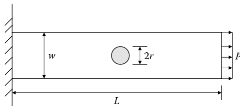
Figure 13.15 Geometry of a plate with a hole at the center. (From MATLAB. With permission.)
