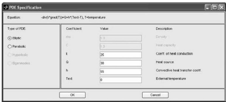
Figure 13.51 PDF specification for input of the physical constants. (From MATLAB. With permission.)
