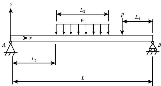
Figure P6.9b Determinate beam structure.
