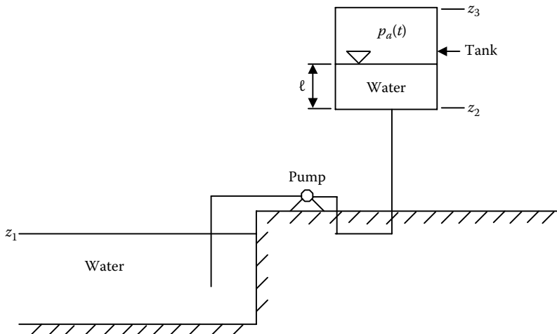
Figure P11.4 A sketch of a reservoir, pump, tank system. (From Reference [5]. With permission of Manchester University Press.)
