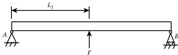
Figure P6.9c Beam with single concentrated load.
