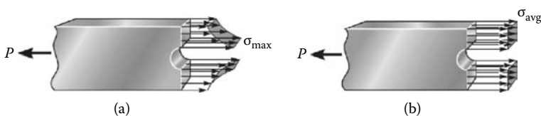
Figure 13.37 (a) Normal stress distribution from FEA solution. (b) Average normal stress obtained from strength of materials. (From MATLAB. With permission.)
