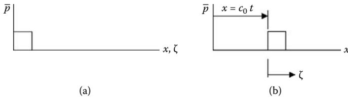
Figure 10.10 Example of a small step pressure disturbance, (a) t = 0 , (b) t > 0 .
