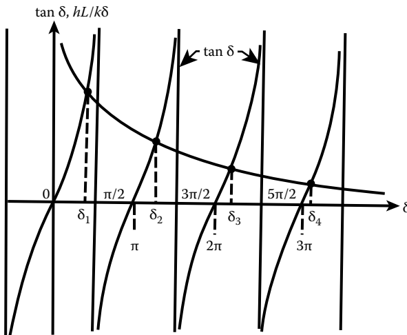
Figure 10.4 The plot of \tan \delta and \frac{hL}{k\delta} vs. \delta .
