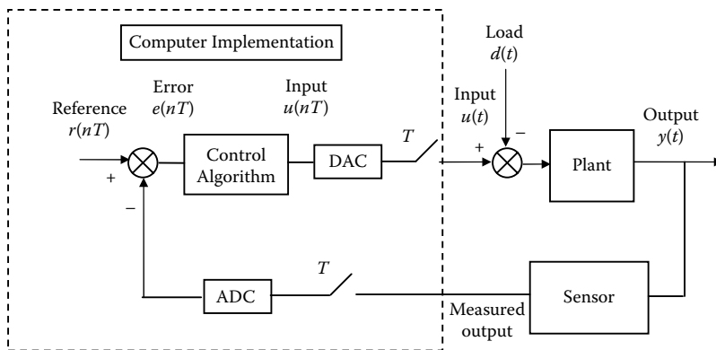
Figure 14.58 Block diagram of a sampled data control system.
