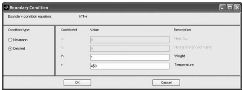
Figure 13.62 Input r = 450 to specify the temperature of 500^{\circ}\text{C} along this edge. (From MATLAB. With permission.)
