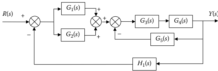
Figure P14.3 Block diagram for Project 14.3.
