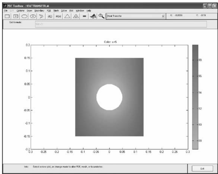
Figure 13.55 Contour plot of the temperature field after adding 5°C to the solutions shown in Figure 13.53. (From MATLAB. With permission.)
