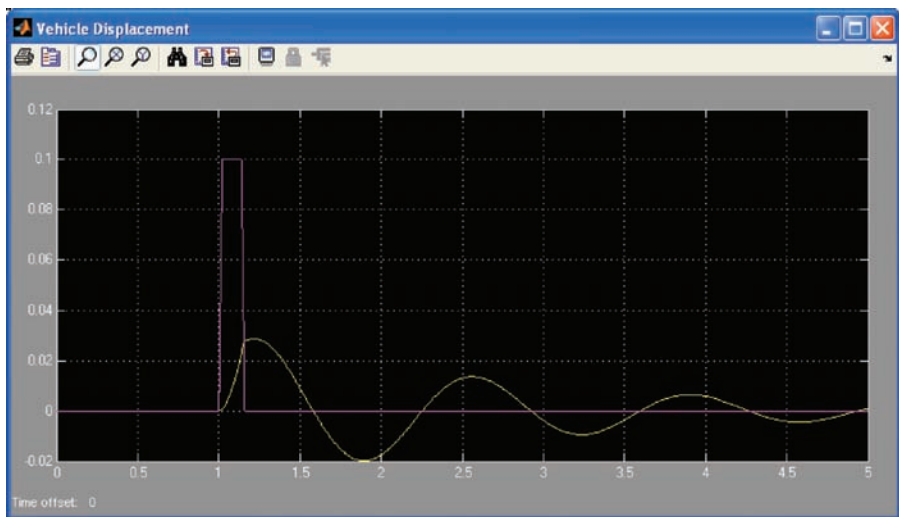
Figure 14.56 Vehicle's displacement. (From MATLAB. With permission.)
