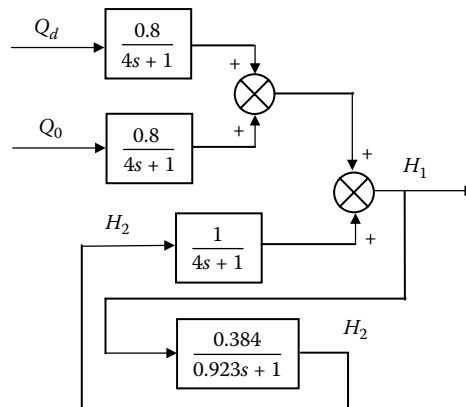
Figure 14.36 Plant's block diagram.
