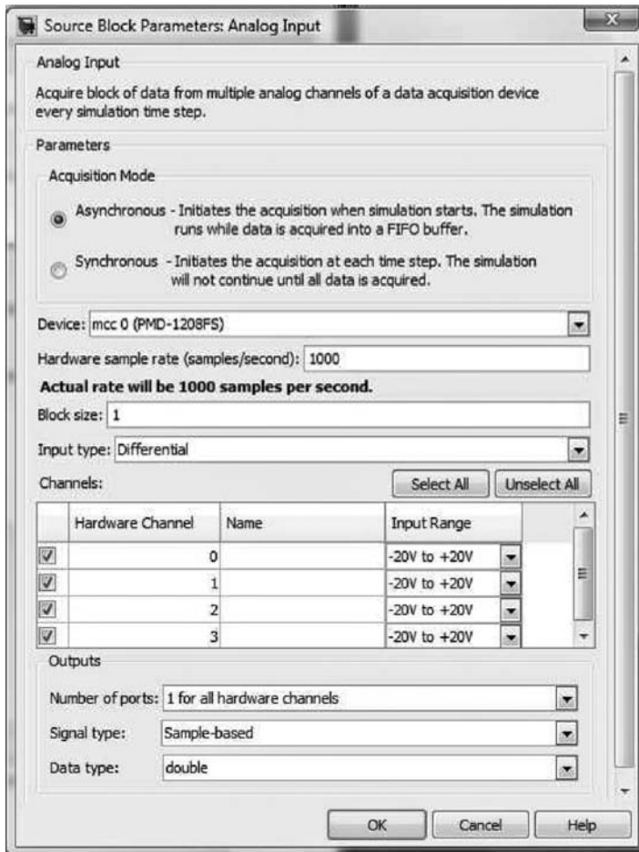
Figure 14.71 Analog Input block parameters. (From MATLAB. With permission.)
