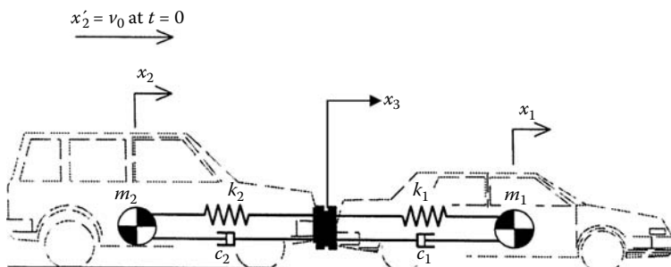
Figure P6.7 Linear three-degree-of-freedom model for low-speed car collision. (SAE Paper 980360. Copyright 1998 SAE International. With permission.)
