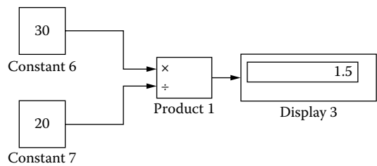
Figure 7.5 Constants, product, and display blocks for division.
