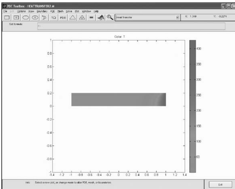
Figure 13.65 Contour plot of the temperature field. (From MATLAB. With permission.) (See color insert.)
