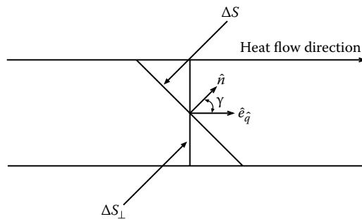
Figure B.1b Heat flow through an arbitrary oriented surface.
