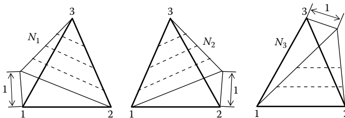
Figure 13.3 Illustration of three shape functions.
