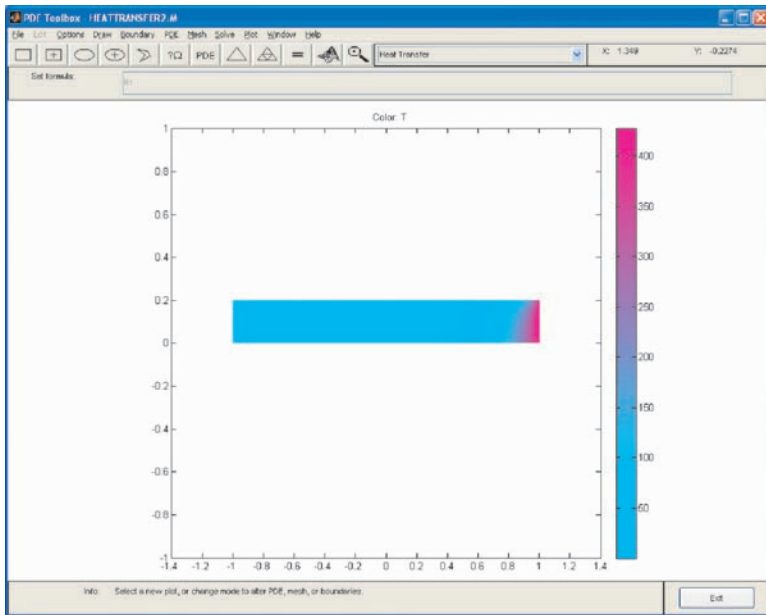
Figure 13.65 Contour plot of the temperature field. (From MATLAB. With permission.)
