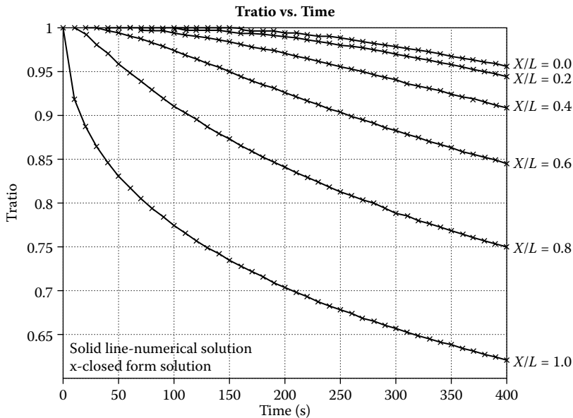
Figure P10.4 The plot of TRATIO vs. time. Numerical solution is by the explicit method.
