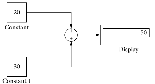
Figure 7.2 Constants, summation, and display blocks for addition.
