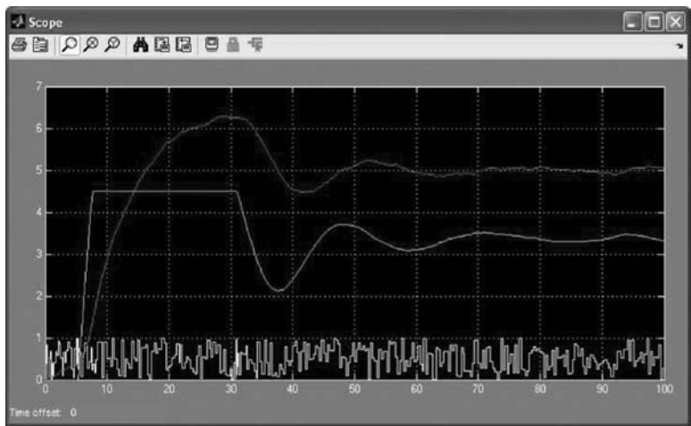
Figure 14.46 Simulation results of the modified model with disturbance ( K_I = 1.0 ). (From MATLAB. With permission.) (See color insert.)
