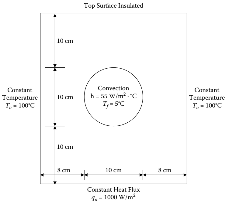
Figure 13.45 Geometry and boundary condition for Example 13.3. (From MATLAB. With permission.)
