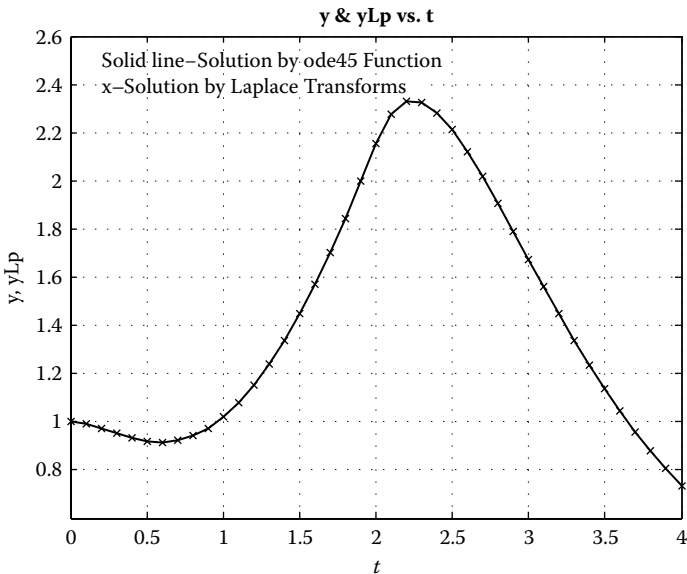
Figure 12.4 A comparison between a solution obtained by Laplace Transforms and ode45.
