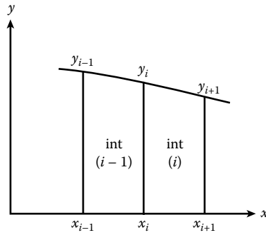
Figure 8.2 Two adjacent arbitrary intervals.
