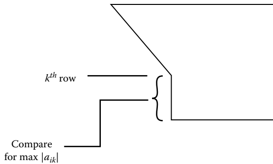
Figure 3.7 Row interchange.
