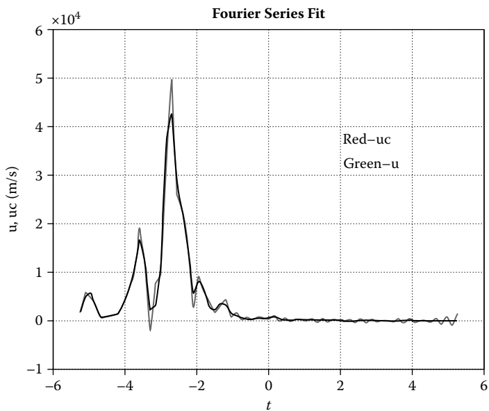
Figure 8.4 Fourier series fit of the data. (See color insert following page 334.)
