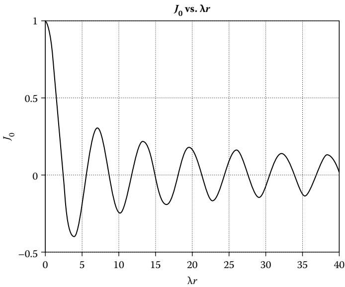
Figure 10.5 The plot of J_0 vs. \lambda r .
