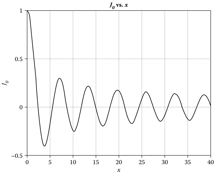
Figure P4.8a Plot of J_0(x) function.
