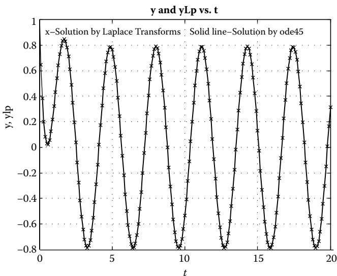
Figure 12.2 A comparison between a solution obtained by Laplace Transforms and ode45.
