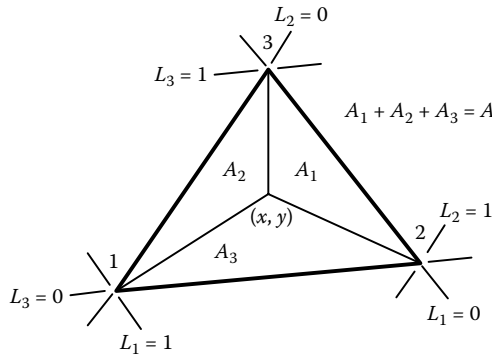
Figure 13.5 Area coordinates in a triangular element.
