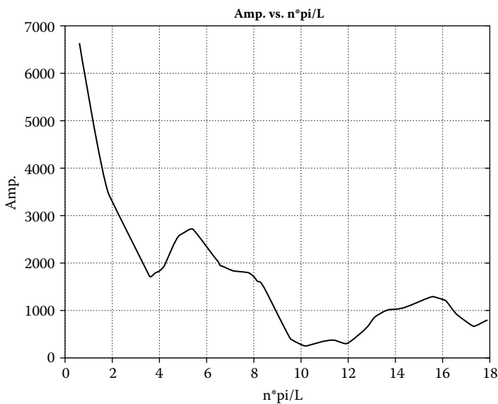
Figure 8.5 Fourier series coefficient amplitudes vs. \frac{n\pi}{L} .
