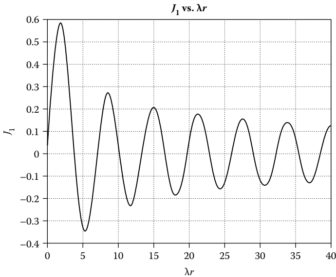
Figure 10.7 The plot of J_1 vs. \lambda r .
