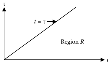
Figure 12.5 Integration in the (\tau, t) plane.
