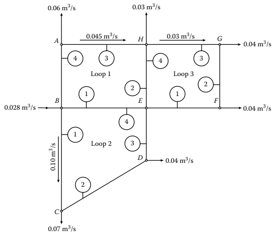
Figure P11.3 A pipe network.
