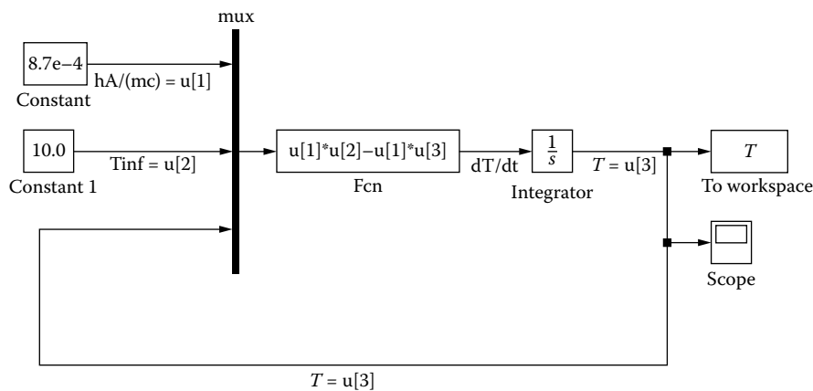
Figure 7.11 Block diagram for solving Equation (7.2) using the mux and fcn blocks.
