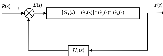
Figure 14.11 Simplified block diagram of the system shown in Figure 14.8.
