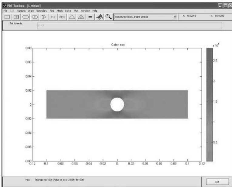
Figure 13.36 Contour plot of normal stress \sigma_x . (From MATLAB. With permission.) (See color insert.)
