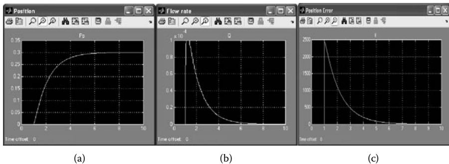
Figure 14.66 Simulation results (for a controller gain of 0.005 and T = 0.01 second): (a) piston position; (b) flow rate through the valve; (c) position error. (From MATLAB. With permission.)
