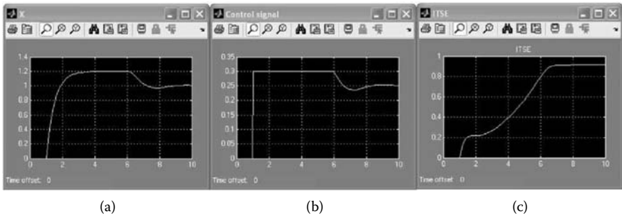
Figure 14.49 Simulation results: (a) X ; (b) u ; (c) ITSE. (From MATLAB. With permission.)
