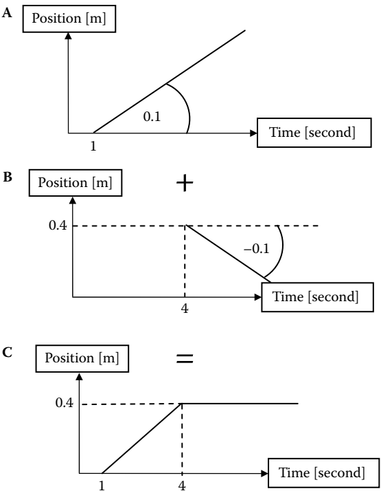
Figure 14.68 Reference generation for speed of 0.1 m/s and final position of 0.4 m.
