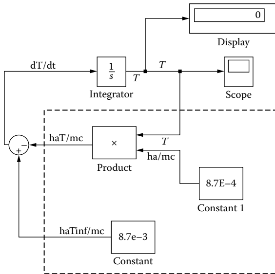
Figure 7.8 Constructing a subsystem.
