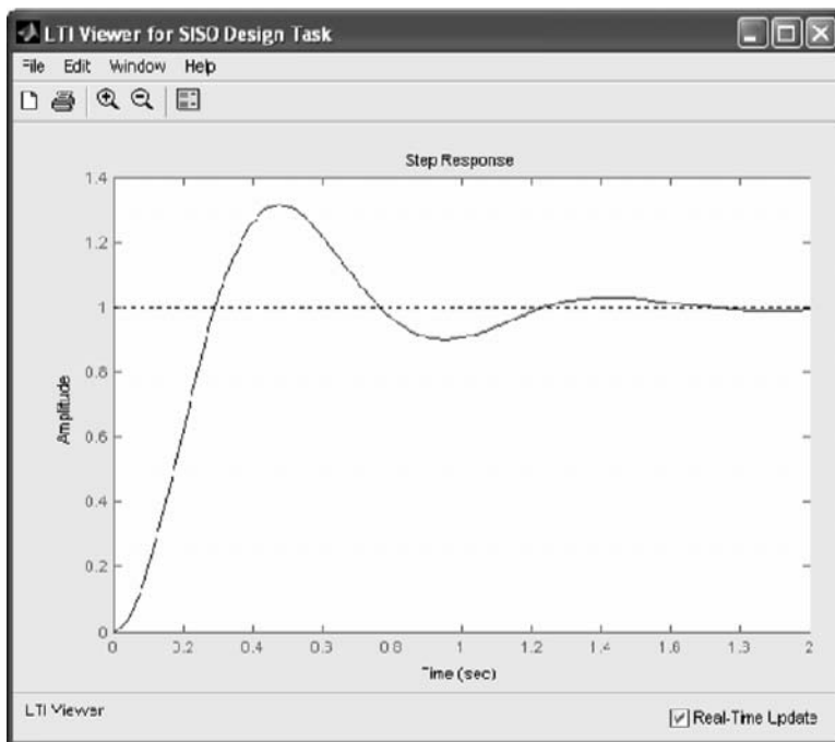
Figure 14.32 Time response to a unit step of the closed-loop system after modification of the GM . (From MATLAB. With permission.)
