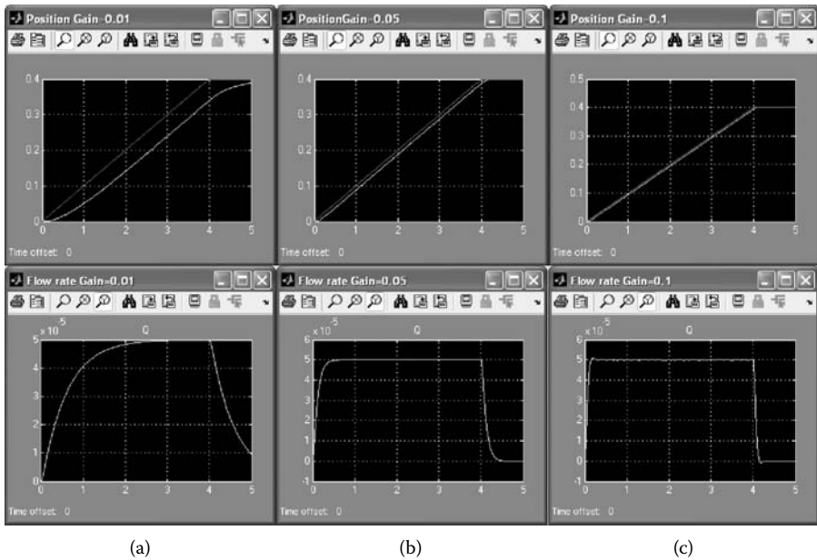
Figure 14.69 Simulation results for different controller gains ( T = 0.01 second): (a) gain = 0.01; (b) gain = 0.05; (c) gain = 0.1. (From MATLAB. With permission.) (See color insert.)
