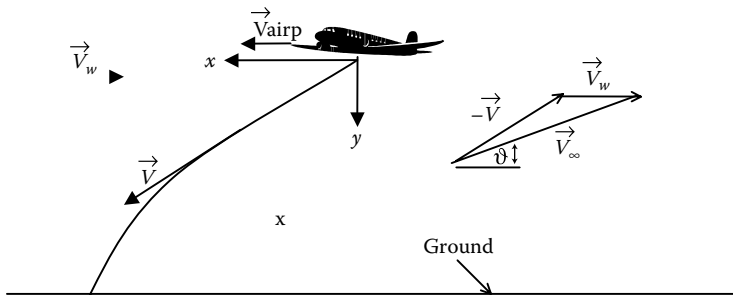
Figure P6.1 Airplane dropping food package.
