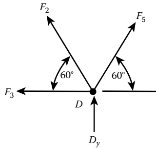
Figure 3.6 Internal forces at Joint D.
