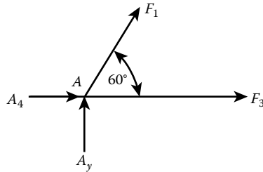
Figure 3.2 Reactions of simple truss.
