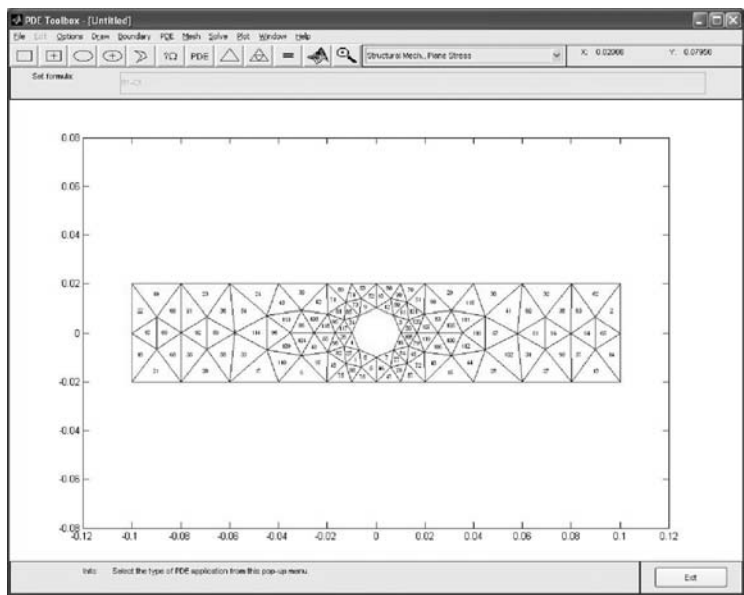
Figure 13.29 Initial mesh with element number. (From MATLAB. With permission.)
