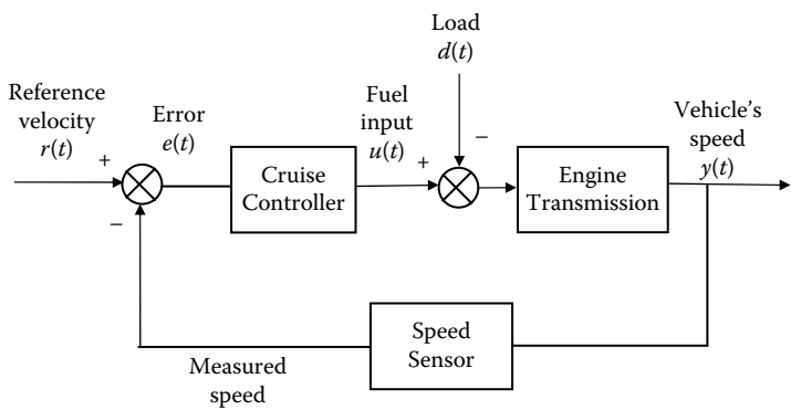
Figure 14.2 Cruise control block diagram.
