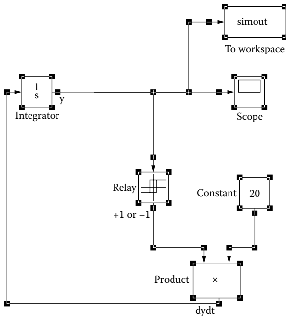
Figure 7.12 Block diagram using the relay block.
