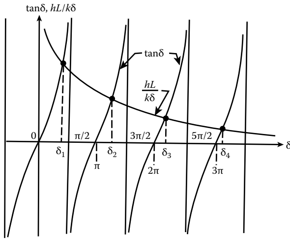
Figure P4.1b Intersection of hL/k\delta and \tan \delta curves.
