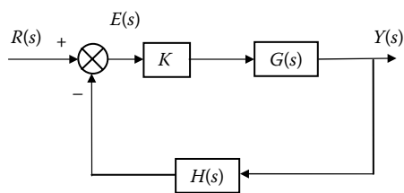
Figure 14.14 A simple closed-loop system.
