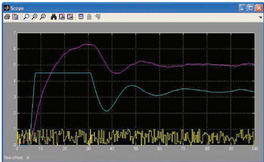
Figure 14.46 Simulation results of the modified model with disturbance ( K_t = 1.0 ). (From MATLAB. With permission.)
