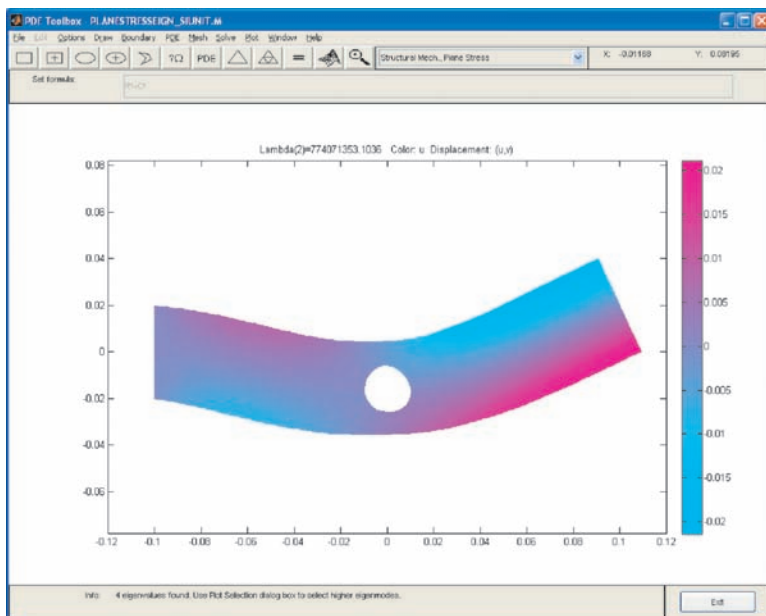
Figure 13.43 The second vibration mode for the second lowest natural frequency. (From MATLAB. With permission.)
