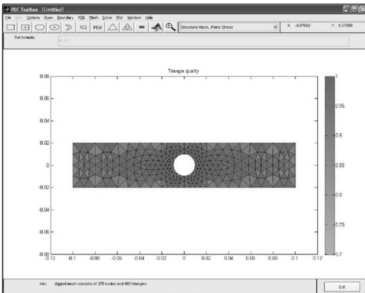
Figure 13.32 Contour plot to display the quality of the triangular element. (From MATLAB. With permission.)
