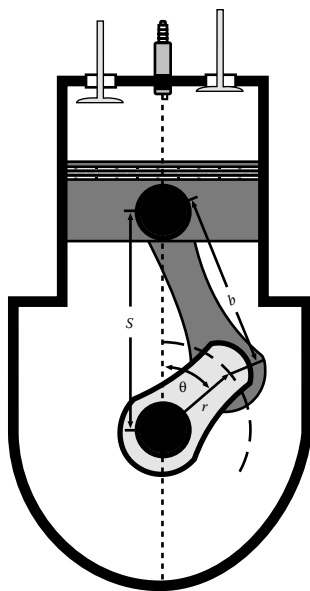
Figure P2.12b Geometry of piston motion.
