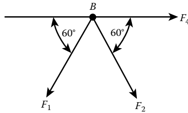
Figure 3.4 Internal forces at Joint B.
