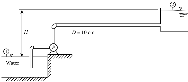
Figure 11.1 A piping system.
