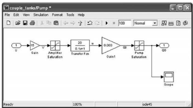
Figure 14.42 Changes in the pump unit block diagram. (From MATLAB. With permission.)
