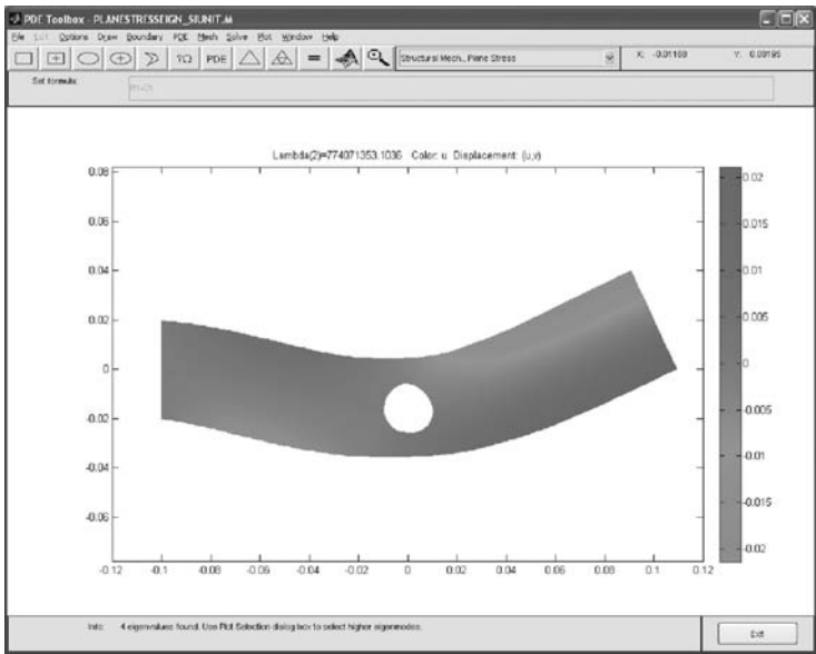
Figure 13.43 The second vibration mode for the second lowest natural frequency. (From MATLAB. With permission.) (See color insert.)
