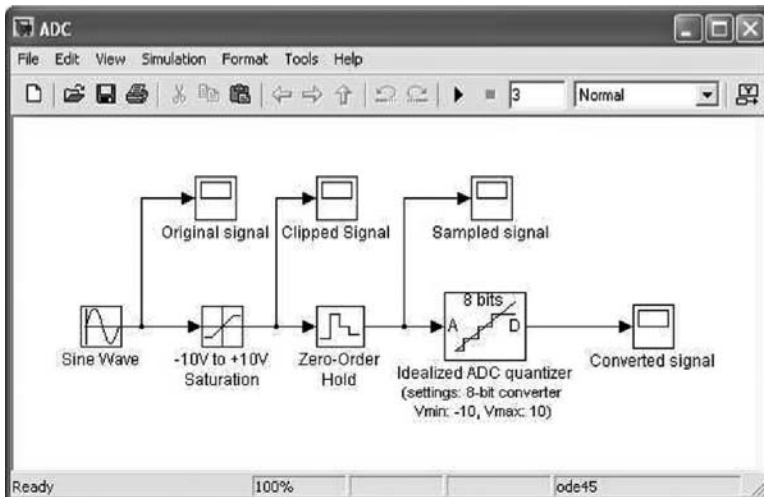
Figure 14.59 Analog-to-digital converter implementation. (From MATLAB. With permission.)
