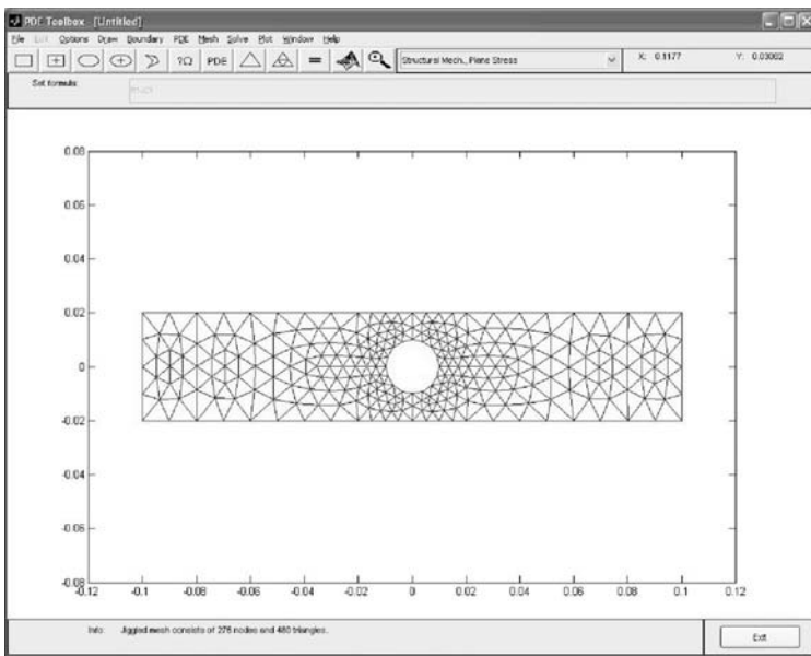
Figure 13.31 Refined mesh. (From MATLAB. With permission.)
