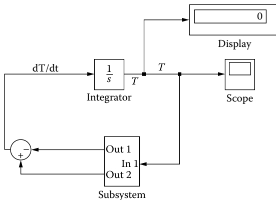
Figure 7.9 Block diagram for solving Equation (7.2).
