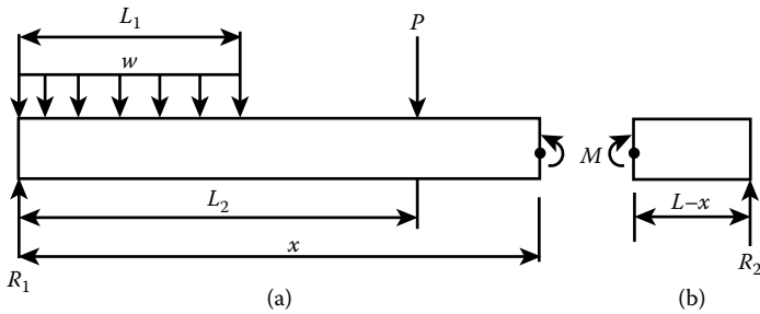
Figure 6.5 Sketch indicating internal moment at section x , where, L_2 < x \leq L , (a) as seen from the left side and (b) as seen from the right side.
