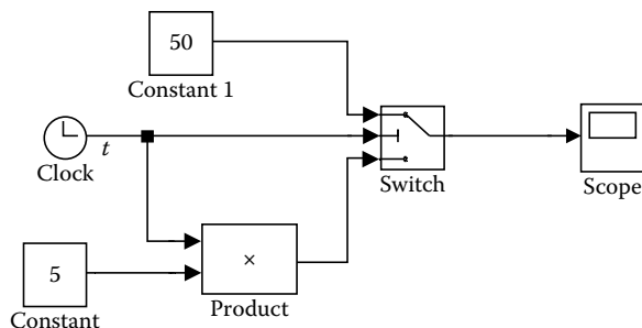
Figure 7.13 Block diagram using the switch block.
