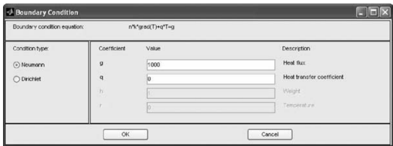
Figure 13.48 Boundary condition window for input of the Neumann boundary condition to specify the heat flux = 1000\text{ W/m}^2 . (From MATLAB. With permission.)
