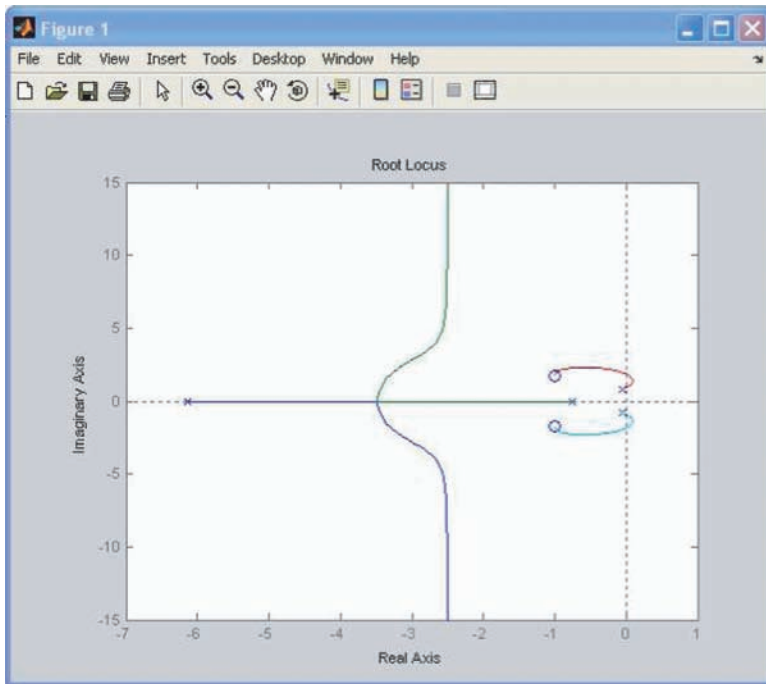
Figure 14.16 Root locus plot of the above closed-loop transfer function. (From MATLAB. With permission.)
