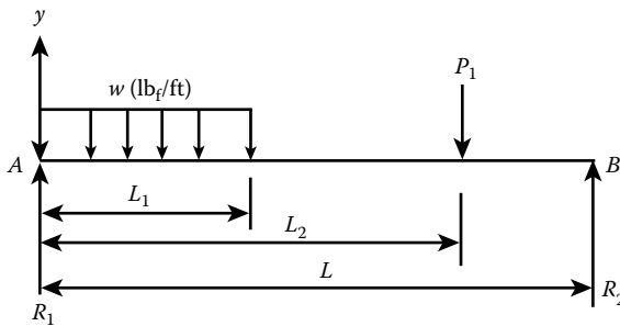
Figure 6.2 Beam loading.
