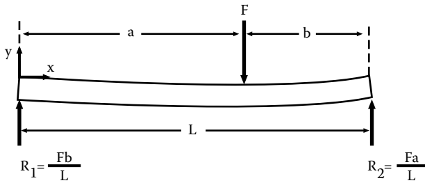
Figure P6.9d Beam loaded with a single concentrated load.
