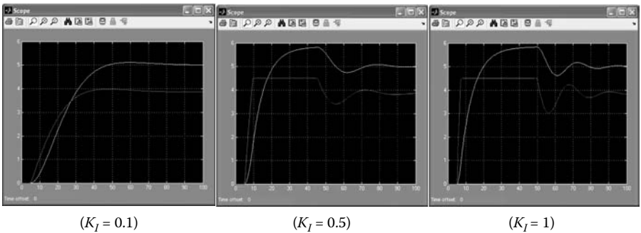
Figure 14.43 Simulation results of the modified model. (From MATLAB. With permission.) (See color insert.)
