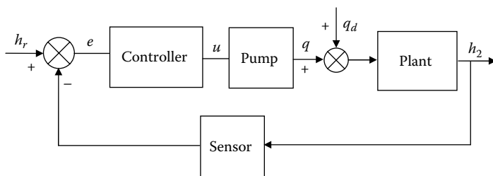
Figure 14.35 Proposed block diagram for the fluid level control system.
