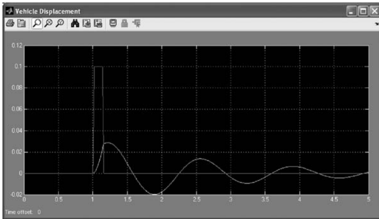
Figure 14.56 Vehicle's displacement. (From MATLAB. With permission.) (See color insert.)
