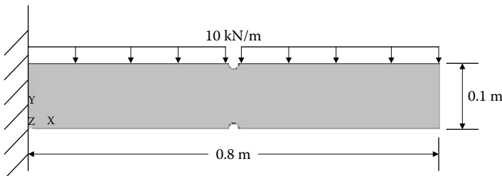
Figure P13.2 Geometry of a cantilevered beam for Project 13.2. (See color insert.)
