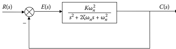
Figure P14.5a Block diagram of the closed-loop DC drive.
