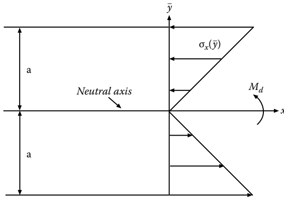
Figure A.1d Section stress distribution.
