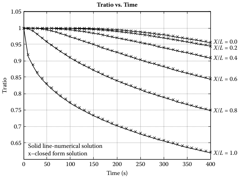
Figure P10.5 The plot of TRATIO vs. time. Numerical solution is by the implicit method.
