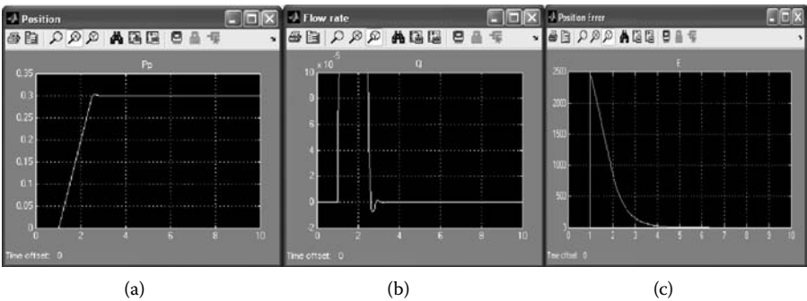
Figure 14.67 Simulation results (for a controller gain of 0.01 and T = 0.01 second): (a) piston position; (b) flow rate through the valve; (c) position error. (From MATLAB. With permission.)
