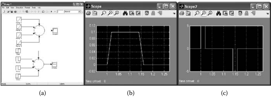
Figure 14.52 Bump simulation: (a) Simulink model; (b) x_r ; (c) \dot{x}_r . (From MATLAB. With permission.)
