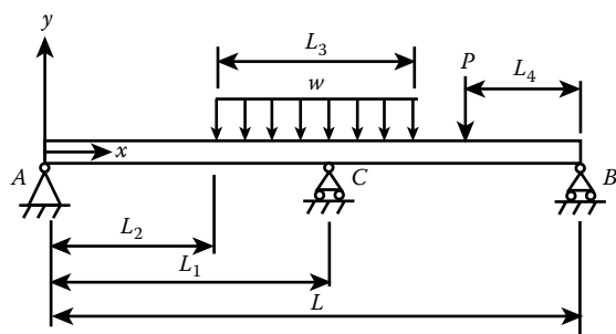
Figure P6.9a Indeterminate beam structure.
