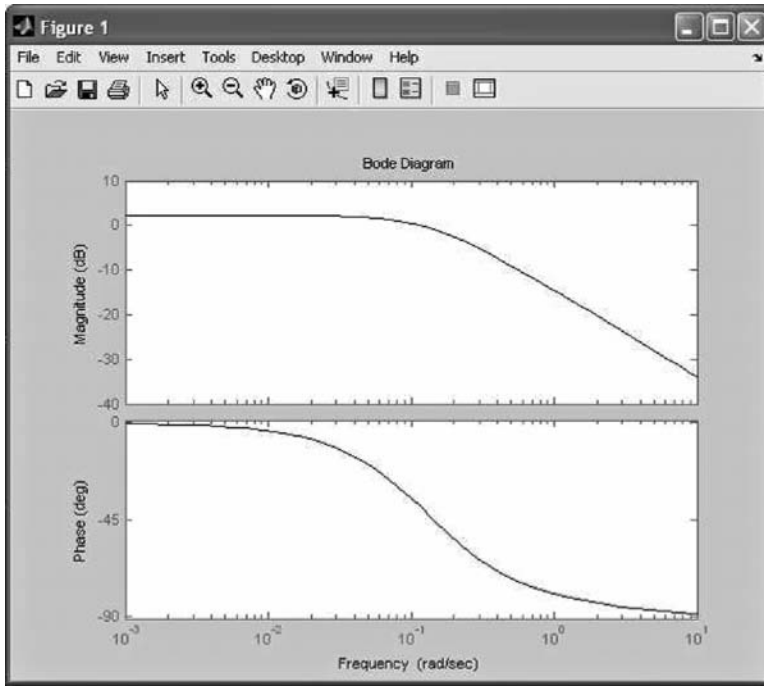
Figure 14.8 Bode plots for the Coupled Tanks system. (From MATLAB. With permission.)
