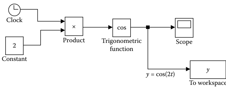
Figure 7.14 Block diagram using the clock, the trig function, and the workspace blocks.
