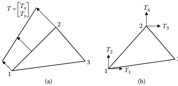
Figure 13.8 (a) Surface tractions T acting on the edge of an element. (b) Equivalent nodal force at each node due to the surface tractions.
