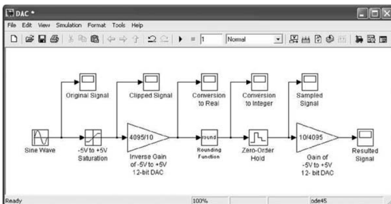
Figure 14.61 Digital-to-analog converter implementation. (From MATLAB. With permission.)
