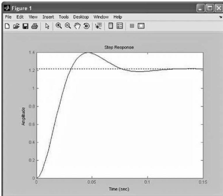
Figure 14.13 Step response for the model shown in Figure 14.10. (From MATLAB. With permission.)
