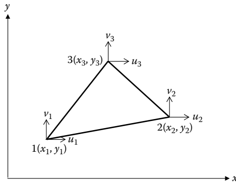
Figure 13.4 Linear triangular element for 2-D stress analysis.
