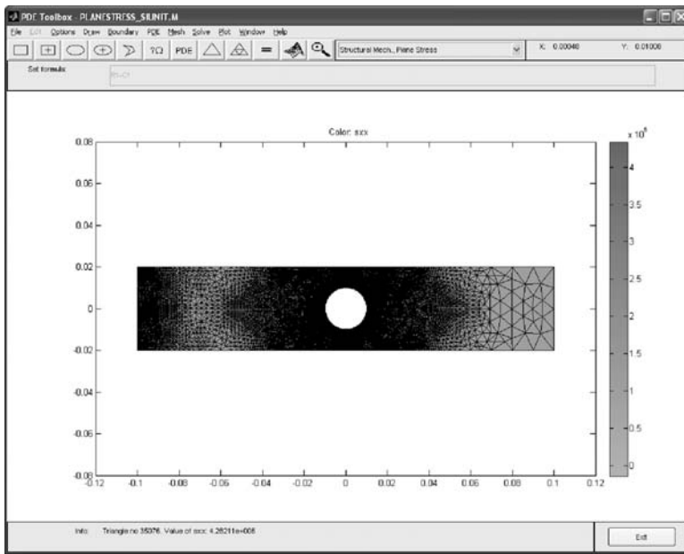
Figure 13.38 Contour plot of \sigma_x obtained from adaptive solution mode. (From MATLAB. With permission.)
