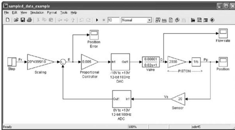
Figure 14.65 Simulink implementation of the position control system that is shown in Figure 14.63. (From MATLAB. With permission.)
