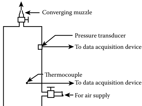
Figure P6.6 Air pressurized tank.
