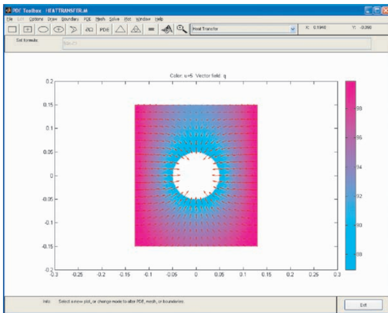
Figure 13.56 Contour plot of the temperature field with heat flux flow. (From MATLAB. With permission.)
