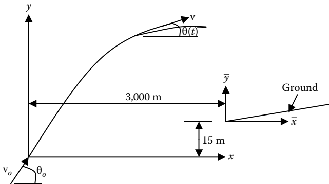
Figure P6.2 Rocket trajectory.
