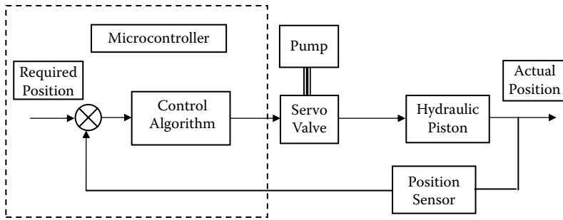
Figure 14.63 Block diagram of a position sampled data control system.
