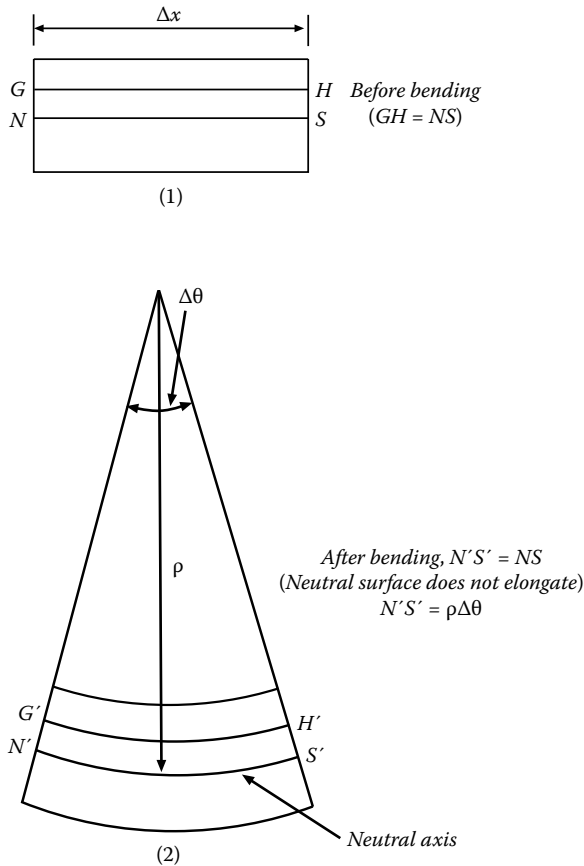
Figure A.1c Normal stress causing a section bending moment. (1) Beam element GH before beam bending; (2) beam element GH after beam bending.
