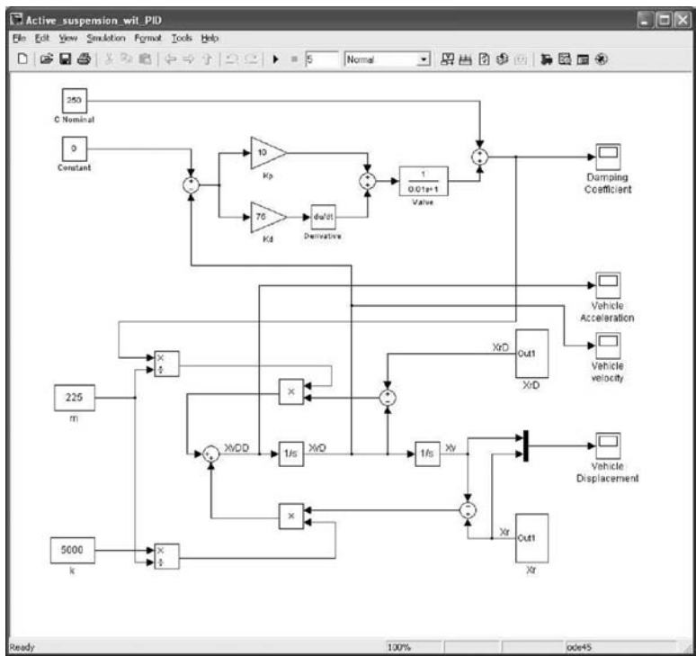
Figure 14.55 Controller implementation. (From MATLAB. With permission.)
