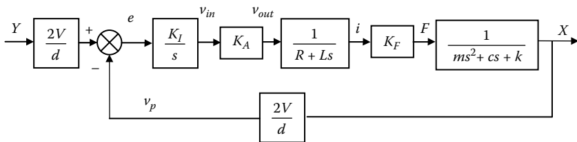
Figure 14.24 Block diagram of the system shown in Figure 14.22.
