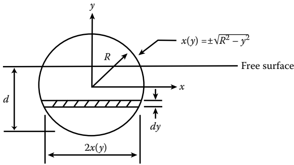
Figure P4.5 Floating log having a circular cross-section.
