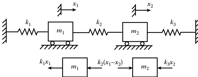
Figure 3.8 Two-degrees-of-freedom vibration system.
