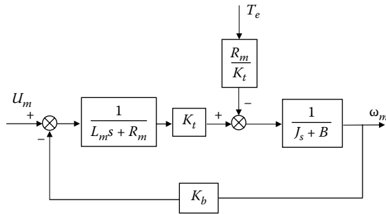
Figure 14.12 Block diagram of a DC motor.
