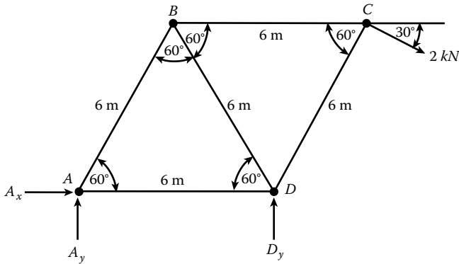
Figure 3.2 Reactions of simple truss.
