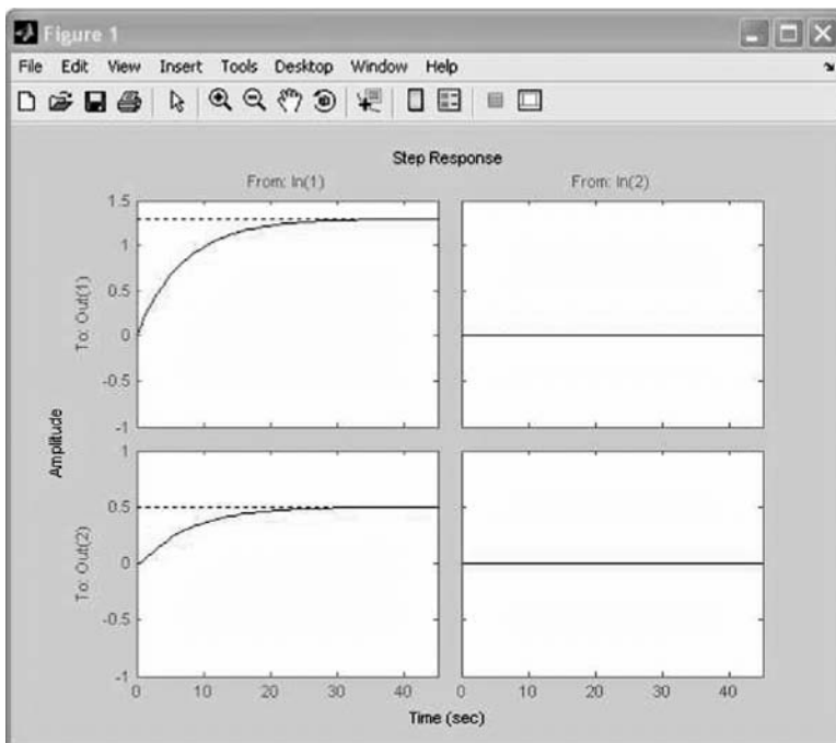
Figure 14.9 System's response to unit step input. (From MATLAB. With permission.)
