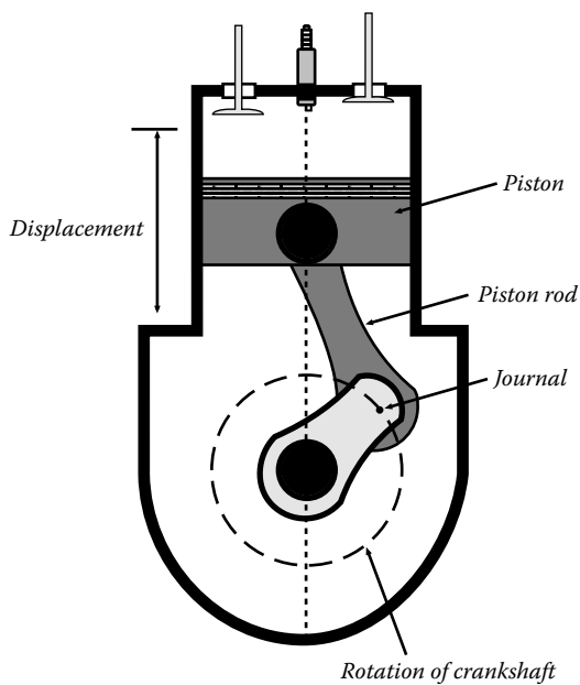
Figure P2.12a Sketch of a typical piston-cylinder engine.
