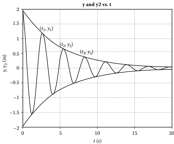
Figure 8.1 Oscilloscope graph of free damped oscillations.
