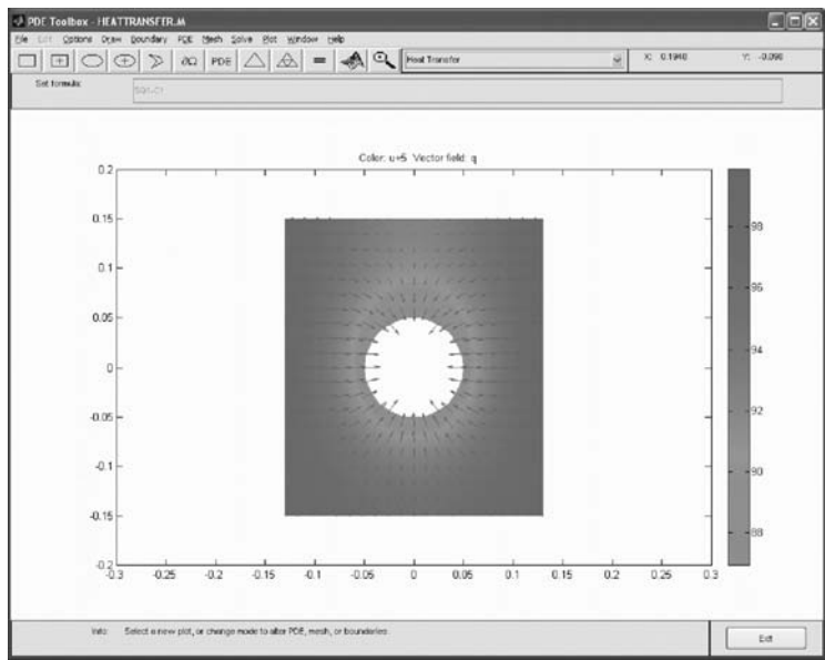
Figure 13.56 Contour plot of the temperature field with heat flux flow. (From MATLAB. With permission.) (See color insert.)
