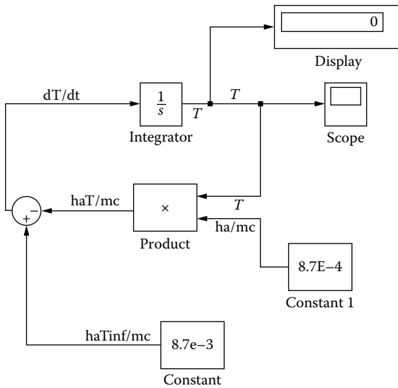
Figure 7.7 Block diagram for solving Equation (7.2).
