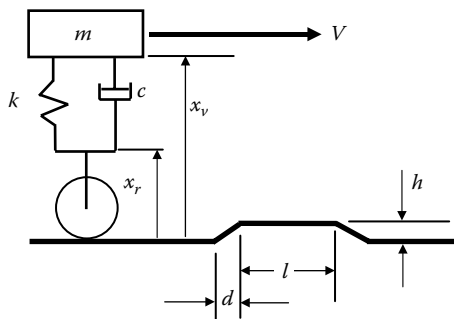
Figure 14.51 A model of the suspension of a single wheel.
