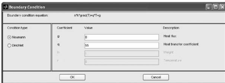
Figure 13.50 Boundary condition window for input of the Neumann boundary condition to specify the heat transfer coefficient for the convection edge. (From MATLAB. With permission.)
