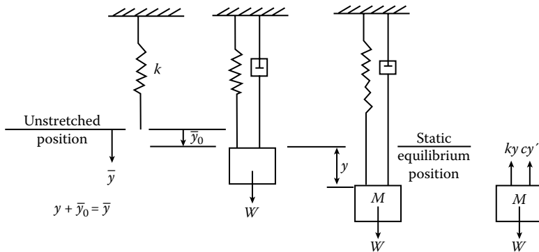
Figure P2.10 Spring-dashpot system.
