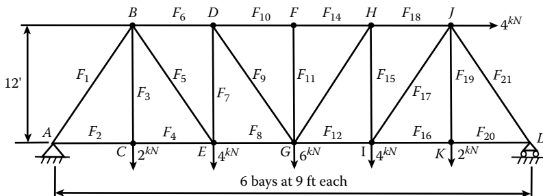
Figure P3.1 Truss structure for Project 3.1.
