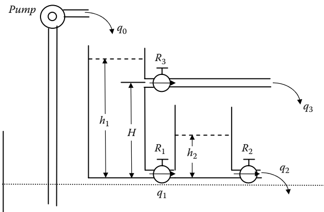
Figure P14.4 Schematic of the tanks for Project 14.4.
