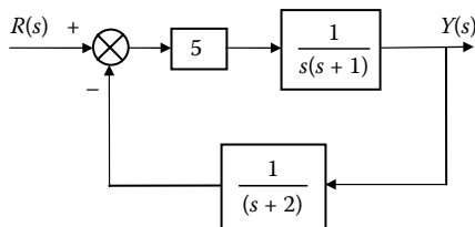
Figure 14.17 Closed-loop system.
