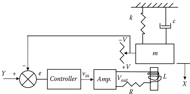
Figure 14.22 Example for SISOtool .
