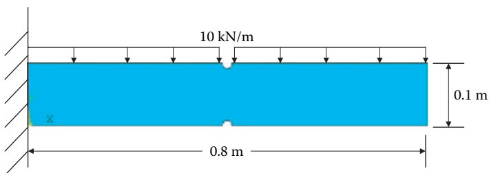
Figure P13.2 Geometry of a cantilevered beam for Project 13.2.
