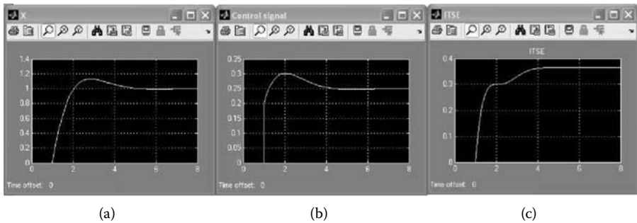
Figure 14.50 Optimum response: (a) X ; (b) u ; (c) ITSE. (From MATLAB. With permission.)
