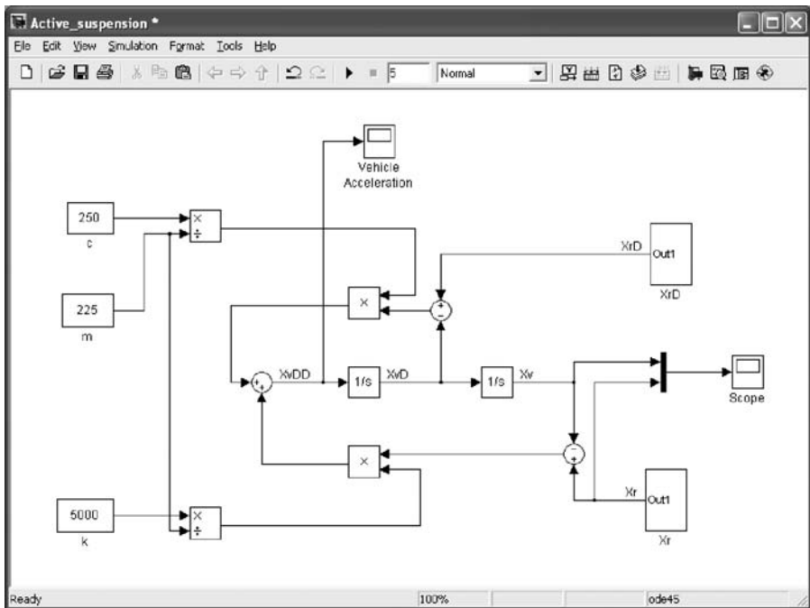
Figure 14.53 Simulink implementation of the suspension model. (From MATLAB. With permission.)
