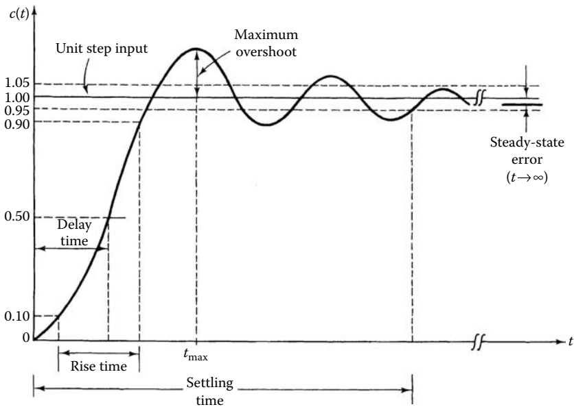
Figure 14.3 Typical system's response to unit step input.
