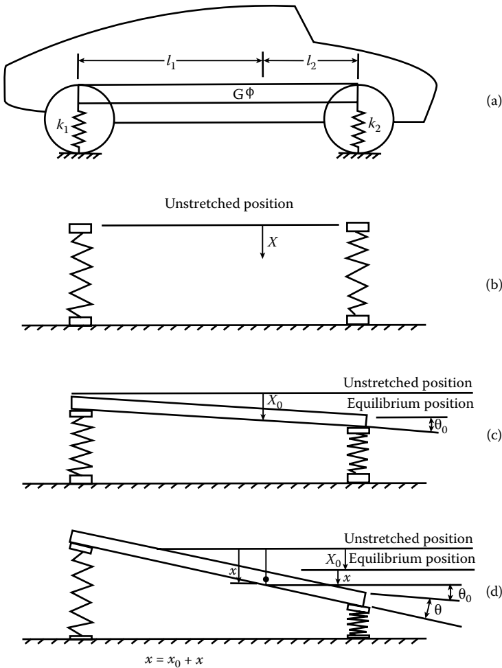
Figure P3.3 Automobile suspension system.
