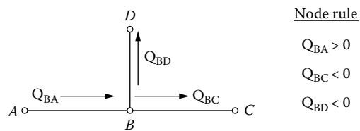
Figure 11.3 Node rule for pipe network.
