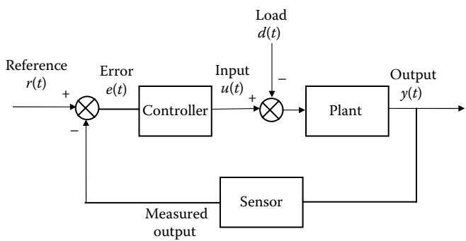
Figure 14.1 A typical structure of control system.
