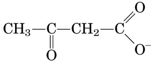
Acetoacetate
