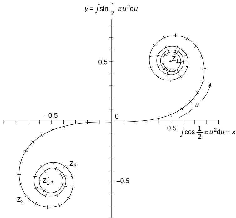
Figure 12.42 Cornu spiral associated with Fresnel diffraction. The spiral in the first quadrant represents the contribution from the upper half of an infinite plane wavefront above an infinite straight edge. The third quadrant spiral results from the downward withdrawal of the straight edge. The width of the wavefront contributing to the diffraction pattern is correlated with the length u along the spiral. The upper half of the wavefront above the straight edge contributes an intensity (OZ_1)^2 which is the square of the length of the chord from the origin to the spiral eye. This intensity is 0.25 of the intensity (Z_1Z_1')^2 due to the whole wavefront
