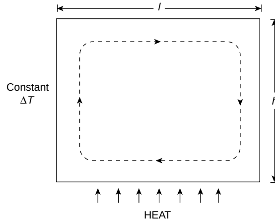
Figure 14.40 The first mode X(t) in the Lorenz equations gives a single convective roll, clockwise for X positive, anti-clockwise for X negative. Warm rising fluid in this mode indicates where X and Y have the same sign. The ratio h/l determines the geometric factor b in the Lorenz equations
