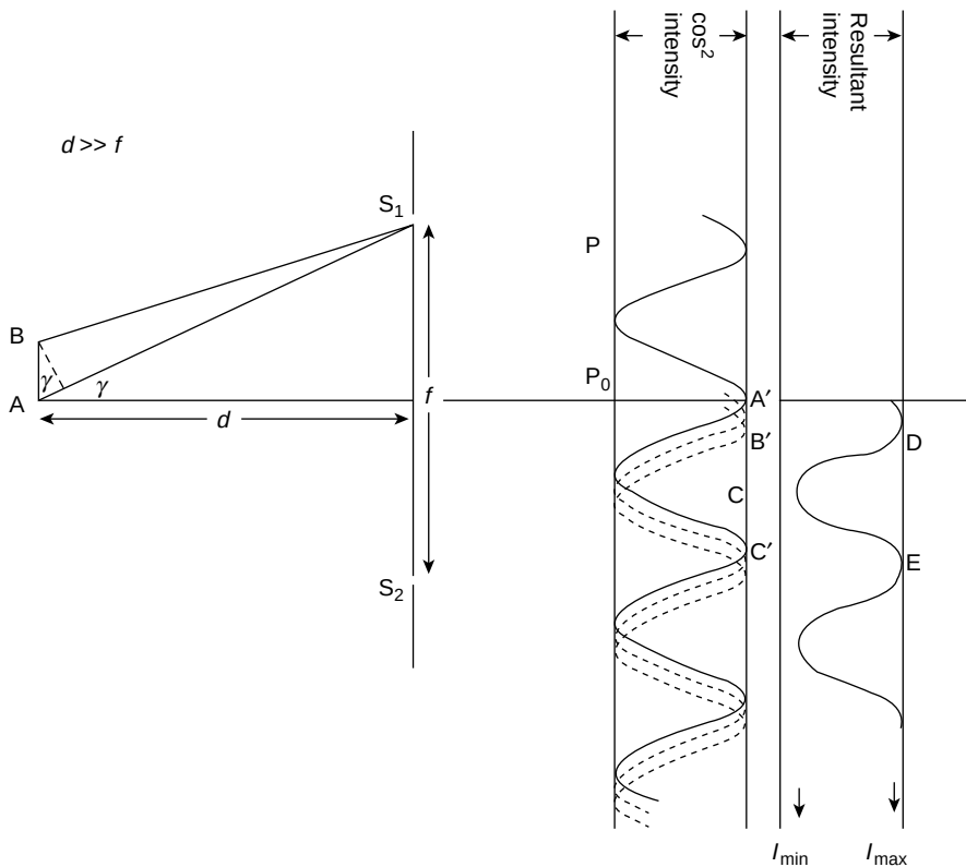
Figure 12.18 The point source A produces the \cos^2 interference fringes represented by the solid curve A'C'. Other points on the line source AB produce \cos^2 fringes (the displaced broken curves B'C') and the observed total intensity is the curve DE. When the points on AB extend A'B' to C the fringes disappear and the field is uniformly illuminated
