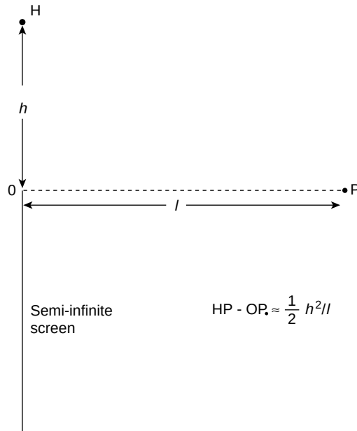
Figure 12.44 Line OP normal to the straight edge defines the geometric shadow. The wavefront at height h above O makes a contribution to the disturbance at P which has a phase lag of \pi h^2/\lambda l with respect to that from O. The total disturbance at P is the vector sum (amplitude and phase) of all contributions from the wavefront section above O
