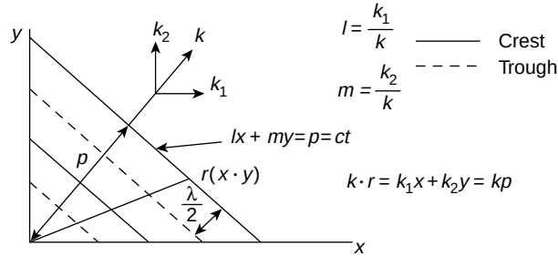
Figure 9.1 Crests and troughs of a two-dimensional plane wave propagating in a general direction \mathbf{k} (direction cosines l and m ). The wave is specified by lx + my = p = ct , where p is its perpendicular distance from the origin, travelled in a time t at a velocity c
