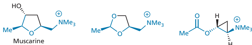
FIGURE 22.14 Rigid molecules incorporating the acetylcholine skeleton ( \text{C-C-O-C-C-N} ).
