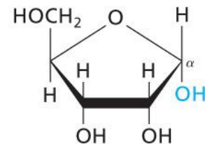
\alpha -D-Ribofuranose (Haworth projection)
