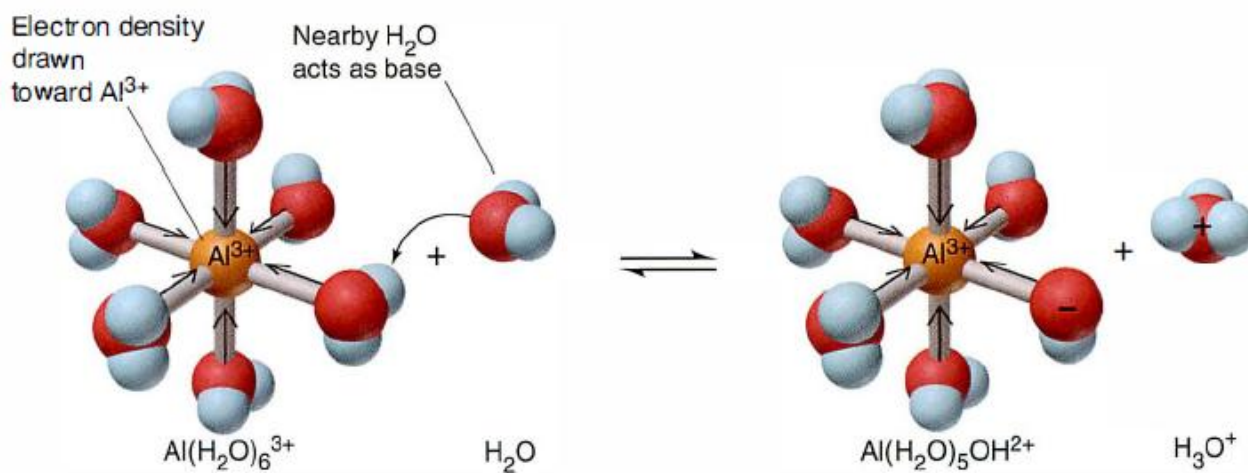
Figure 18.13 The acidic behavior of the hydrated \text{Al}^{3+} ion. When a metal ion enters water, it is hydrated as water molecules bond to it. If the ion is small and multiply charged, as is the \text{Al}^{3+} ion, it pulls sufficient electron density from the O-H bonds of the attached water molecules to make the bonds more polar, and an \text{H}^+ ion is transferred to a nearby water molecule.
