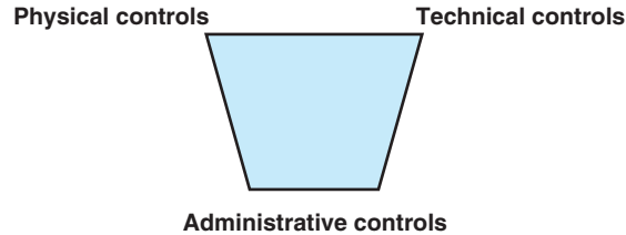
FIGURE 11.2 Control Taxonomy
