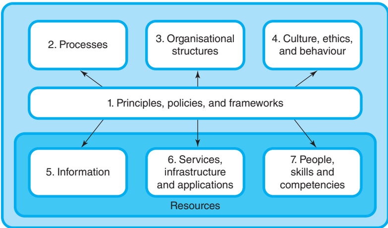
FIGURE 11.4 CoBIT 5 Enablers
