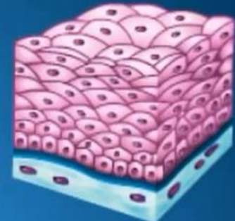
Stratified Epithelium
