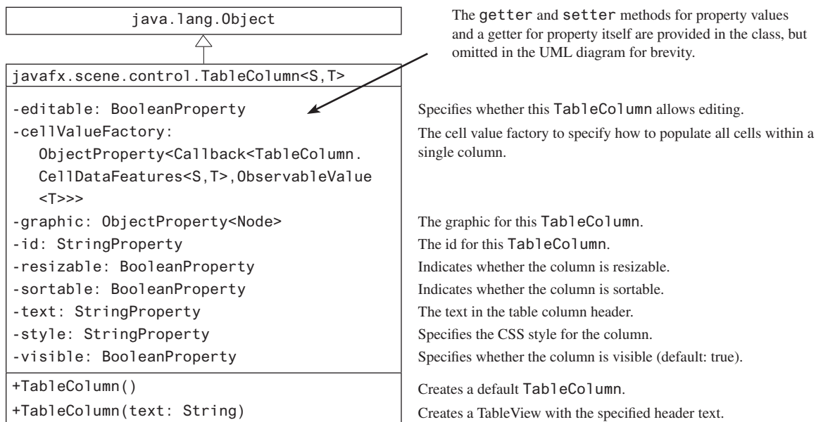
FIGURE 31.32 TableColumn defines a column in the TableView .
