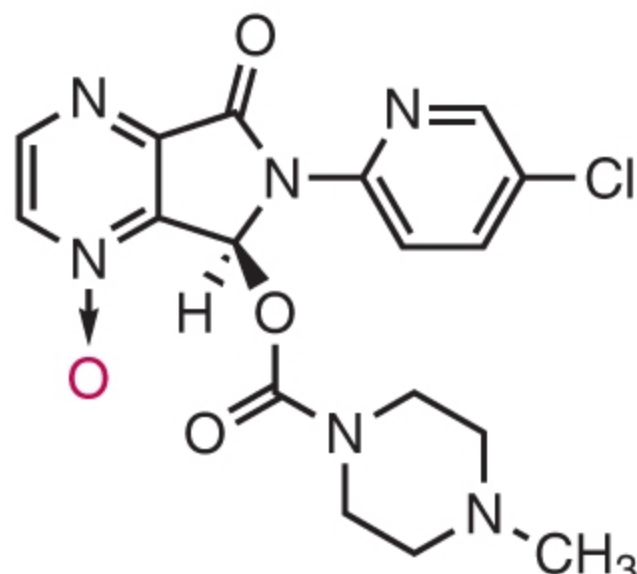
(S)-N-oxidezopiclone (inactive)
