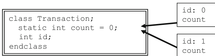
Fig. 5.2 Static variables in a class
