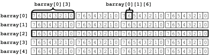
Fig. 2.3 Packed array bit layout
