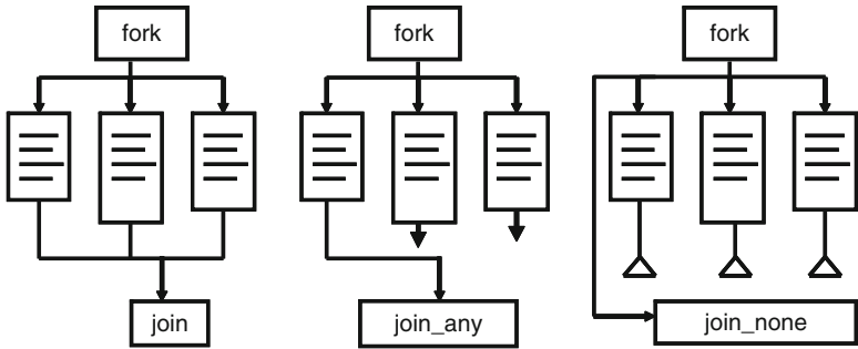
Fig. 7.2 Fork...join blocks
