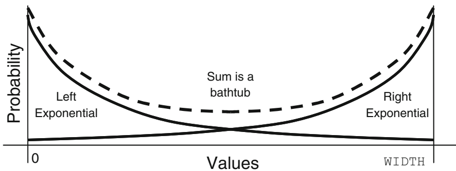
Fig. 6.1 Building a bathtub distribution
