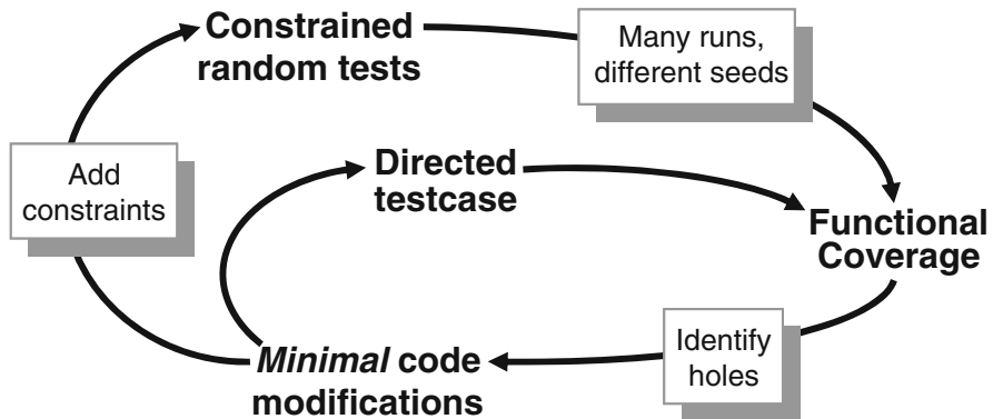
Fig. 9.1 Coverage convergence
