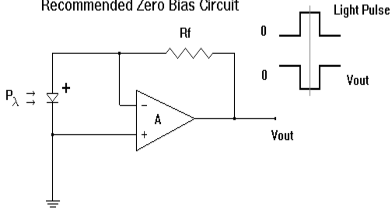
Recommended Zero Bias Circuit
