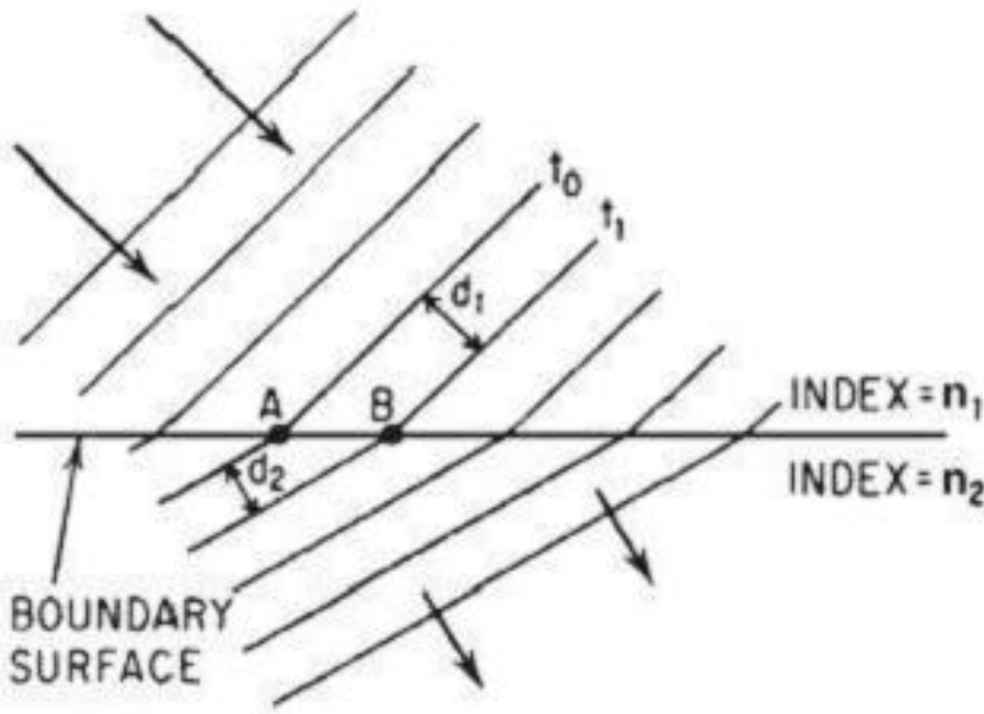
Figure 1.4 A plane wave front passing through the boundary between two media of differing indices of refraction ( n_2 > n_1 ).
