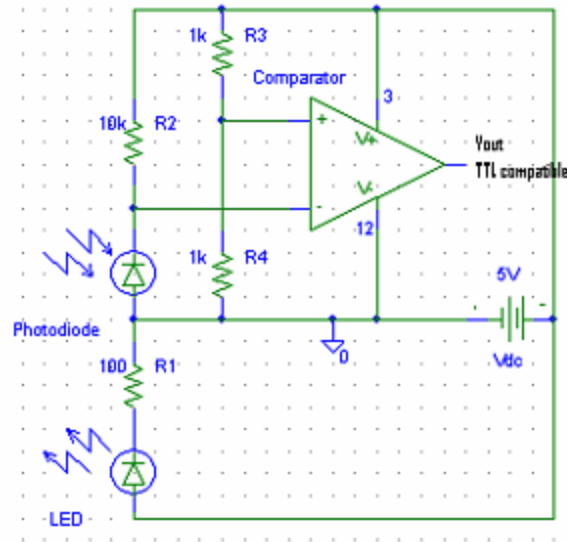
Negative Bias Circuit
