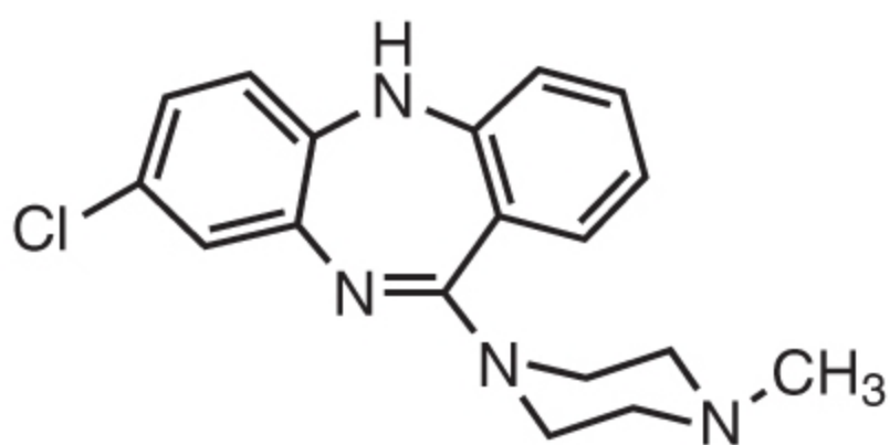
Clozapine
