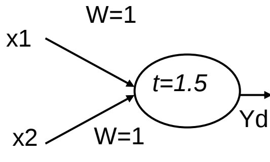
AND
