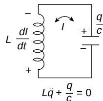
Figure 1.5 Electrical system which oscillates simple harmonically. The sum of the voltages around the circuit is given by Kirchhoff's law as L \frac{di}{dt} + \frac{q}{C} = 0
