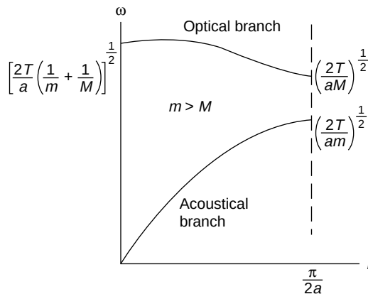
Figure 5.17 Dispersion relations for the two modes of transverse oscillation in a crystal structure
