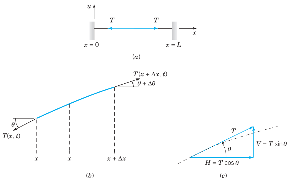
FIGURE 10.B.1 (a) An elastic string under tension. (b) An element of the displaced string. (c) Resolution of the tension T into components.
