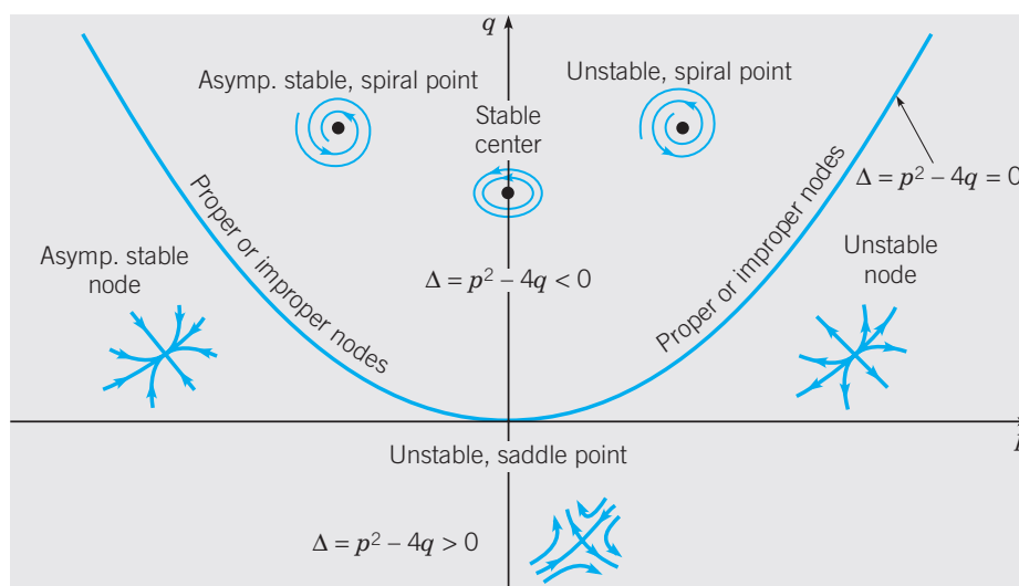
FIGURE 9.1.9 Stability diagram.
