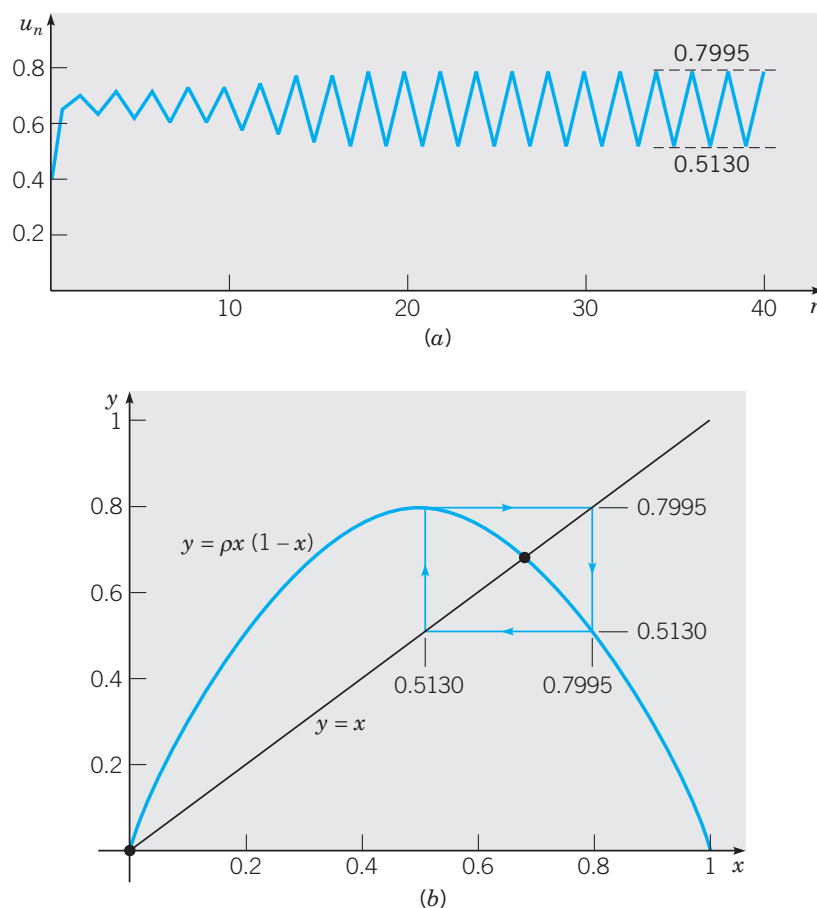
FIGURE 2.9.4 A solution of u_{n+1} = \rho u_n(1 - u_n) for \rho = 3.2 ; period 2. (a) u_n versus n ; (b) a two-cycle.
