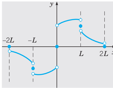
FIGURE 10.4.6 Graph of the function in Problem 38.
