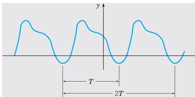
FIGURE 10.2.1 A periodic function of period T .
