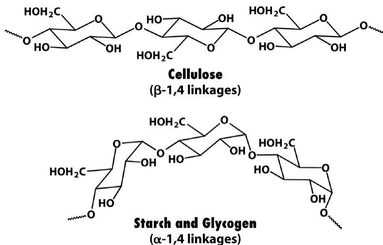
Figure 11-14 Biochemistry, Sixth Edition © 2007 W. H. Freeman and Company
