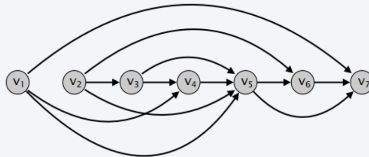
a topological ordering
