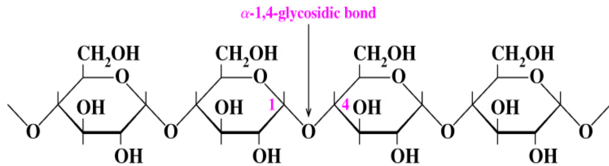
(a) Unbranched chain of amylose
