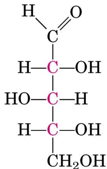
D-Xylose
