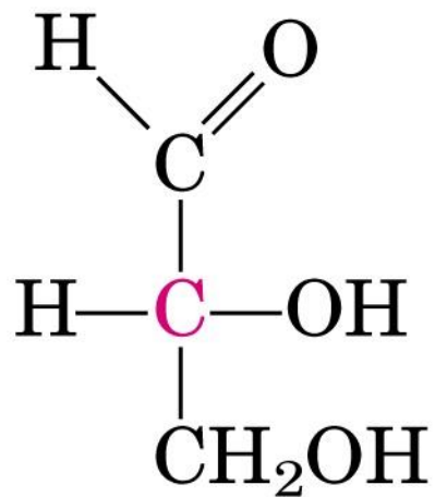
D-Glyceraldehyde
