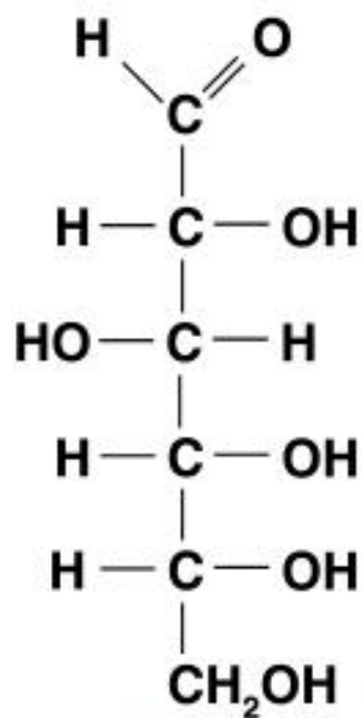
D-Glucose
