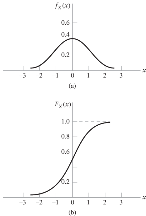
FIGURE 8.10 The normalized Gaussian distribution. (a) The probability density function. (b) The distribution function.
