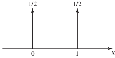
FIGURE 8.4 Illustration of probability mass function for coin-tossing experiment.
