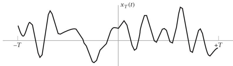
FIGURE 8.17 Sample function of a random process.
