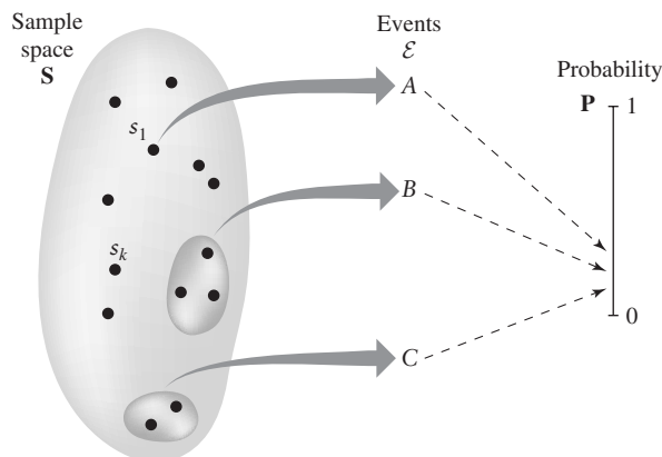
FIGURE 8.2 Illustration of the relationship between sample space, events, and probability.
