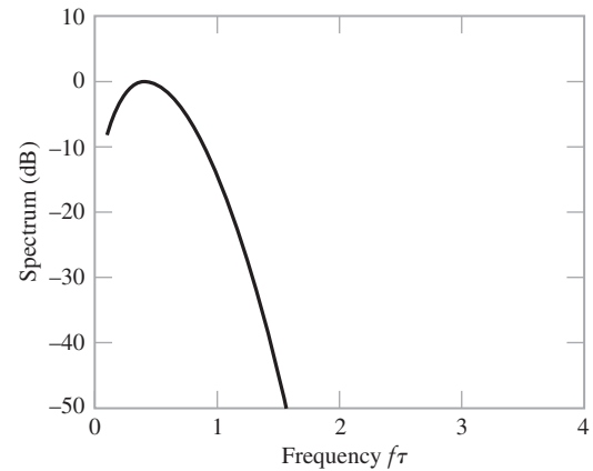
FIGURE 5.23 Spectrum of Gaussian monocycle.
