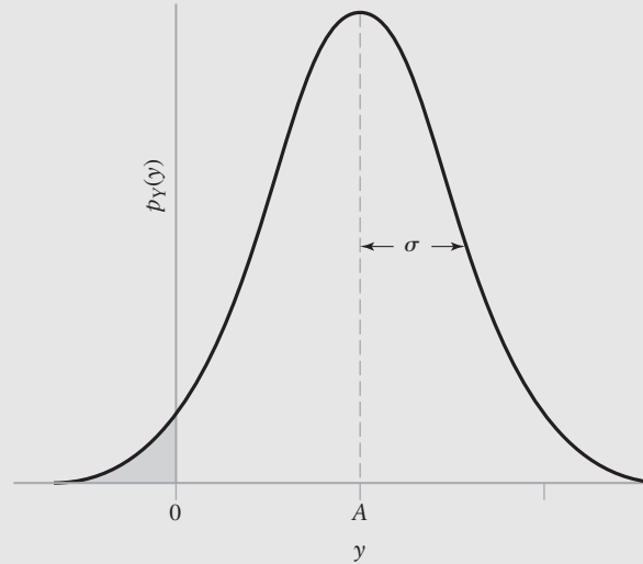
FIGURE 8.12 Density function of noisy PAM signal Y .
