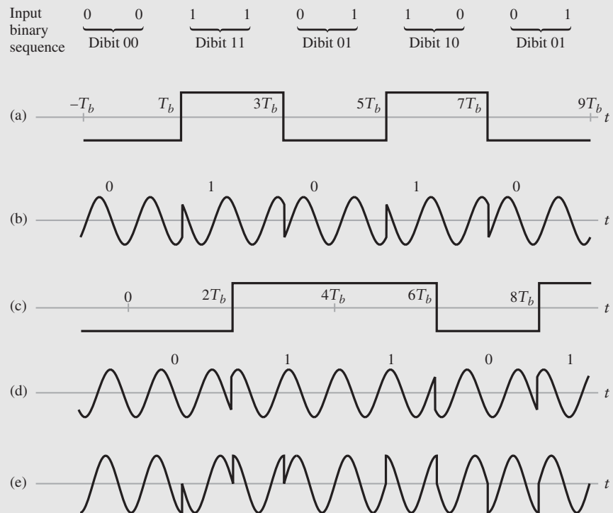
FIGURE 7.13 OQPSK signal components: (a) Modulating signal for in-phase component. (b) Modulated waveform of in-phase component. (c) Modulating signal for quadrature component. (d) Modulated waveform of quadrature component. (e) Waveform of OQPSK signal obtained by subtracting (d) from (b).
