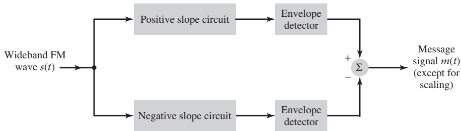
FIGURE 4.13 Block diagram of balanced frequency discriminator.
