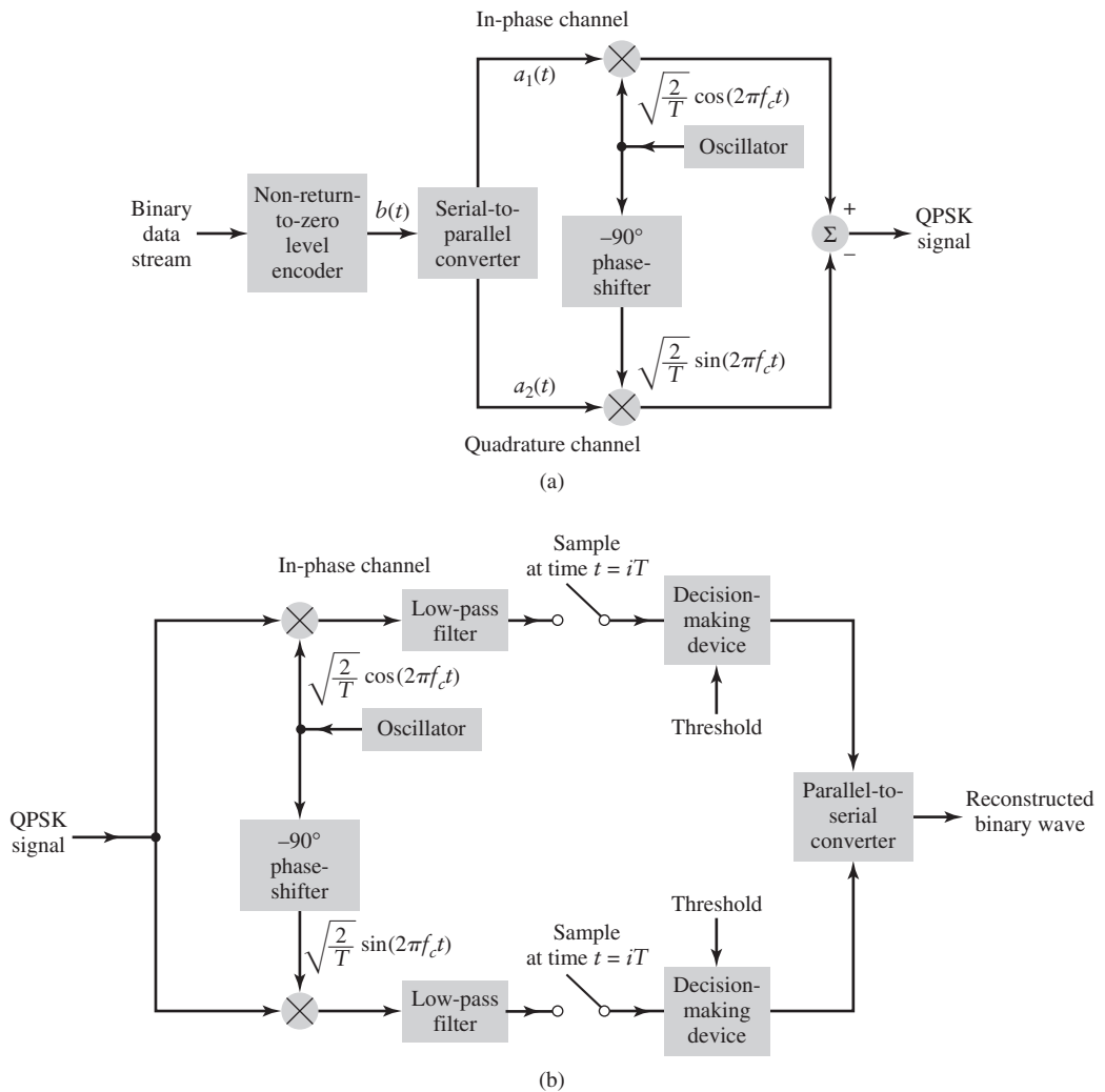
FIGURE 7.7 Block diagrams of (a) QPSK transmitter and (b) coherent QPSK receiver; for the two synchronous samplers, integer i = 0, \pm 1, \pm 2, \dots
