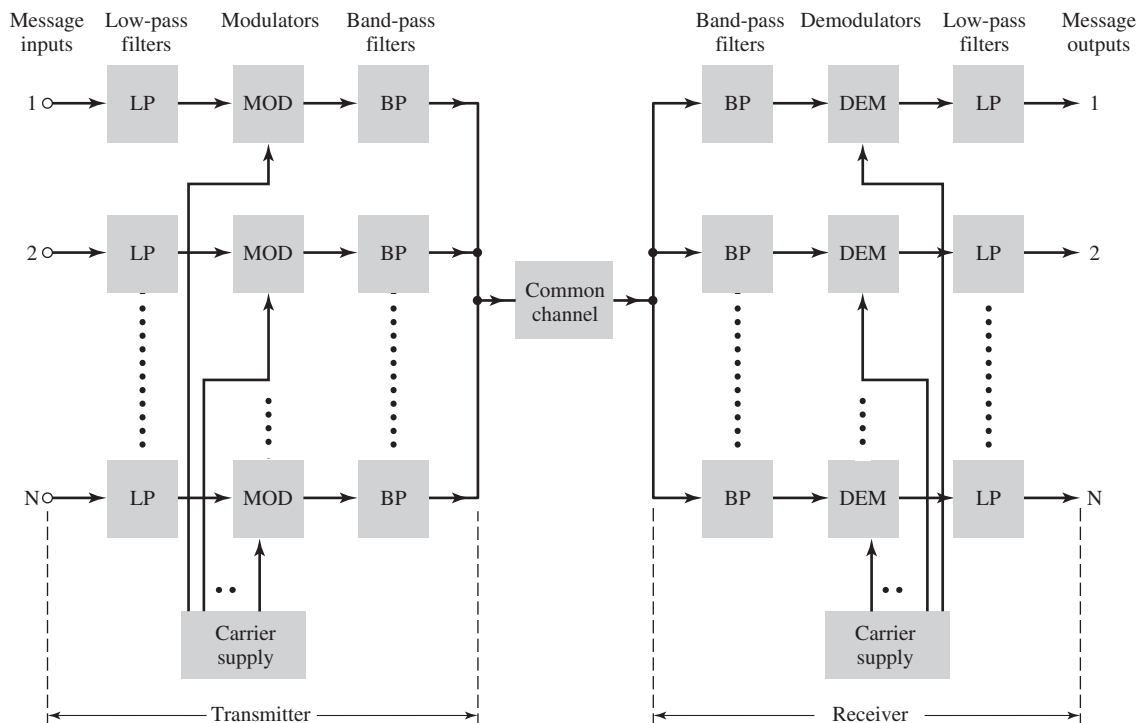
FIGURE 3.29 Block diagram of frequency-division multiplexing (FDM) system.
