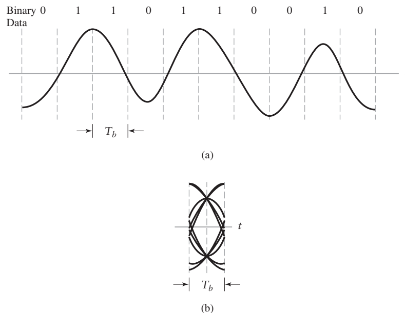
FIGURE 6.5 (a) Binary data sequence and its waveform. (b) Corresponding eye pattern.
