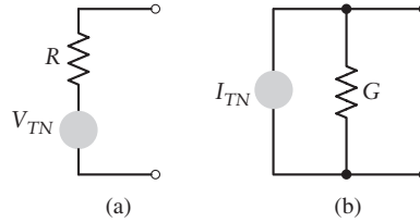
FIGURE 11.1 Models of a noisy resistor: (a) Thévenin equivalent circuit and (b) Norton equivalent circuit.
