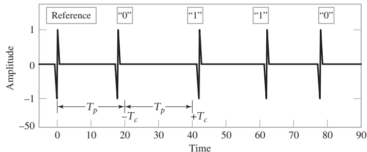
FIGURE 5.24 Pulse-position modulation of impulse radio.
