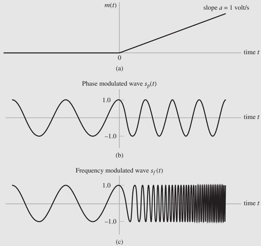
FIGURE 4.2 Starting at time t = 0 , the figure displays (a) linearly increasing message signal m(t) , (b) phase-modulated wave, and (c) frequency-modulated wave.
