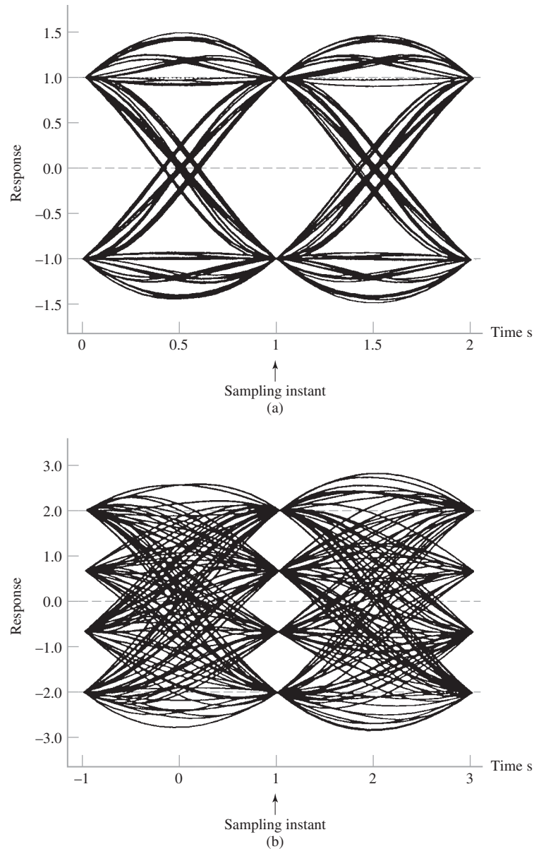
FIGURE 6.8 Eye diagram of received signal with no bandwidth limitation. (a) M = 2 . (b) M = 4 .
