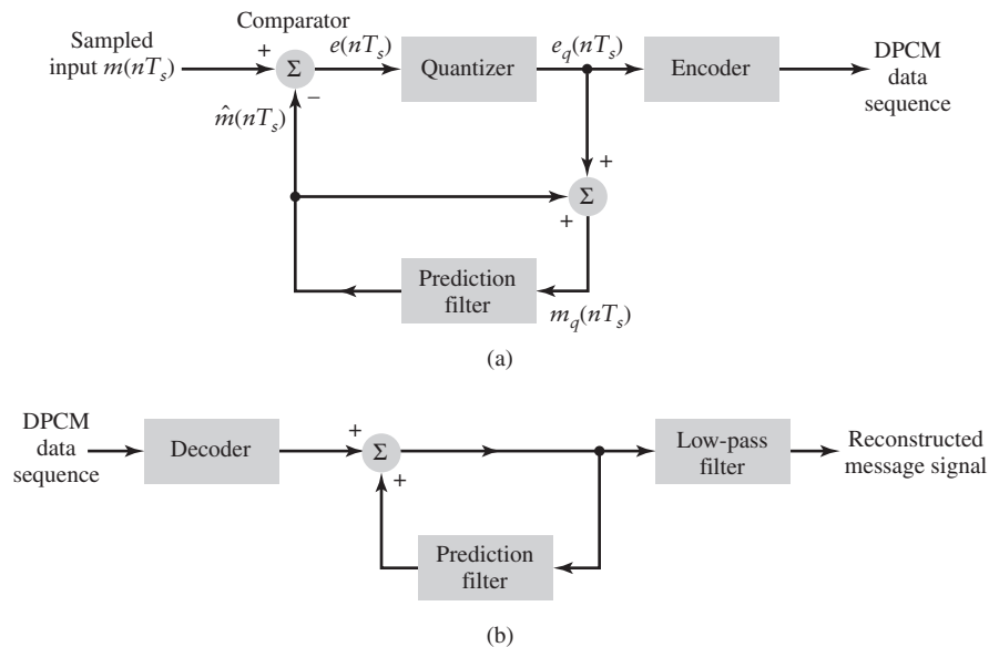
FIGURE 5.18 DPCM system: (a) Transmitter and (b) receiver.
