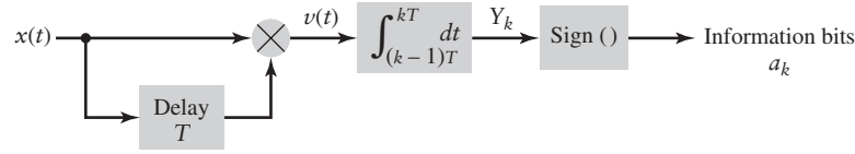
FIGURE 10.14 Differential detector.
