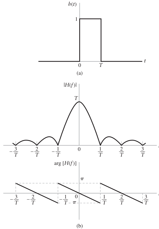
FIGURE 5.6 (a) Rectangular pulse b(t) . (b) Spectrum H(f) , defined in terms of its magnitude and phase.
