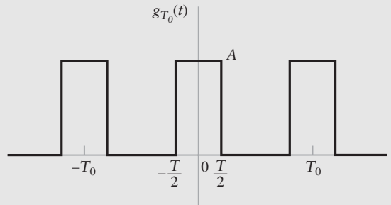
FIGURE A2.1 Periodic train of rectangular pulses of amplitude A , duration T , and period T_0 .
