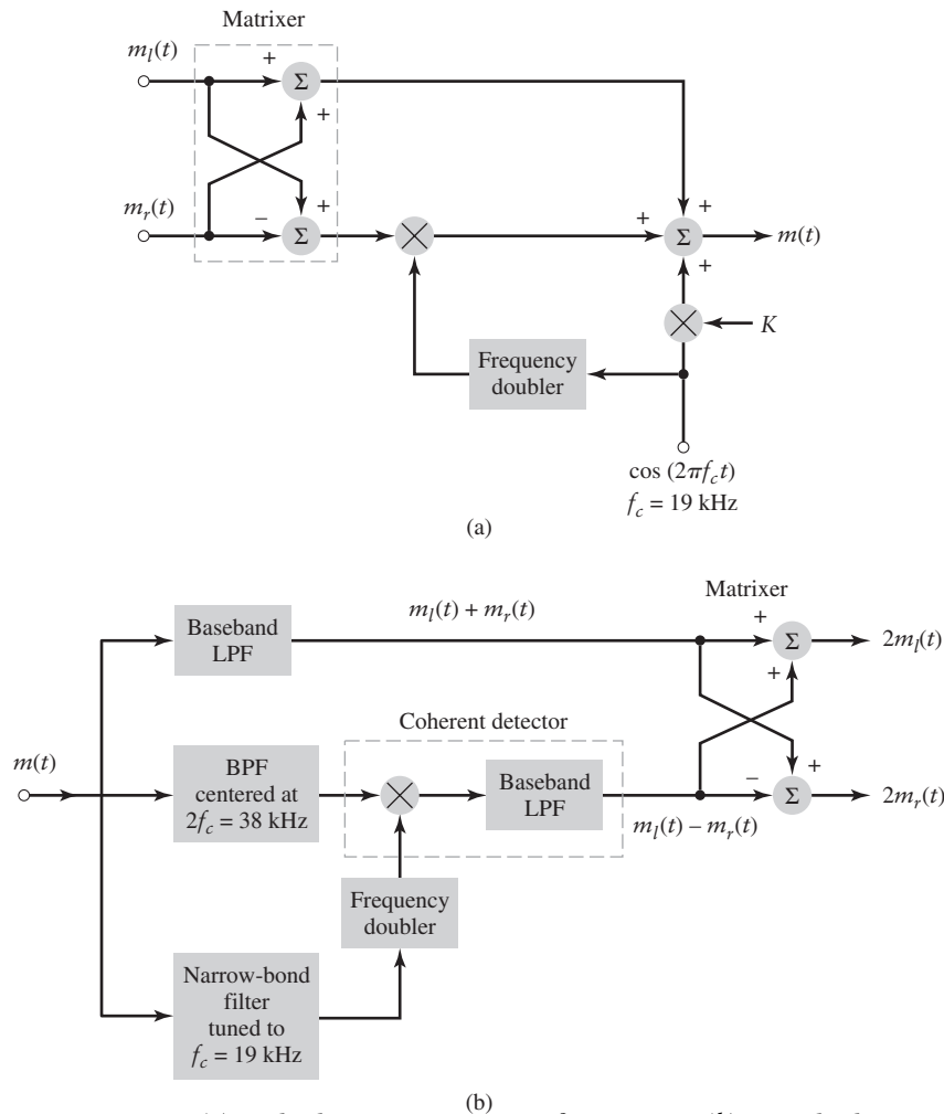
FIGURE 4.16 (a) Multiplexer in transmitter of FM stereo. (b) Demultiplexer in receiver of FM stereo.
