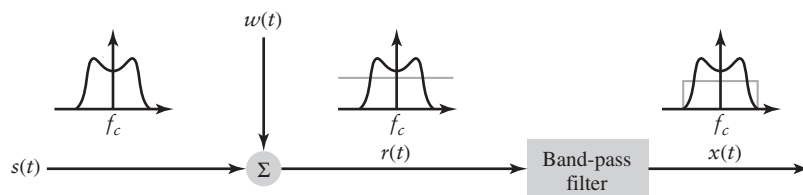
FIGURE 9.1 Block diagram of signal plus noise before and after filtering, showing spectra at each point.
