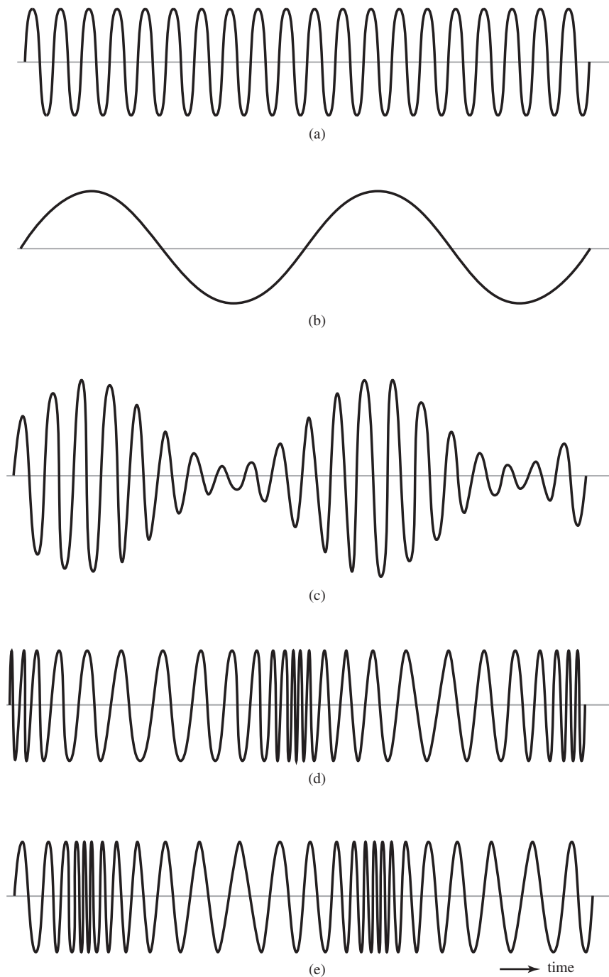
FIGURE 4.1 Illustration of AM, PM, and FM waves produced by a single tone. (a) Carrier wave. (b) Sinusoidal modulating signal. (c) Amplitude-modulated signal. (d) Phase-modulated signal. (e) Frequency modulated signal.
