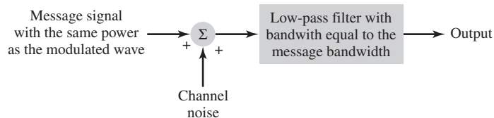
FIGURE 9.4 Reference transmission model for analog communications.
