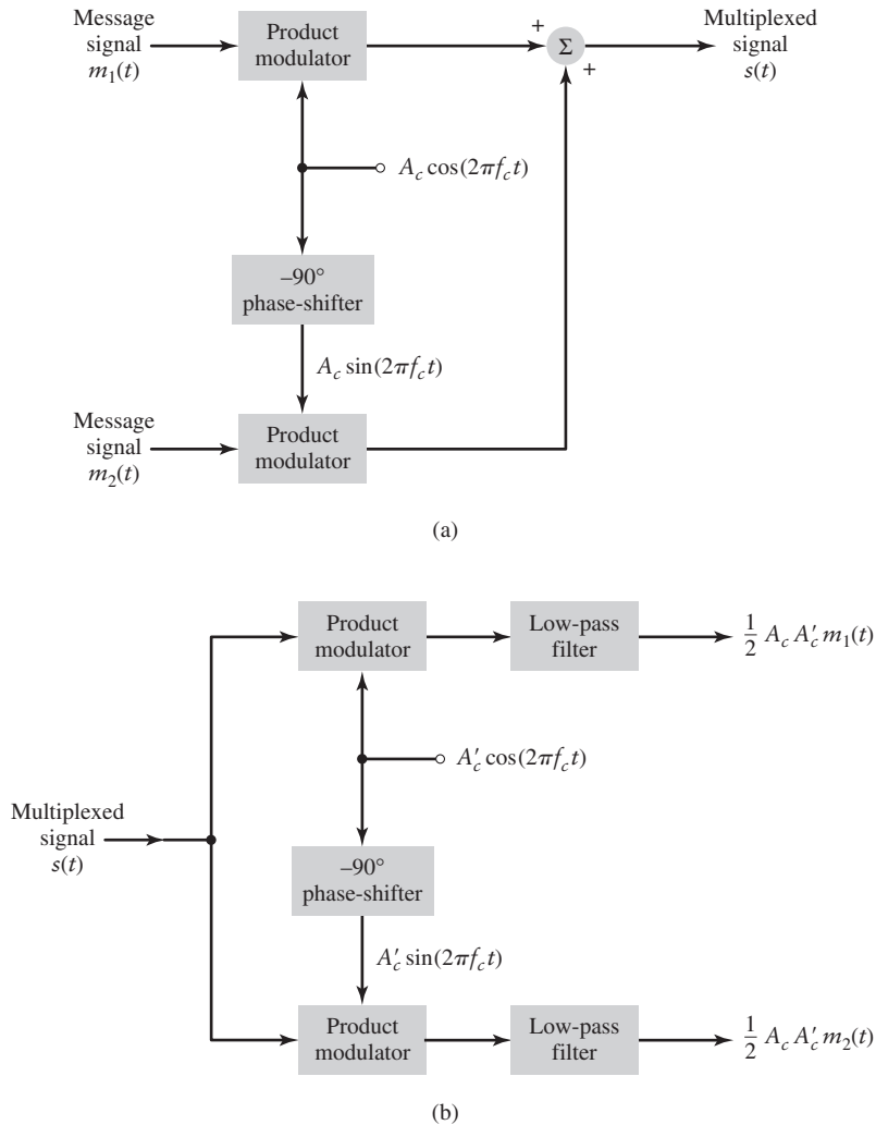
FIGURE 3.17 Quadrature-carrier multiplexing system: (a) Transmitter, (b) receiver.
