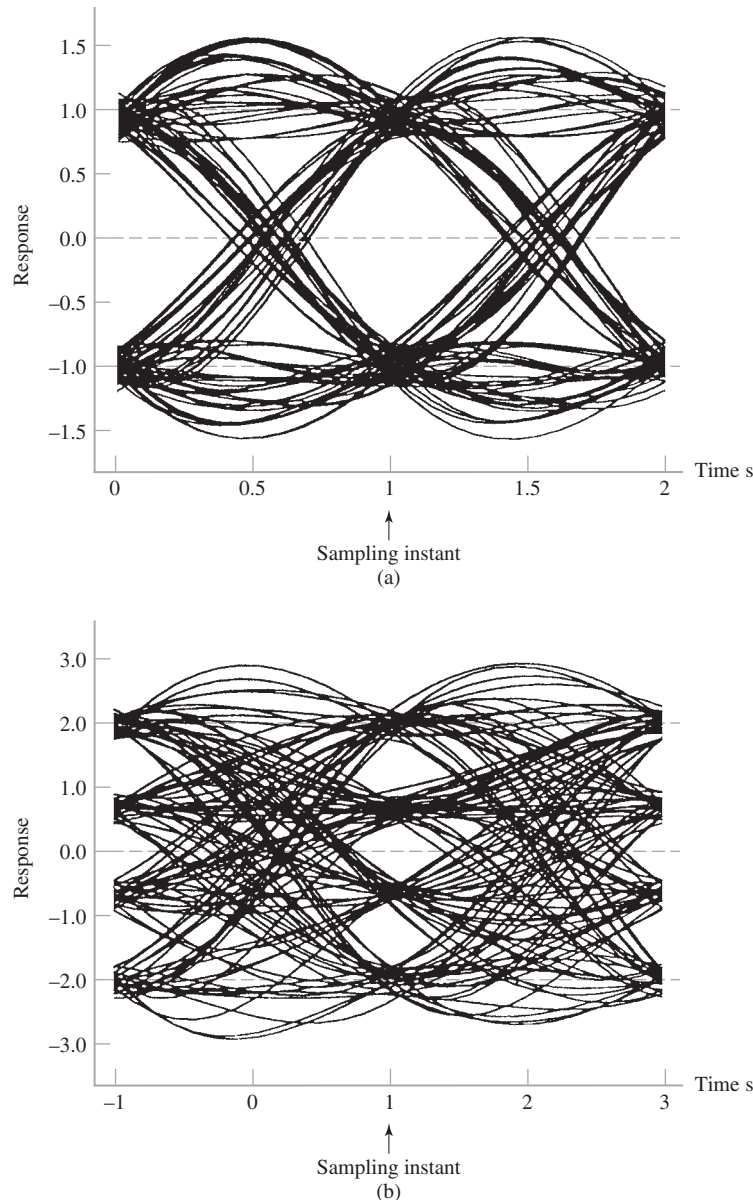
FIGURE 6.9 Eye diagram of received signal, using a bandwidth-limited channel. (a) M = 2 . (b) M = 4 .
