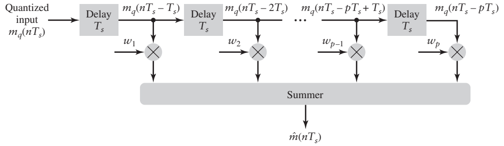
FIGURE 5.19 Tapped-delay line filter used as prediction filter.
