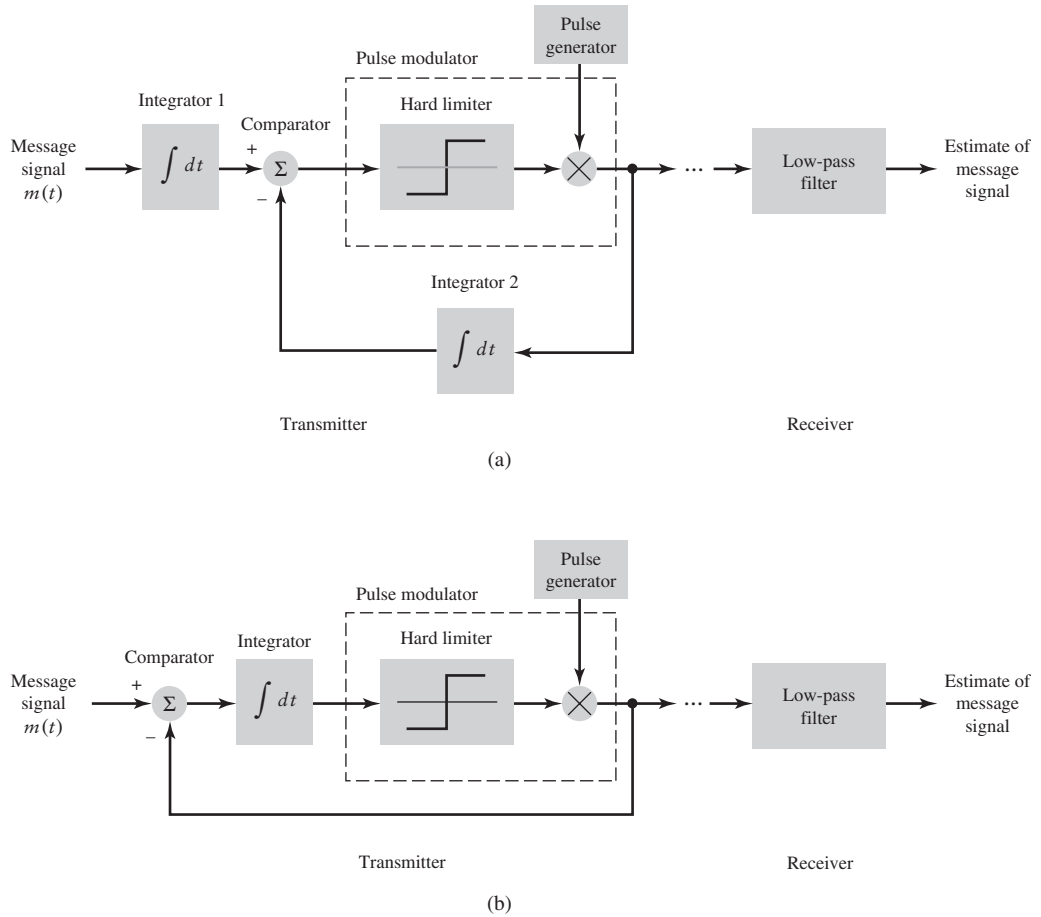
FIGURE 5.17 Two equivalent versions of delta-sigma modulation system: the system shown in part (b) of the figure is a simplified version of the system in part (a).
