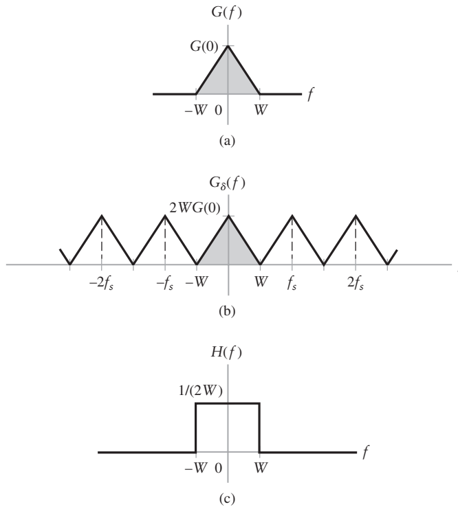
FIGURE 5.2 (a) Spectrum of a strictly band-limited signal g(t) . (b) Spectrum of instantaneously sampled version of g(t) for a sampling period T_s = 1/2W . (c) Frequency response of ideal low-pass filter aimed at recovering the original message signal g(t) from its uniformly sampled version.
