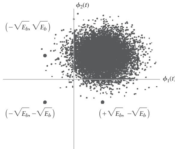
FIGURE 10.17 Signal space representation of noisy constellation.
