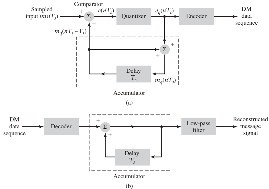
FIGURE 5.15 DM system: (a) Transmitter and (b) receiver.
