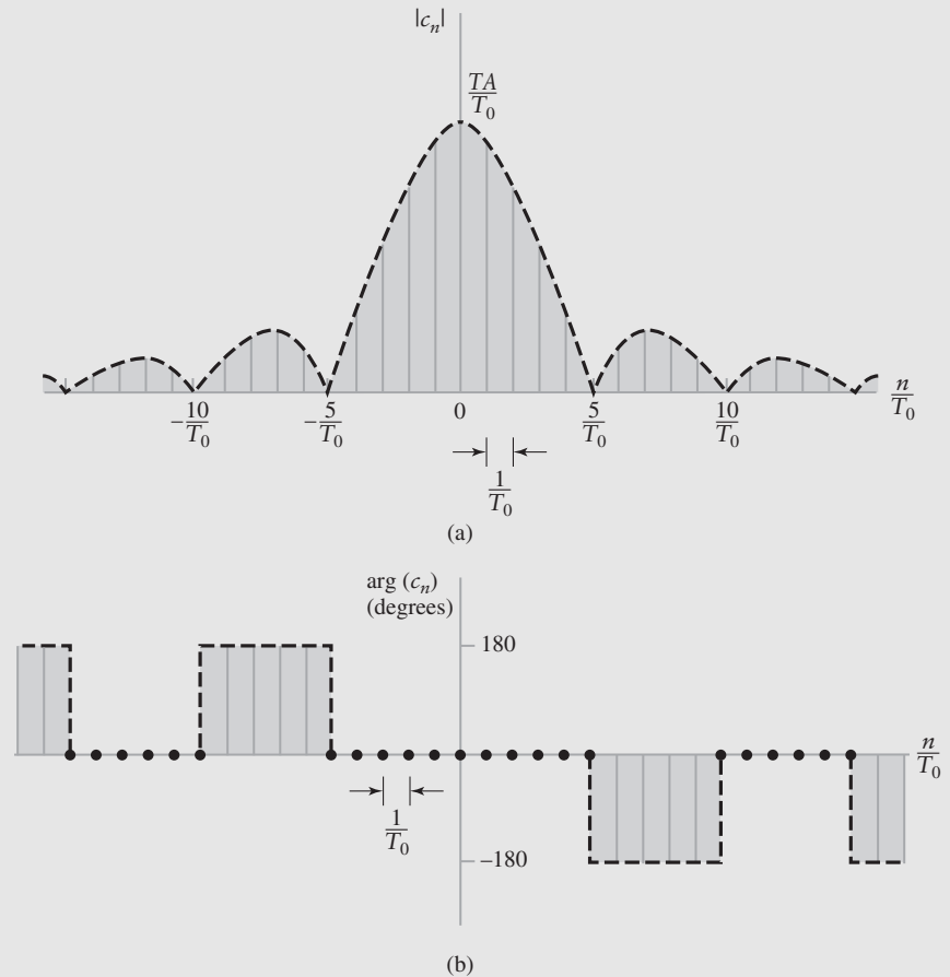
FIGURE A2.2 Discrete spectrum of a periodic train of rectangular pulses for a duty cycle T/T_0 = 0.2 . (a) Amplitude spectrum. (b) Phase spectrum.
