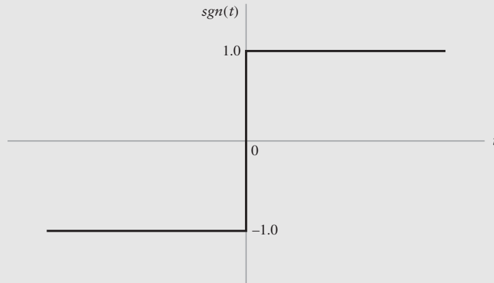
FIGURE 2.7 Signum function.
