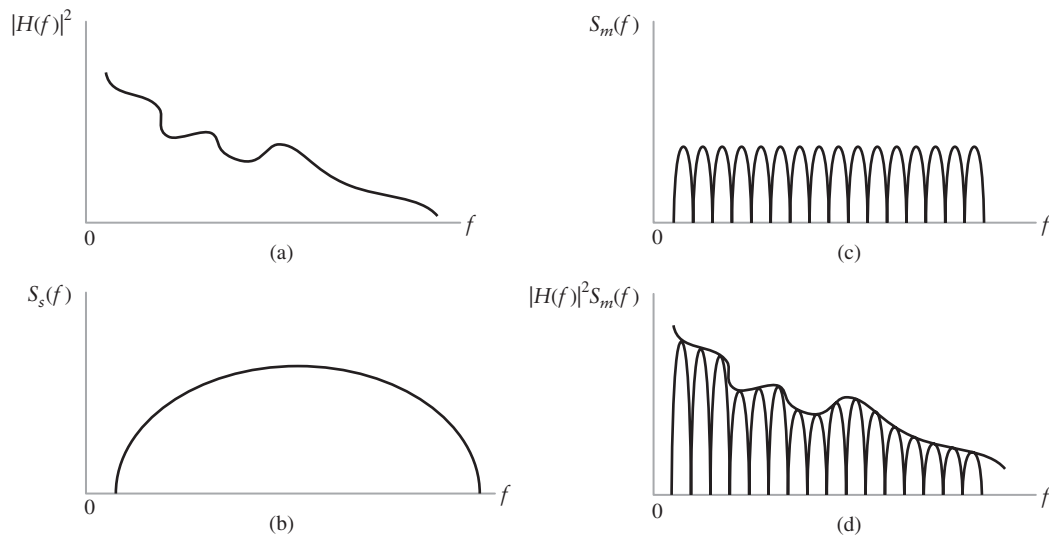
FIGURE 7.25 (a) Frequency response squared of channel. (b) Transmit power spectral density of single-carrier modulation. (c) Transmit power spectral density of multi-carrier modulation. (d) Received power spectral density of multi-carrier modulation.
