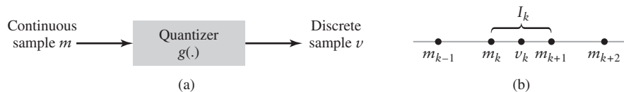
FIGURE 5.9 Description of a memoryless quantizer.
