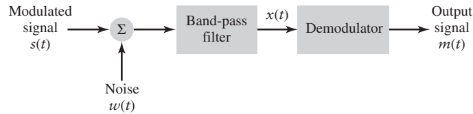
FIGURE 9.3 High-level block diagram of a communications receiver.
