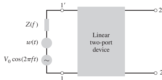
FIGURE 11.4 Linear two-port device.
