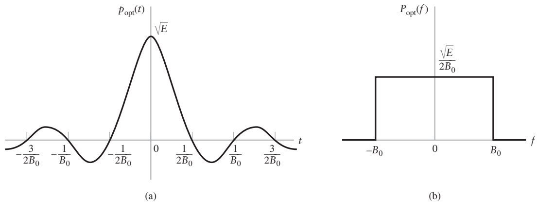
FIGURE 6.2 (a) Sinc function p(t) as the optimum pulse shape. (b) Optimum pulse spectrum.
