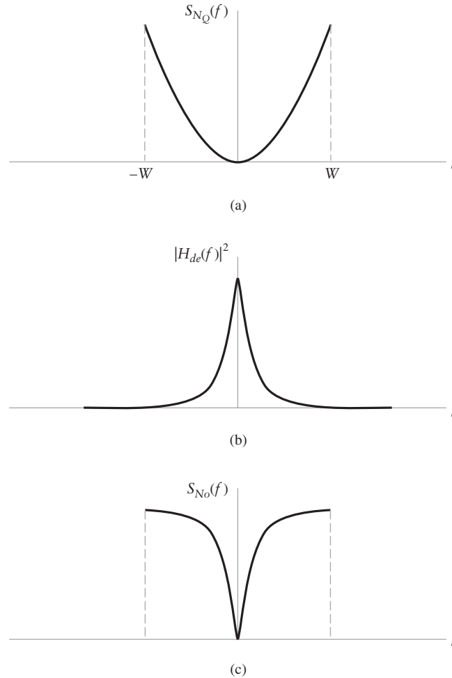
FIGURE 9.18 Use of pre-emphasis and de-emphasis in an FM system. (a) Output noise spectrum before de-emphasis. (b) Frequency response of de-emphasis filter. (c) Noise spectrum after de-emphasis.
