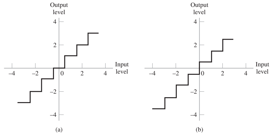
FIGURE 5.10 Two types of quantization: (a) midtread and (b) midrise.
