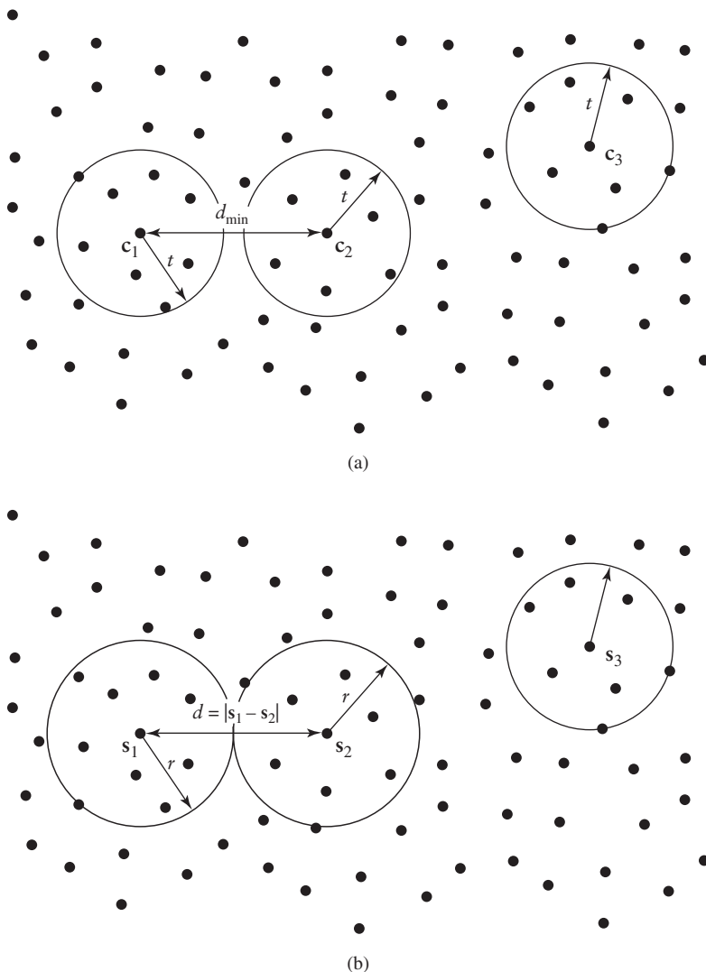
FIGURE 10.20 Illustration of minimum distance in: (a) code word space with t = \lfloor (d_{\min} - 1)/2 \rfloor ; and (b) signal space with d = 2\sqrt{d_{\min}E_b} and r = \sqrt{d_{\min}E_b} .
