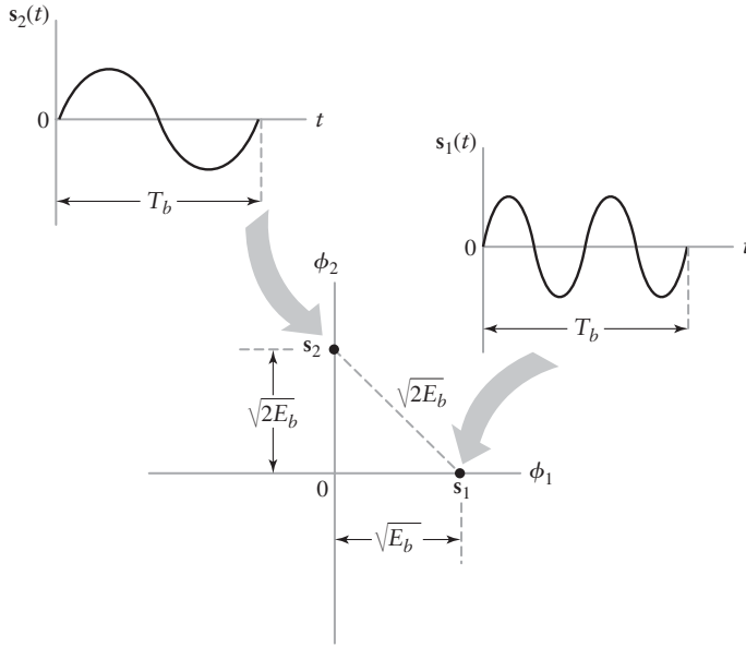
FIGURE 7.24 Mapping of BFSK onto two-dimensional signal-space diagram.
