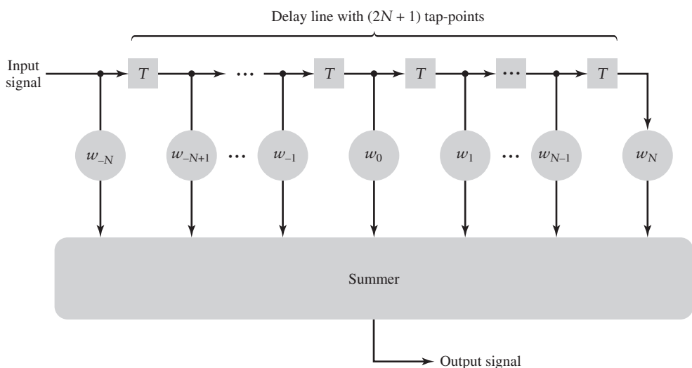
FIGURE 6.10 Transversal filter.
