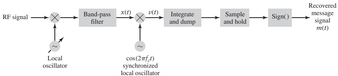
FIGURE 10.7 Typical BPSK receiver structure.
