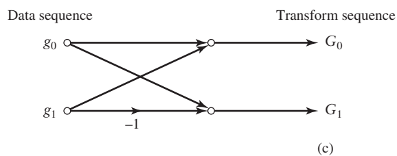
FIGURE 2.35 (a) Reduction of 8-point DFT into two 4-point DFTs. (b) Reduction of 4-point DFT into two 2-point DFTs. (c) Trivial case of 2-point DFT.
