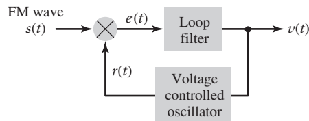
FIGURE 4.14 Block diagram of the phase-locked loop.
