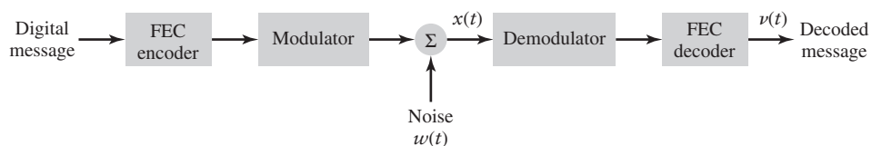
FIGURE 10.18 Block diagram of system including coding and decoding.
