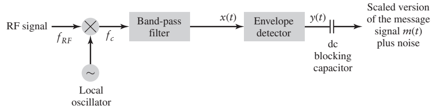
FIGURE 9.8 Model of AM receiver using envelope detection.
