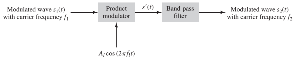
FIGURE 3.21 Block diagram of mixer.
