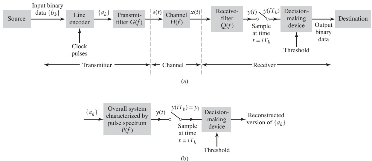
FIGURE 6.1 Baseband binary data transmission. (a) Block diagram of the system, depicting its constituent components all the way from the source to destination. (b) Simplified representation of the system.
