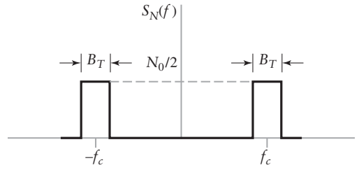
FIGURE 9.7 Power spectral density of band-pass noise.
