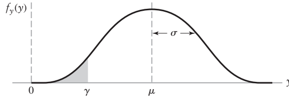
FIGURE 10.4 The Gaussian density function for detecting a 1 with on-off signaling.
