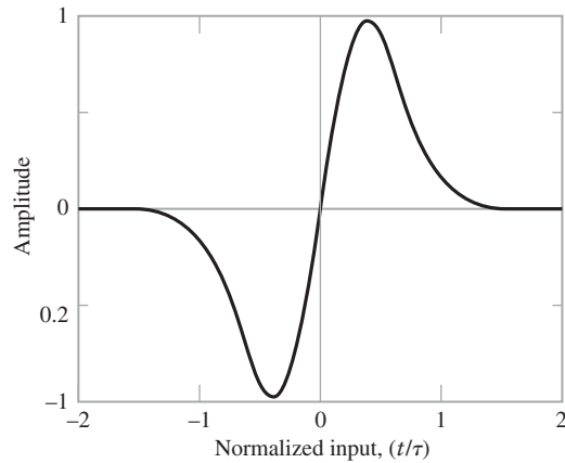
FIGURE 5.22 Time-domain plot of Gaussian monocycle used for impulse radio.
