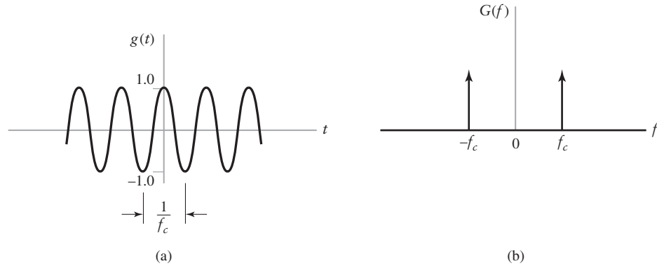
FIGURE 2.15 (a) Cosine function. (b) Spectrum.
