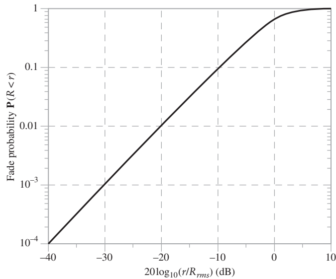
FIGURE 11.11 Normalized Rayleigh amplitude distribution ( r/R_{\text{rms}} ).
