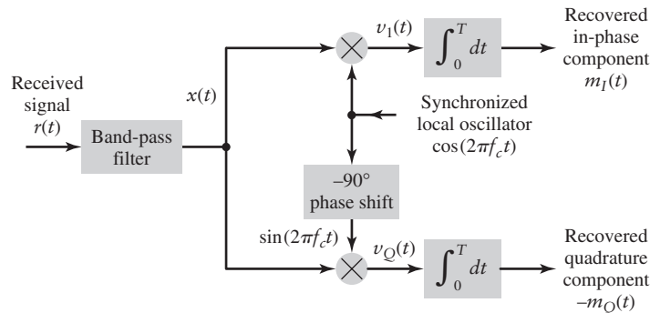
FIGURE 10.8 Quadrature receiver for QPSK.
