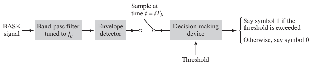
FIGURE 7.17 Noncoherent BASK receiver; the integer i for the sampler equals 0, \pm 1 , \pm 2 , ...
