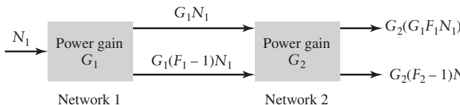
FIGURE 11.6 A cascade of two noisy networks.
