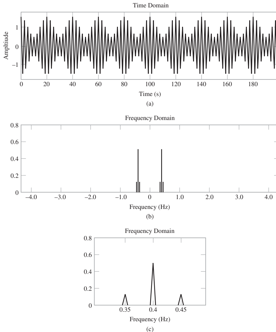
FIGURE 3.5 Amplitude modulation with 50 percent modulation: (a) AM wave, (b) magnitude spectrum of the AM wave, and (c) expanded spectrum around the carrier frequency.
