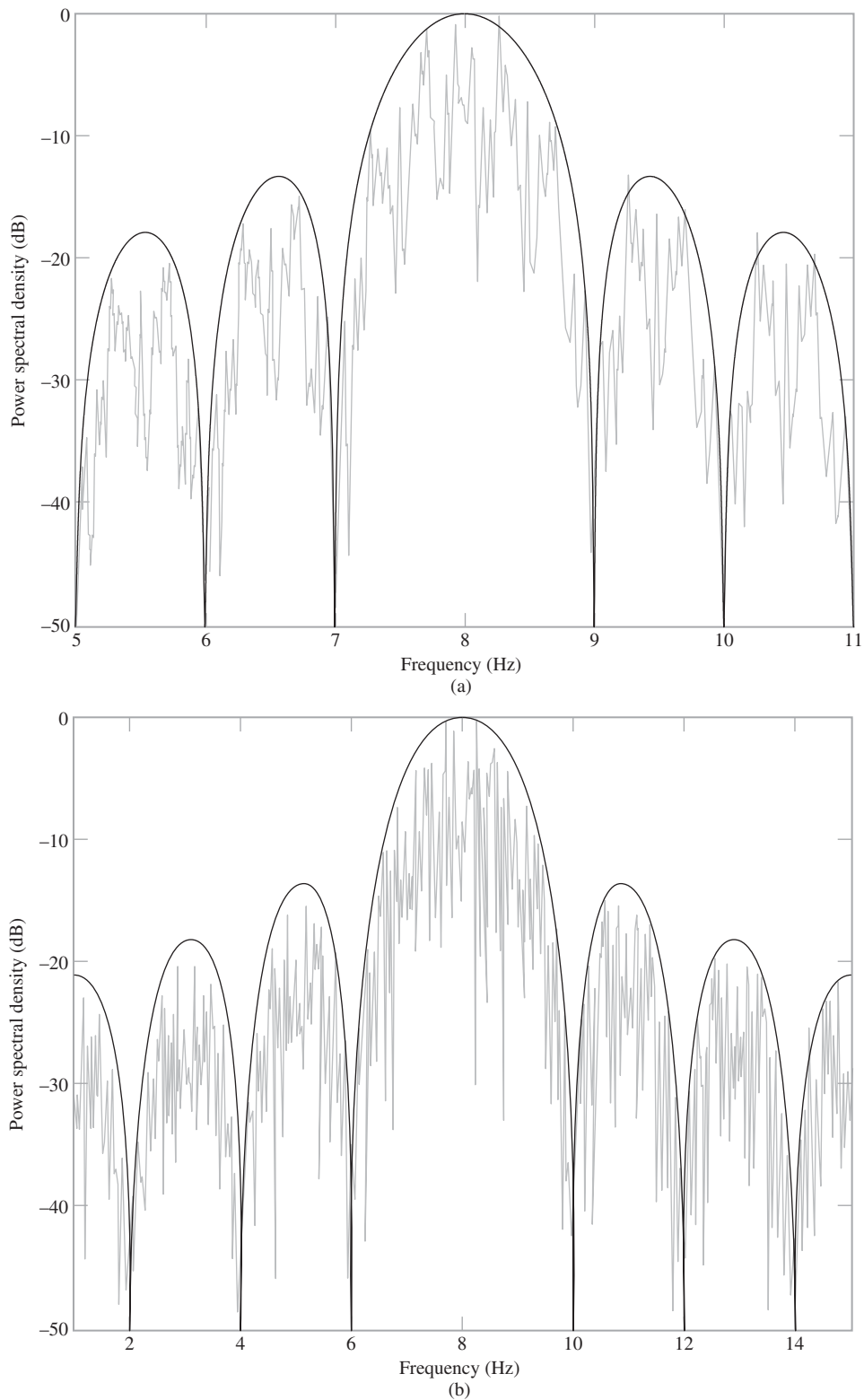
FIGURE 7.6 Power spectra of BPSK signal produced by square wave as the modulating signal for varying bit duration: (a) f_c = 8 Hz and T_b = 1 s; (b) f_c = 8 Hz and T_b = 1/2 s.
