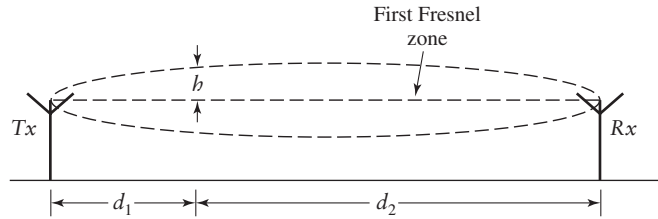
FIGURE 11.8 The first Fresnel zone for free-space propagation.
