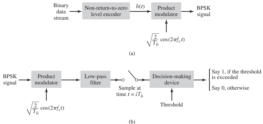
FIGURE 7.4 (a) BPSK modulator. (b) Coherent detector for BPSK; for the sampler, integer i = 0, \pm 1, \pm 2, \dots
