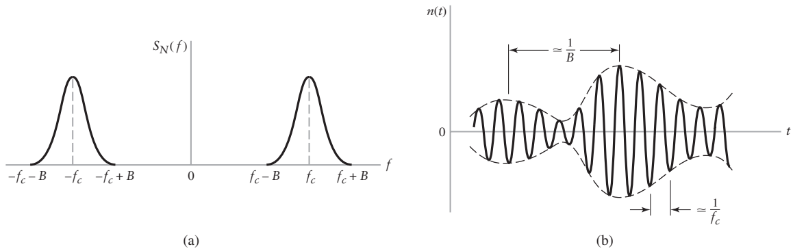
FIGURE 8.21 (a) Power spectral density of narrowband noise. (b) Sample function of narrowband noise.
