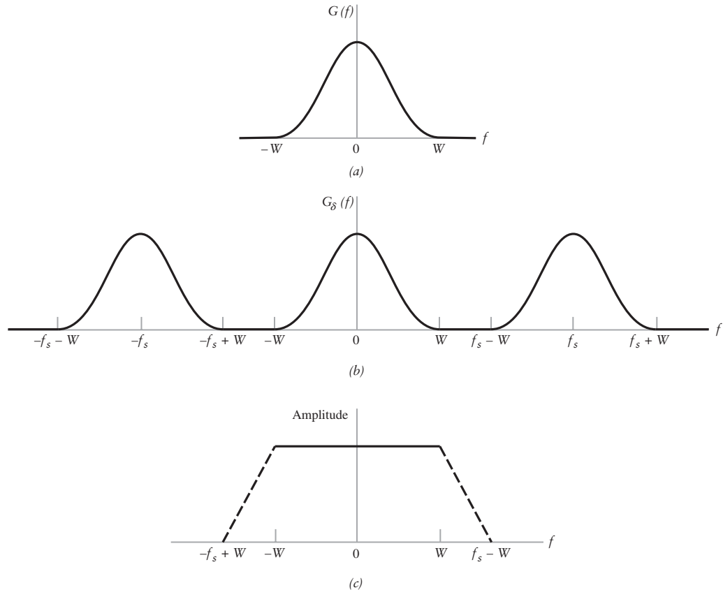
FIGURE 5.4 (a) Anti-alias filtered spectrum of an information-bearing signal. (b) Spectrum of instantaneously sampled version of the signal, assuming the use of a sampling rate greater than the Nyquist rate. (c) Idealized amplitude response of the reconstruction filter.
