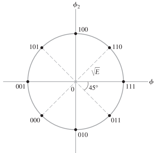
FIGURE 7.20 Signal-space diagram of 8-PSK.
