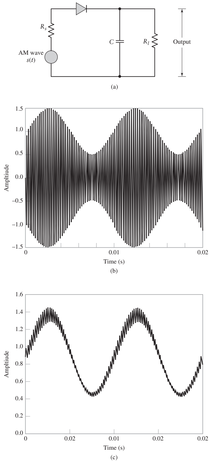
FIGURE 3.9 Envelope detector. (a) Circuit diagram. (b) AM wave input. (c) Envelope detector output
