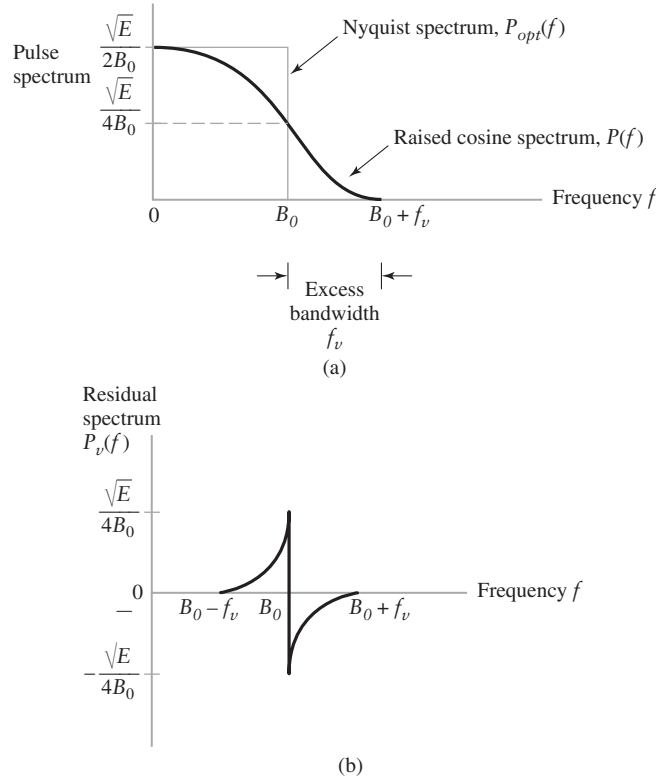
FIGURE 6.4 (a) Nyquist and raised-cosine pulse spectra for positive frequencies. (b) Residual spectrum P_v(f) .
