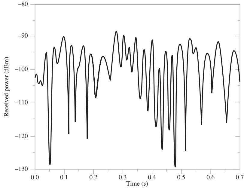
FIGURE 11.10 Illustration of received signal power variations in Rayleigh fading.
