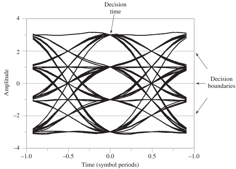
FIGURE 10.9 Eye diagram for four-level PAM.
