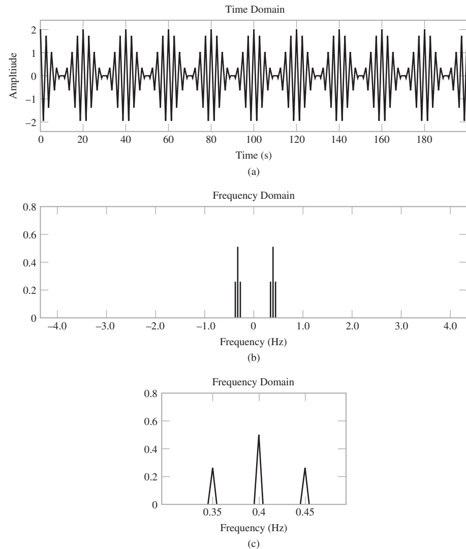
FIGURE 3.6 Amplitude modulation with 100 percent modulation: (a) AM wave, (b) magnitude spectrum of the AM wave, and (c) expanded spectrum around the carrier frequency.
