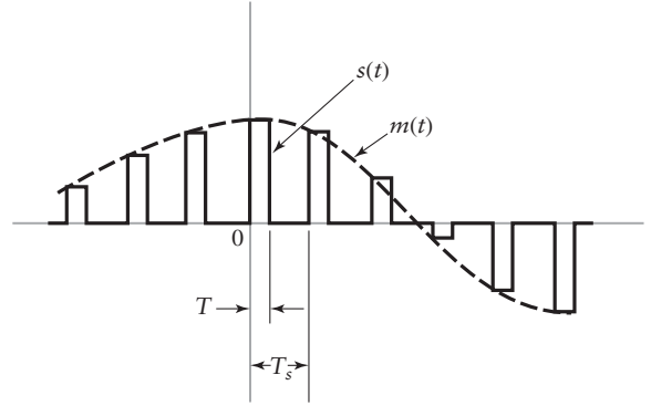
FIGURE 5.5 Flat-top sampling of a message signal.
