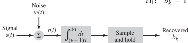
FIGURE 10.3 The integrate-and-dump detector.
