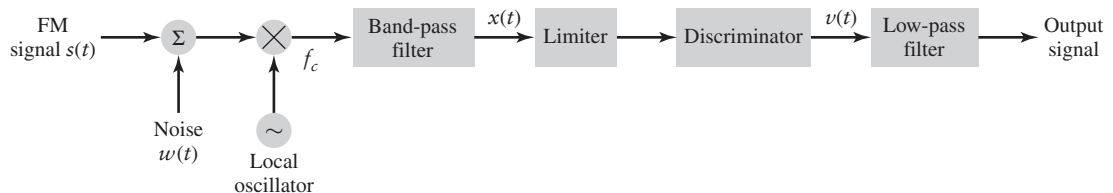
FIGURE 9.13 Model of an FM receiver.
