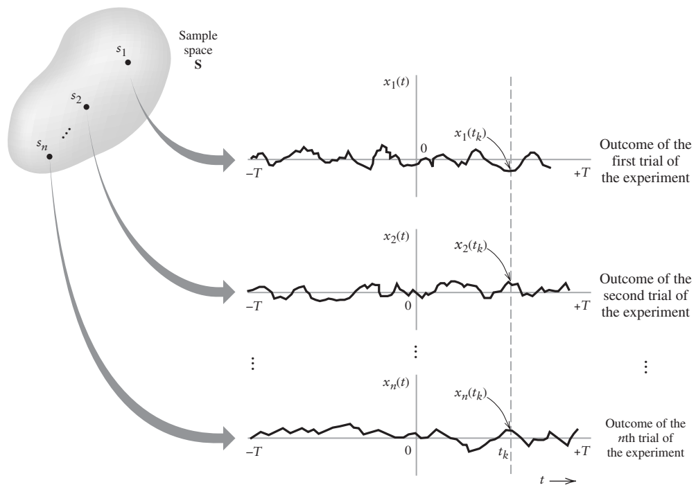
FIGURE 8.14 Illustration of the relationship between sample space and the ensemble of sample functions.
