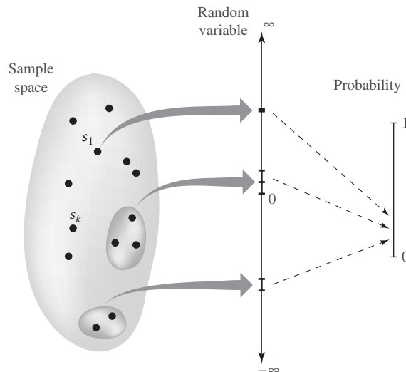
FIGURE 8.3 Illustration of the relationship between sample space, random variables, and probability.
