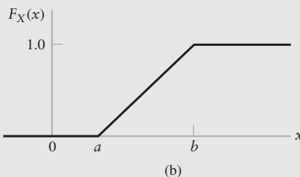
FIGURE 8.5 The uniform distribution. (a) The probability density function. (b) The distribution function.
