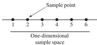
FIGURE 8.1 Sample space of the experiment of throwing a die.
