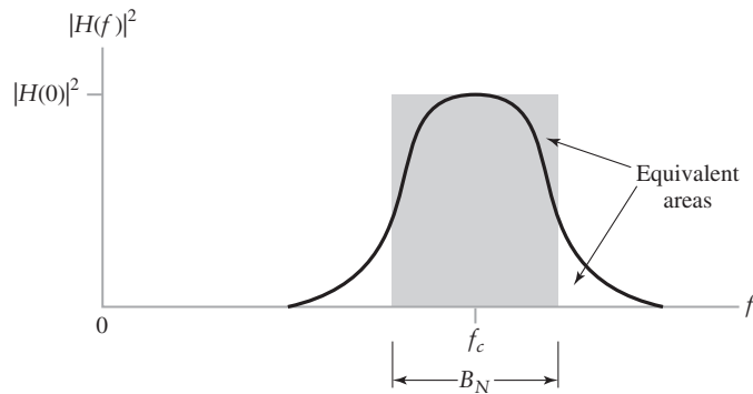
FIGURE 8.25 Illustration of arbitrary bandpass filter H(f) and ideal bandpass filter of bandwidth B_N .
