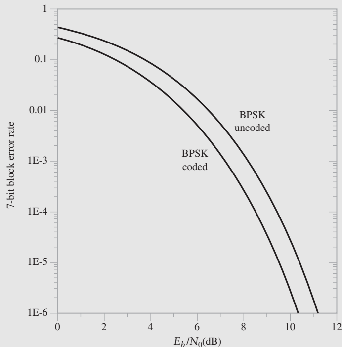
FIGURE 10.19 Comparison of 7-bit block error rate of uncoded BPSK and Hamming (7, 4) coded BPSK.
