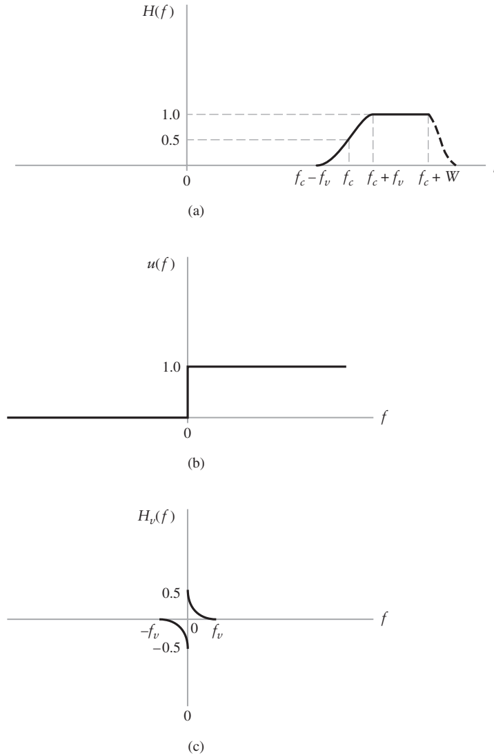
FIGURE 3.24 (a) Amplitude response of sideband-shaping filter; only the positive-frequency portion is shown, the dashed part of the amplitude response is arbitrary. (b) Unit-step function defined in the frequency domain. (c) Low-pass transfer function H_v(f) .
