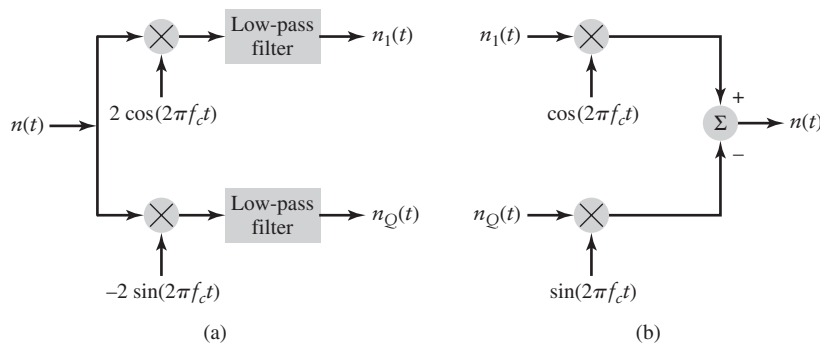
FIGURE 8.22 (a) Extraction of in-phase and quadrature components of narrowband noise process. (b) Generation of narrowband noise process from its in-phase and quadrature components.
