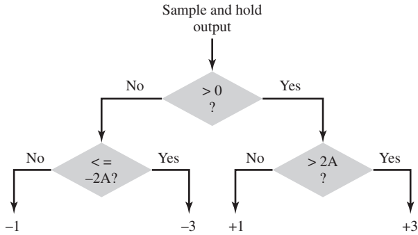
FIGURE 10.11 Illustration of decision rules with four level PAM.
