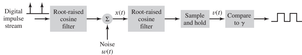
FIGURE 10.6 Implementation of PAM with root-raised cosine filtering. (Root-raised cosine pulse shaping was discussed in Section 6.4.)
