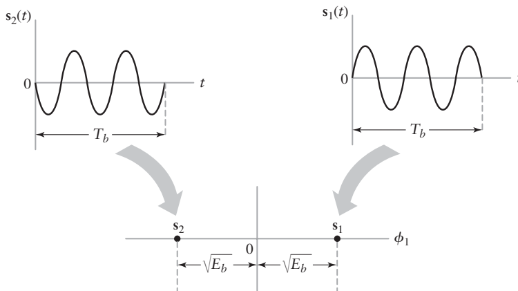
FIGURE 7.23 Mapping of BPSK signal onto a one-dimensional signal-space diagram.
