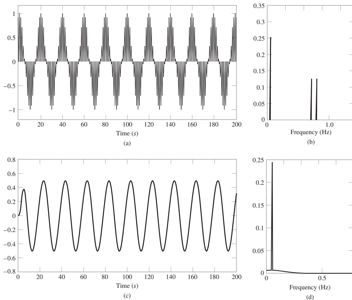
FIGURE 3.15 Coherent detection of DSB-SC modulated wave: (a) Waveform of signal produced at the output of product modulator, (b) amplitude spectrum of the signal in part (a); (c) waveform of low-pass filter output; and (d) amplitude spectrum of signal in part (c).
