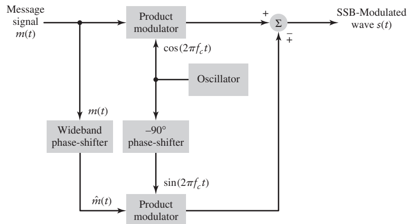
FIGURE 3.20 Phase discrimination method for generating a SSB-modulated wave.
