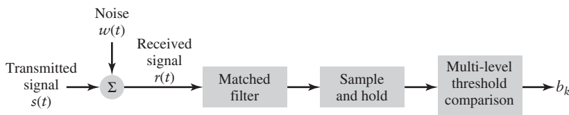
FIGURE 10.10 Multi-level PAM detector.
