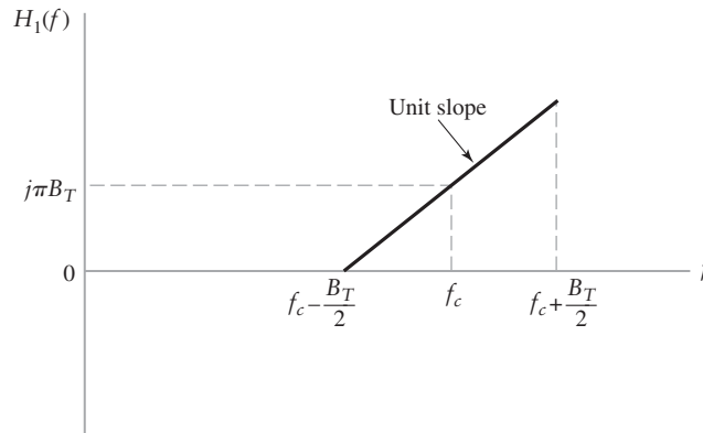
FIGURE 4.12 Frequency response of an ideal slope circuit.
