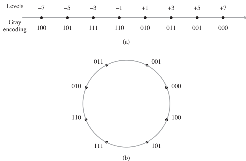
FIGURE 10.15 Gray-encoding of (a) 8-ary PAM and (b) 8-PSK.
