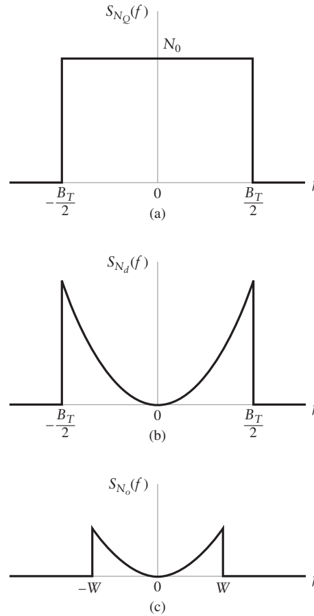
FIGURE 9.16 Noise analysis of FM receiver. (a) Power spectral density of quadrature component n_Q(t) of narrowband noise n(t) . (b) Power spectral density n_d(t) at discriminator output. (c) Power spectral density of noise n_o(t) at receiver output.
