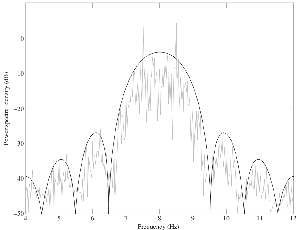
FIGURE 7.12 Power spectrum of Sunde's BFSK produced by square wave as the modulating signal for the following parameters: f_c = 8 \text{ Hz} and T_b = 1 \text{ s} .
