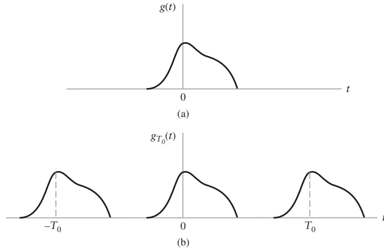
FIGURE A2.3 Illustration of the use of an arbitrarily defined function of time to construct a periodic waveform. (a) Arbitrarily defined function of time g(t) . (b) Periodic waveform g_{T_0}(t) based on g(t) .
