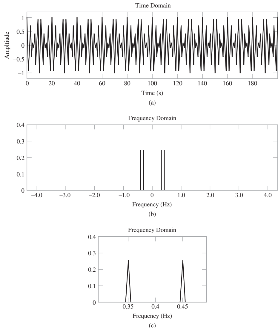
FIGURE 3.14 DSB-SC modulation: (a) DSB-SC modulated wave, (b) magnitude spectrum of the modulated wave, and (c) expanded spectrum around the carrier frequency.
