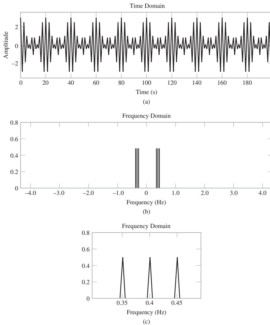
FIGURE 3.7 Amplitude modulation with 200 percent modulation: (a) AM wave, (b) magnitude spectrum of the AM wave, and (c) expanded spectrum around the carrier frequency.
