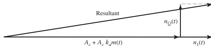
FIGURE 9.11 Phasor diagram for AM wave plus narrowband noise.
