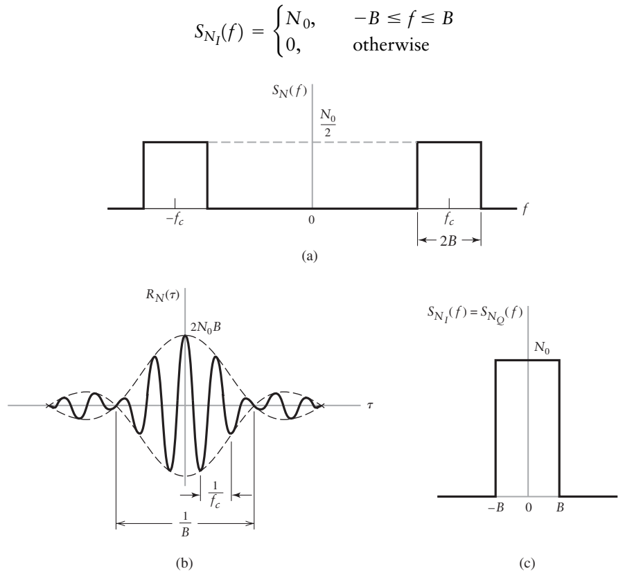
FIGURE 8.23 Characteristics of ideal band-pass filtered white noise. (a) Power spectral density. (b) Autocorrelation function. (c) Power spectral density of in-phase and quadrature components.
