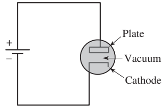
FIGURE 11.2 A temperature-limited vacuum diode.
