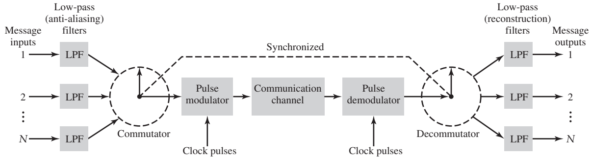
FIGURE 5.21 Block diagram of TDM system.
