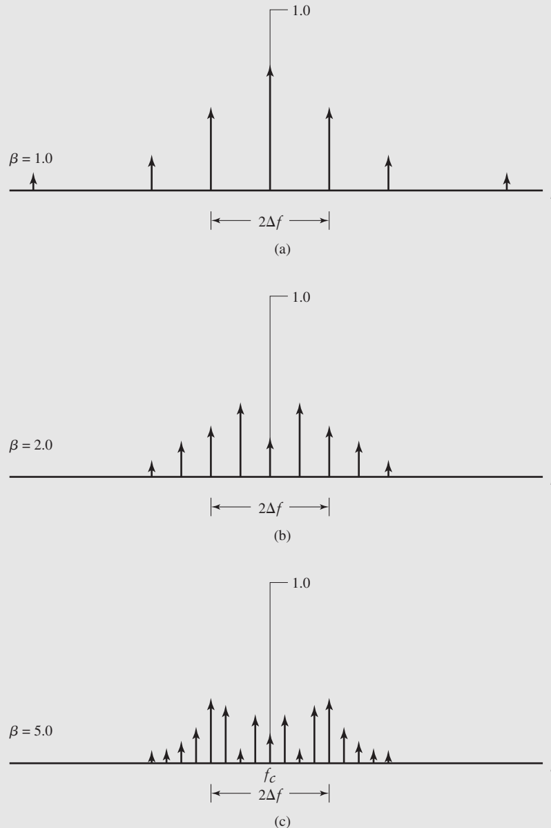
FIGURE 4.8 Discrete amplitude spectra of an FM wave, normalized with respect to the unmodulated carrier amplitude, for the case of sinusoidal modulation of varying frequency and fixed amplitude. Only the spectra for positive frequencies are shown.
