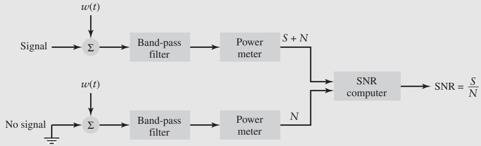
FIGURE 9.2 SNR measurement scheme for Example 9.1.
