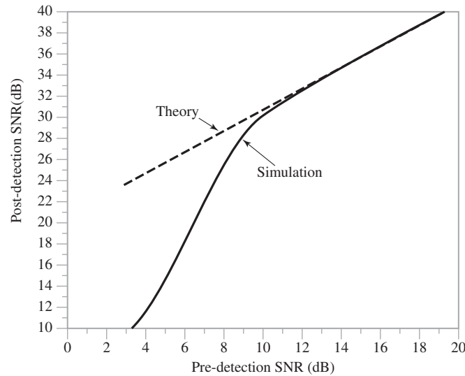
FIGURE 9.17 Comparison of pre-detection and post-detection SNRs for a simulated FM receiver. ( f_m = 1 Hz, k_f = 20 Hz, B_T = 62.5 Hz, W = 5.5 Hz, A_c = 1 )
