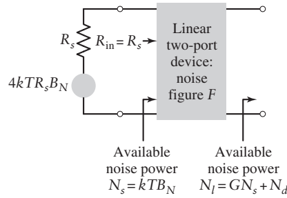
FIGURE 11.5 Linear two-port device matched to the internal resistance of a source connected to the input.
