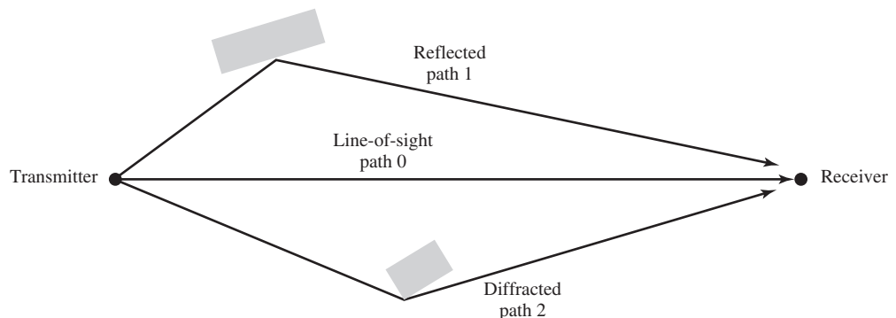
FIGURE 11.9 Illustration of multiple transmission paths between transmitter and receiver.
