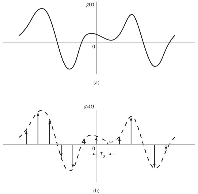
FIGURE 5.1 Illustration of the sampling process. (a) Analog waveform g(t) . (b) Instantaneously sampled representation of g(t) .
