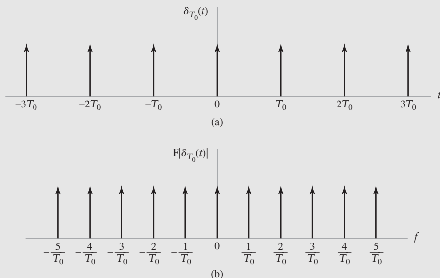
FIGURE 2.19 (a) Dirac comb. (b) Spectrum.
