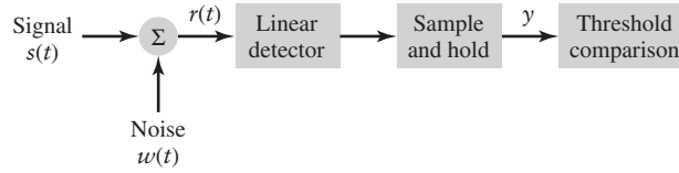
FIGURE 10.1 Processing of a single pulse.
