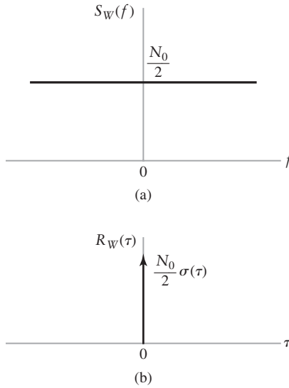
FIGURE 8.18 Characteristics of white noise. (a) Power spectral density. (b) Autocorrelation function.
