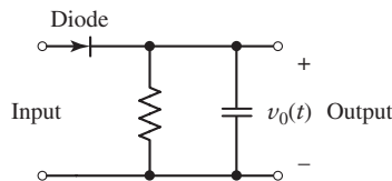
FIGURE 9.9 Circuit diagram of envelope detector.
