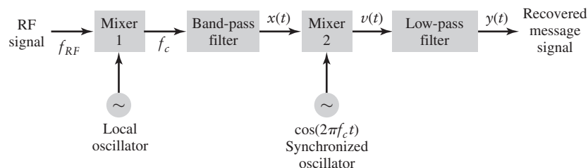
FIGURE 9.6 A linear DSB-SC receiver using coherent demodulation.
