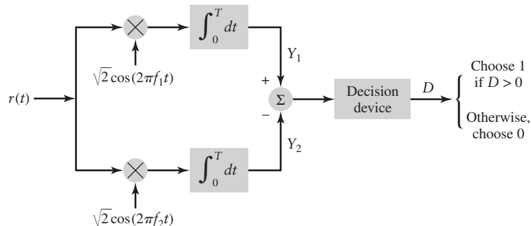
FIGURE 10.12 Coherent detection of binary FSK.
