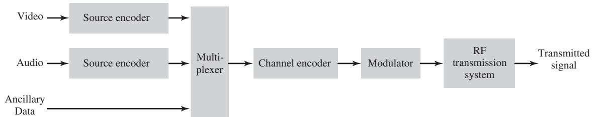
FIGURE 7.27 Digital television broadcasting model.
