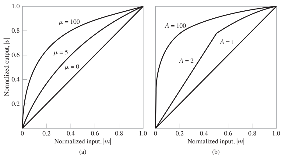
FIGURE 5.12 Compression laws. (a) \mu -law. (b) A-law .
