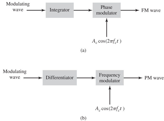
FIGURE 4.3 Illustration of the relationship between frequency modulation and phase modulation. (a) Scheme for generating an FM wave by using a phase modulator. (b) Scheme for generating a PM wave by using a frequency modulator.
