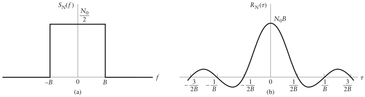
FIGURE 8.19 Characteristics of low-pass filtered white noise. (a) Power spectral density. (b) Autocorrelation function.
