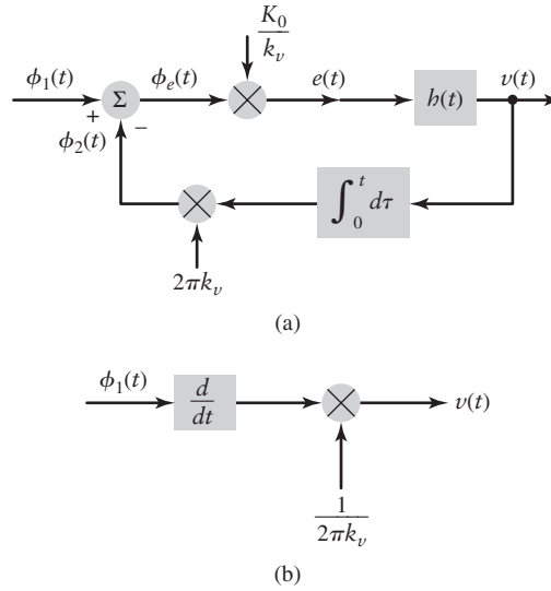
FIGURE 4.15 (a) Linearized model of the phase-locked loop. (b) Approximate form of the model, assuming that the loop gain K_0 is large compared with unity.
