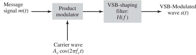
FIGURE 3.23 VSB modulator using frequency discrimination.
