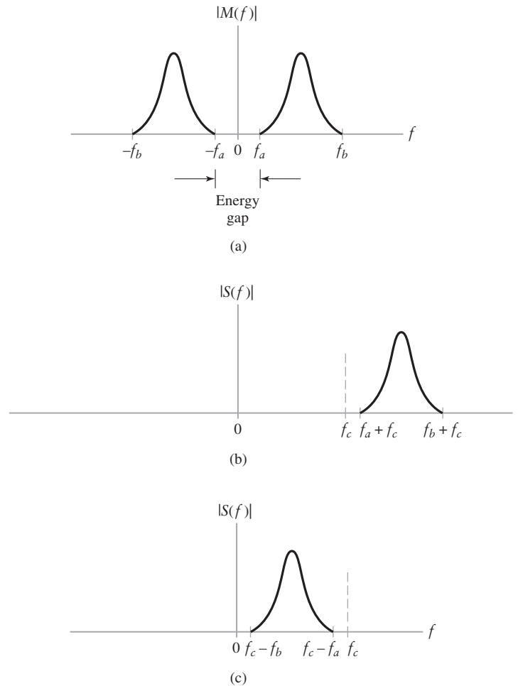
FIGURE 3.18 (a) Spectrum of a message signal m(t) with energy gap centered around zero frequency. Corresponding spectra of SSB-modulated waves using (b) upper sideband, and (c) lower sideband. In parts (b) and (c), the spectra are only shown for positive frequencies.
