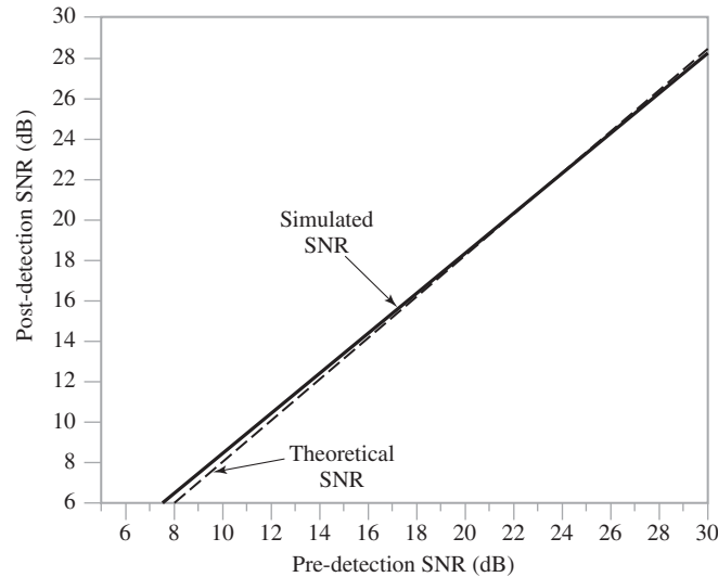
FIGURE 9.12 Comparison of pre-detection and post-detection SNRs with simulated envelope detection of AM.
