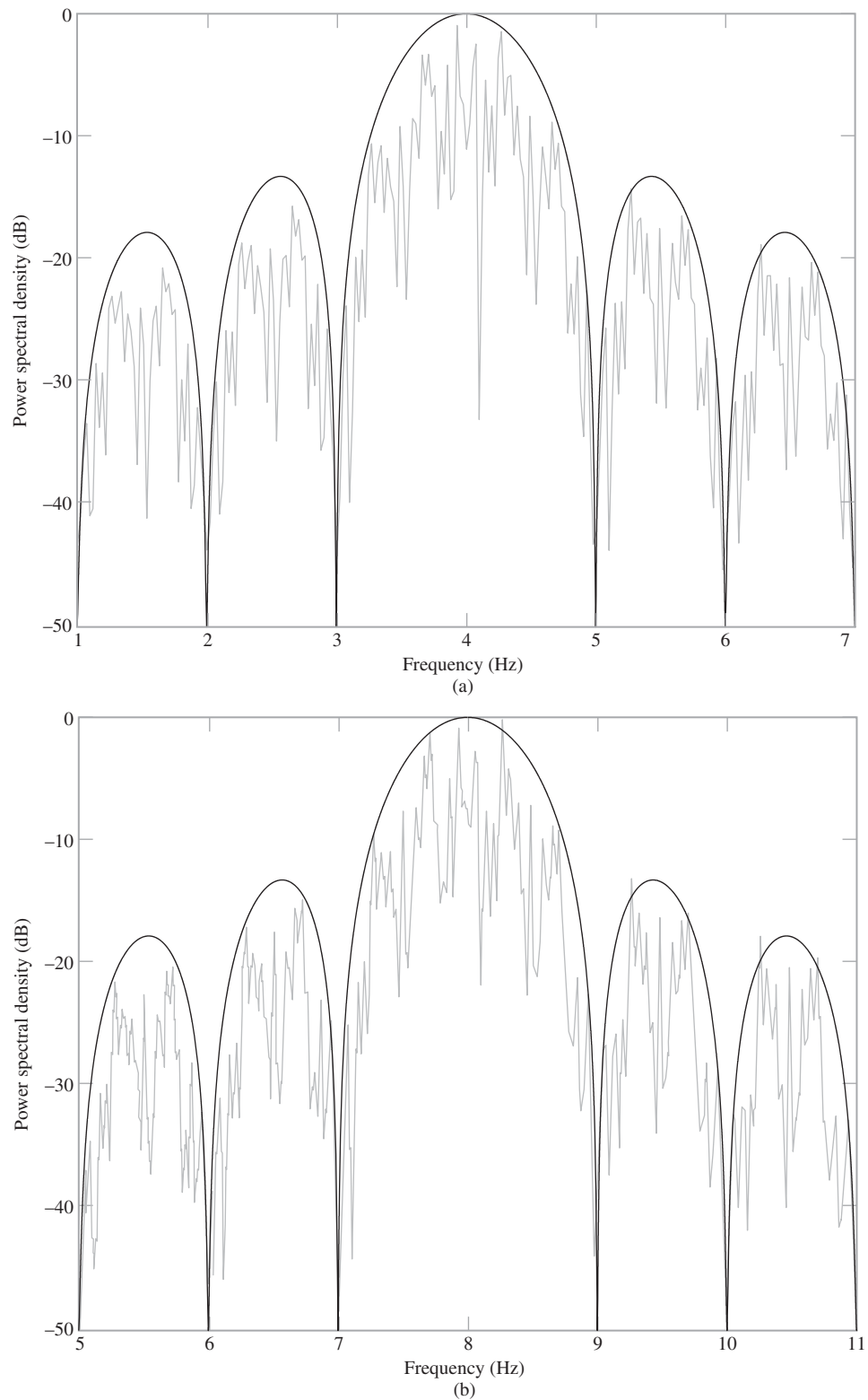
FIGURE 7.5 Power spectra of BPSK signal produced by square wave as the modulating signal for varying modulation frequency: (a) f_c = 4 Hz and T_b = 1 s; (b) f_c = 8 Hz and T_b = 1 s.
