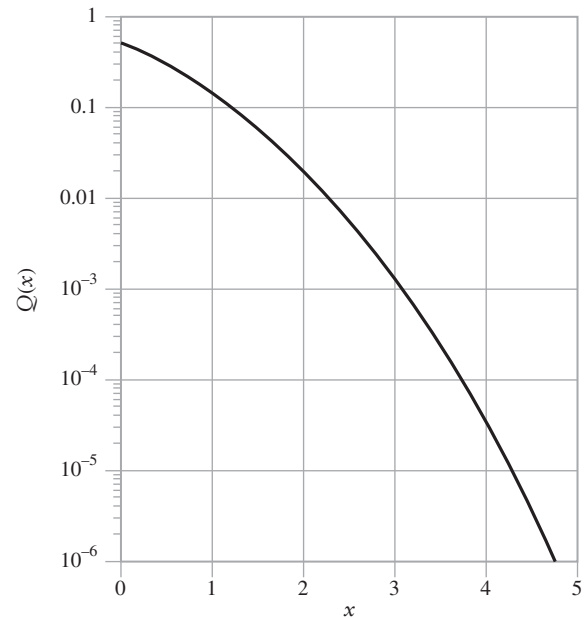
FIGURE 8.11 The Q -function.
