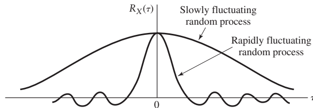
FIGURE 8.15 Illustration of autocorrelation functions of slowly and rapidly fluctuating random processes.
