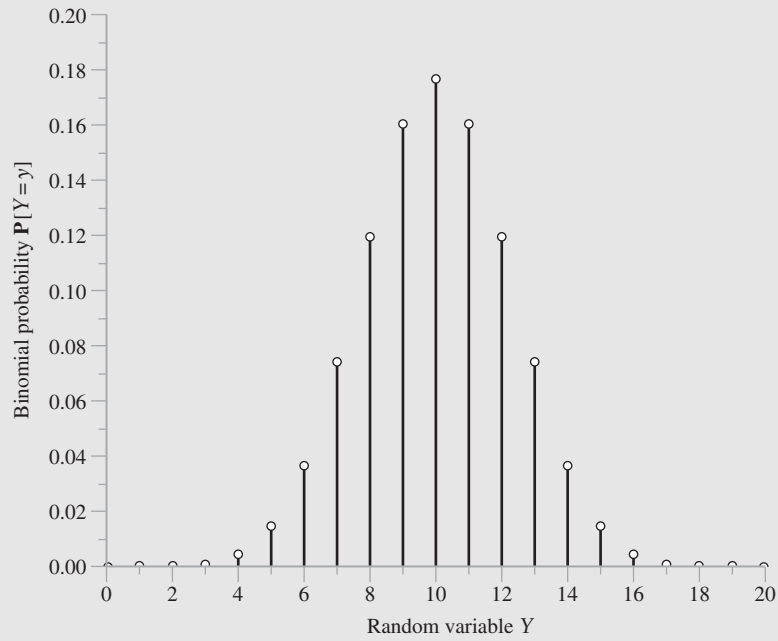
FIGURE 8.6 The binomial probability mass function for N = 20 and p = \frac{1}{2} .
