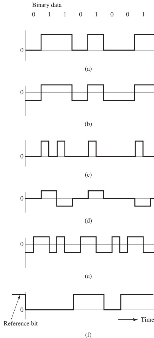
FIGURE 5.20 Line codes. (a) On-off signaling. (b) Nonreturn-to-zero signaling. (c) Return-to-zero signaling. (d) Bipolar return-to-zero signaling. (e) Split-phase or Manchester encoding. (f) Differential encoding.
