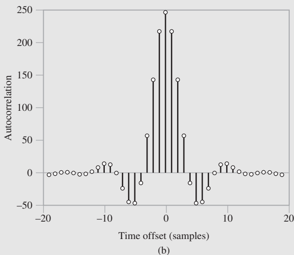
FIGURE 8.16 Illustration of (a) a random signal, and (b) its autocorrelation.
