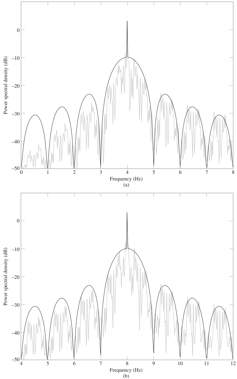
FIGURE 7.2 Power spectra of BASK signal produced by square wave as the modulating signal for varying modulation frequency: (a) f_c = 4 Hz and T_b = 1 s; (b) f_c = 8 Hz and T_b = 1 s.
