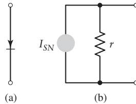
FIGURE 11.3 (a) Junction diode. (b) Shot noise model.
