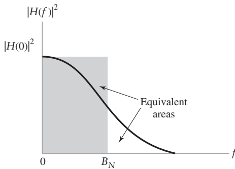
FIGURE 8.24 Illustration of arbitrary low-pass filter H(f) and ideal low-pass filter of bandwidth B_N .
