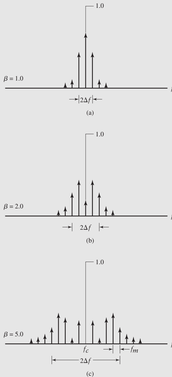
FIGURE 4.7 Discrete amplitude spectra of an FM wave, normalized with respect to the unmodulated carrier amplitude, for the case of sinusoidal modulation of fixed frequency and varying amplitude. Only the spectra for positive frequencies are shown.
