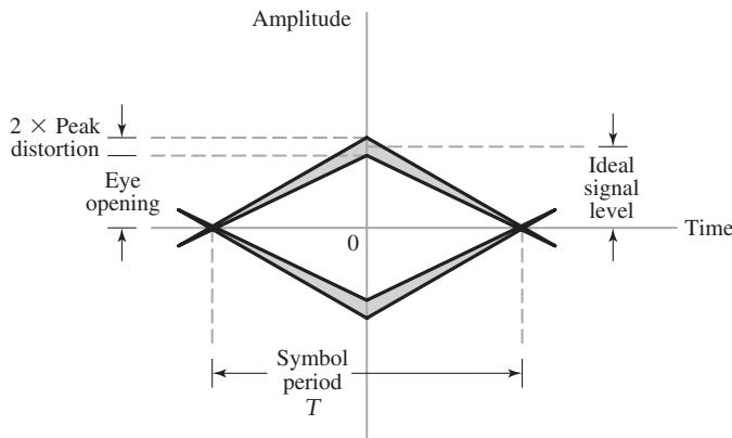
FIGURE 6.7 Illustrating the relationship between peak distortion and eye opening. Note: The ideal signal level is scaled to lie inside the range -1 to +1 .
