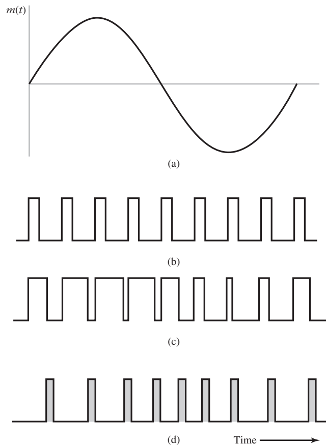
FIGURE 5.8 Illustration of two different forms of pulse-time modulation for the case of a sinusoidal modulating wave. (a) Modulating wave. (b) Pulse carrier. (c) PDM wave. (d) PPM wave.
