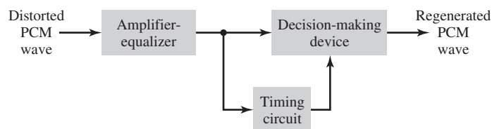
FIGURE 5.13 Block diagram of a regenerative repeater.
