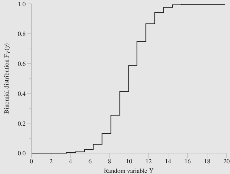
FIGURE 8.7 The binomial distribution function for N = 20 and p = \frac{1}{2} .
