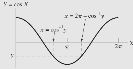
FIGURE 8.9 Illustration of cosine transformation.
