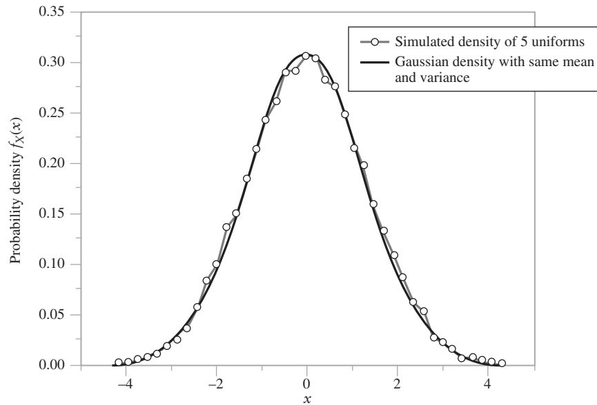
FIGURE 8.13 Comparison of the empirical density of sum of five uniform variables with a Gaussian density having the same mean and variance.
