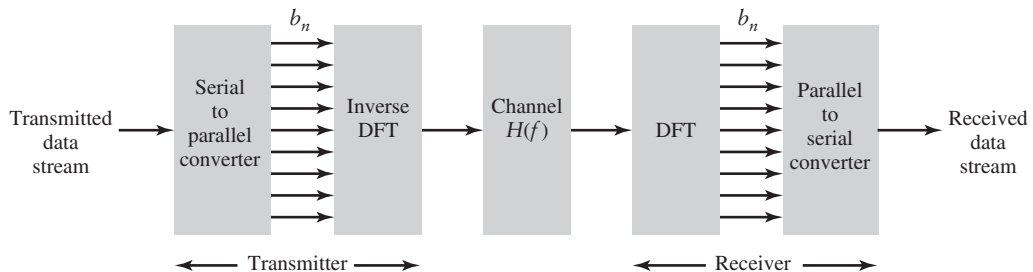
FIGURE 7.26 Block diagram of OFDM system.
