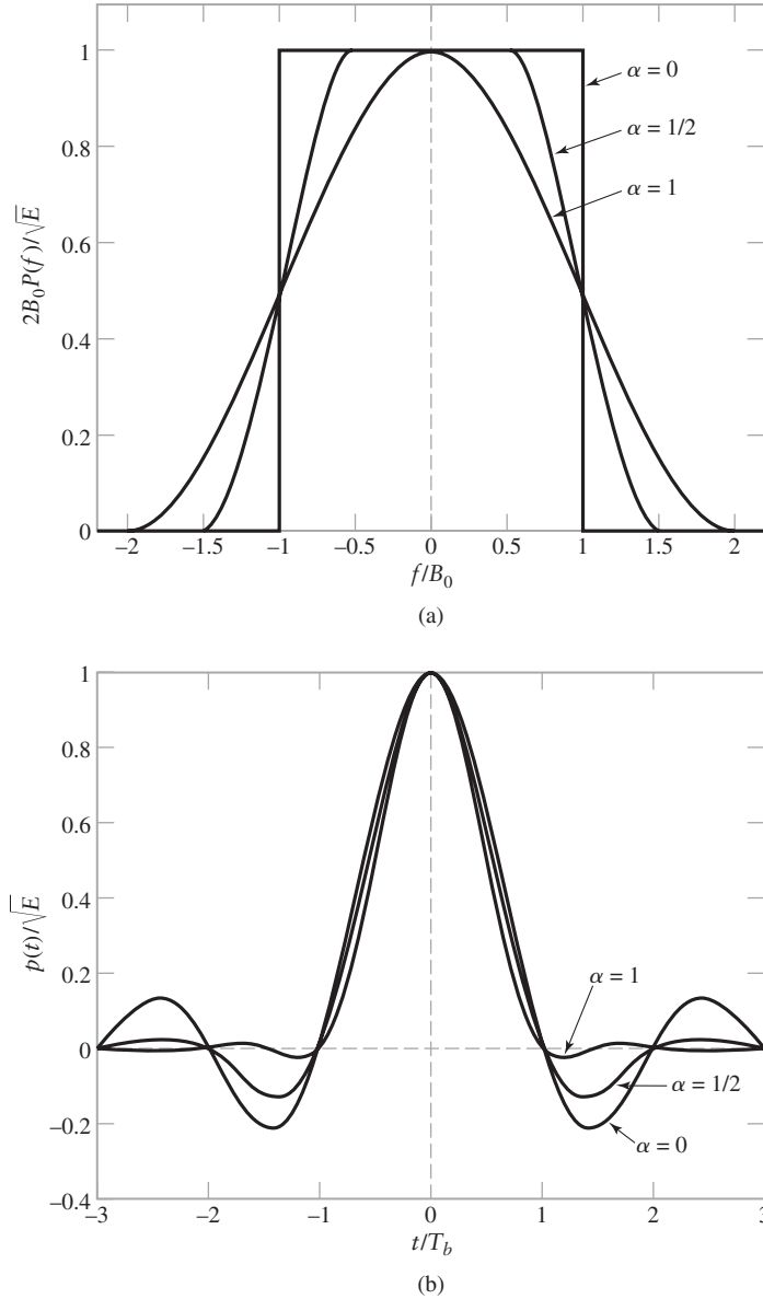
FIGURE 6.3 (a) Raised-cosine pulse spectrum for varying roll-off rates. (b) Pulse response p(t) (i.e., inverse Fourier transform of P(f) for varying roll-off rates).
