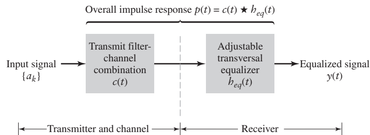
FIGURE 6.11 Simplified depiction of the scenario for solving the channel-equalization problem.
