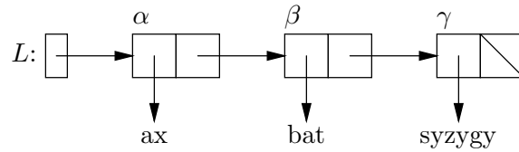
(a) Original list
