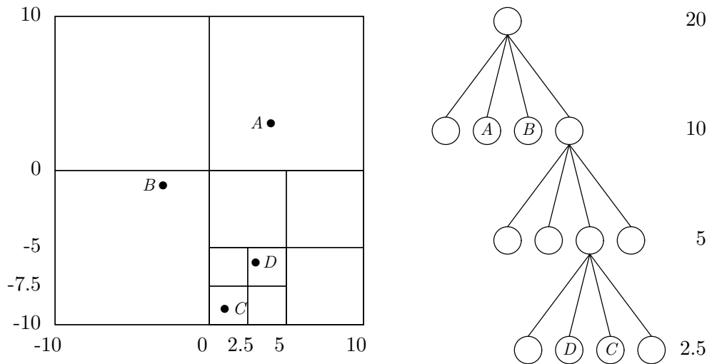
Figure 6.9: Illustration of a four-level quad tree, using square regions for simplicity. The left diagram shows the geometry; the dots represent the positions—the keys—of four data items at (4, 3) , (-3, -1) , (1, -9) , and (3, -6) . On the right, we see the corresponding tree data structure. Each level of the tree contains nodes that represent squares with the same size of edge (shown at the right). The four children of each node represent the upper-left, upper-right, lower-left, and lower-right quadrants of their common parent node, respectively. From the coordinates of the center the square represented by any node, and that node's edge length, you can compute the coordinates of the centers of each child. Hence, from the center the center of the topmost parent— (0, 0) —and its edge length—20 units—you can calculate the regions corresponding to any node in the tree.
