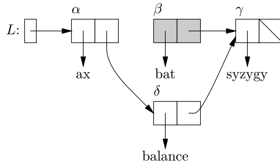
(c) After adding balance with L.\text{next} = \text{new Entry("balance", L.next)}
