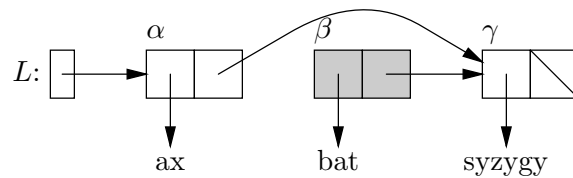
(b) After removing bat with L.\text{next} = L.\text{next}.\text{next}
