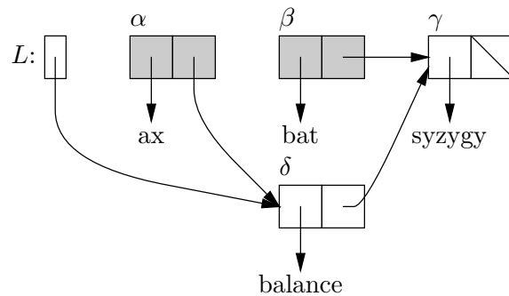
(d) After deleting ax with L = L.\text{next}
