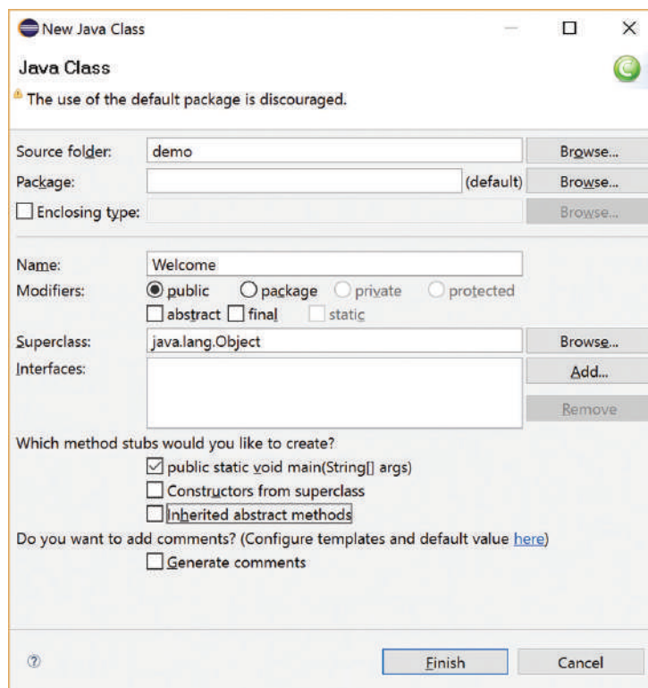
FIGURE 1.19 The New Java Class dialog box is used to create a new Java class. Source:
