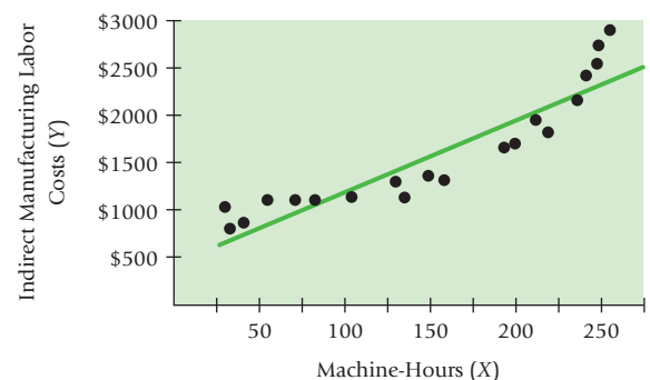
PANEL B: Serial Correlation in Residuals (A Pattern of Positive Residuals for Extreme Machine-Hours Used; Negative Residuals for Moderate Machine-Hours Used)
