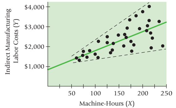
PANEL B: Nonconstant Variance (Higher Outputs Have Larger Residuals)
