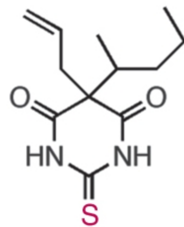
Thiopentobarbital
