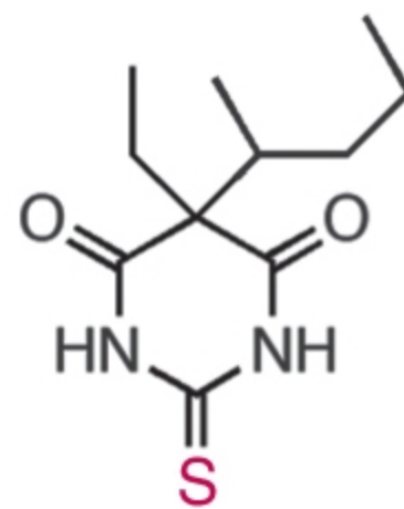
Thiopentobarbital
