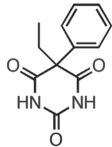
Phenobarbital
