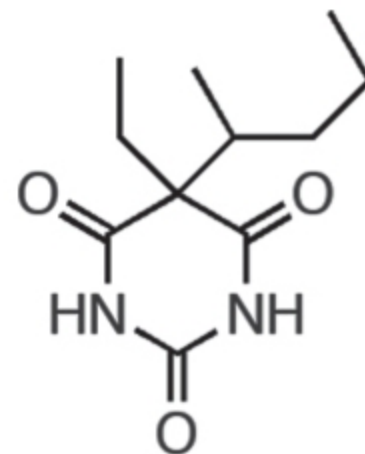
Pentobarbital
