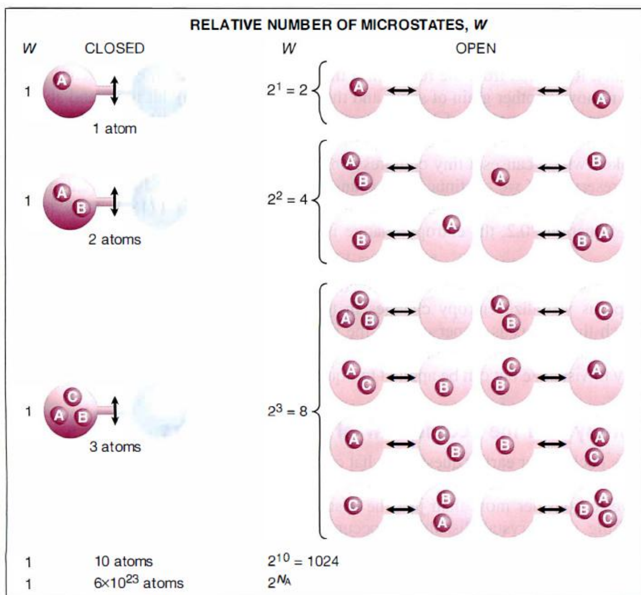
Figure 20.2 Expansion of a gas and the increase in number of microstates. When a gas confined to one flask is allowed to spread through two flasks, the energy of the particles is dispersed over more microstates, and so the entropy is higher. Each combination of particles in the available volume represents a different microstate. The increase in the number of possible microstates that occurs when the volume increases is given by 2^n , where n is the number of particles.
