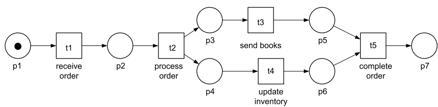
Fig. 4.26. Sample Petri net representing single process instance
