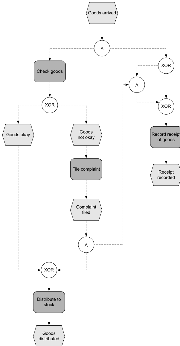
Fig. 6.16. Typical example of an event-driven process chain
