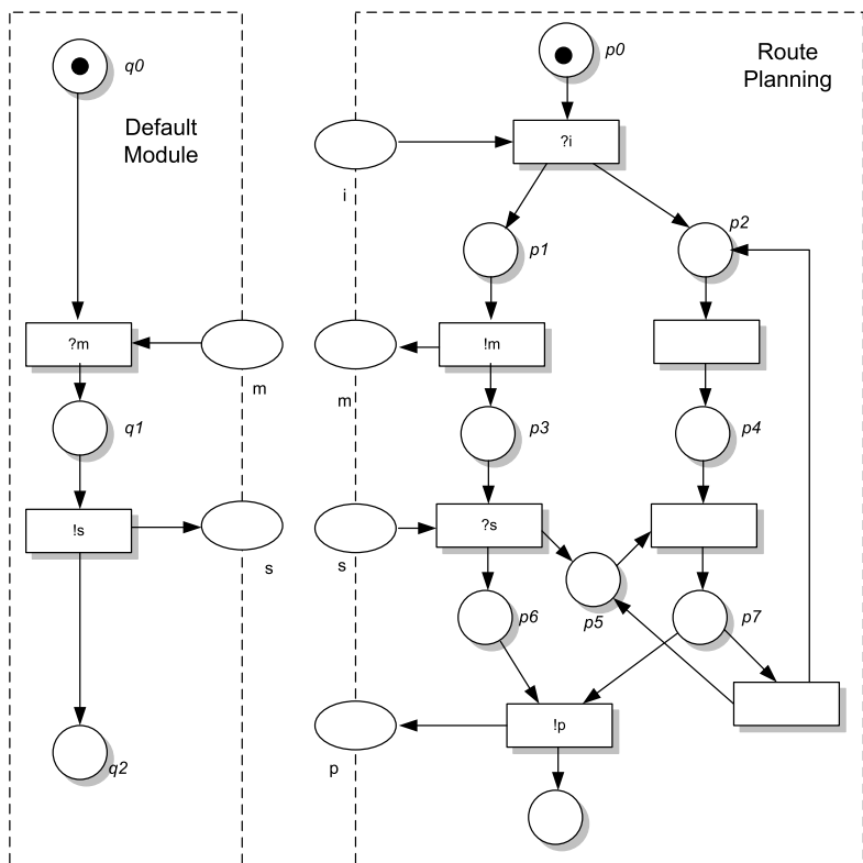
Fig. 6.20. Workflow module with syntactically compatible default module
