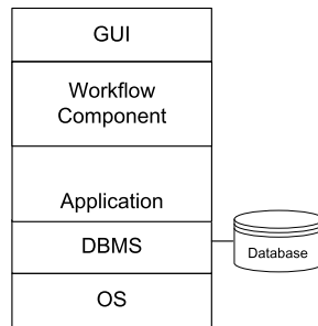
Fig. 2.17. Single-application workflow systems architecture
