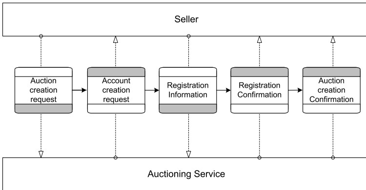
Fig. 5.41. Choreography diagram with pools
