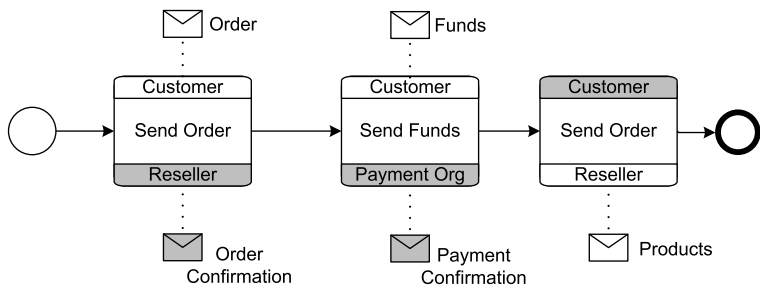
Fig. 5.42. Choreography diagram that is not enforceable, since the reseller cannot know if the customer has already sent the funds
