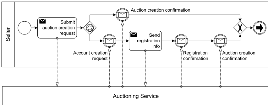
Fig. 5.9. Behavioural interface for seller
