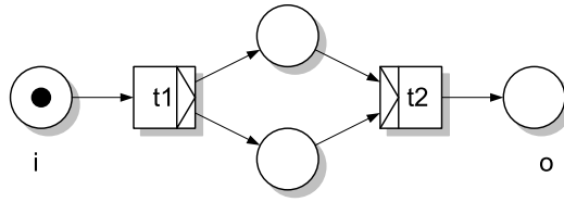
Fig. 6.7. Workflow net with deadlock
