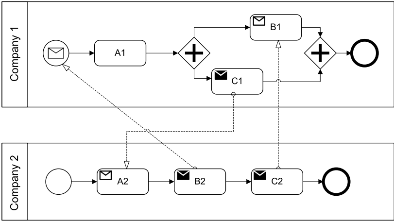
Fig. 5.1. Deadlock of interacting process orchestrations
