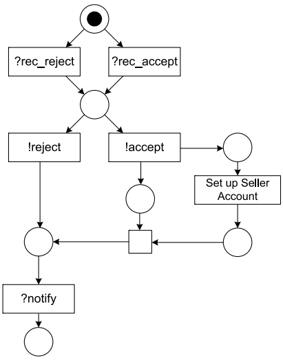
Fig. 5.20. Concur transformation operation of the public-to-private approach
