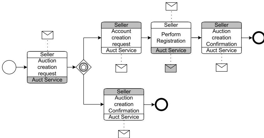
Fig. 5.51. Choreography diagram representing auctioning scenario
