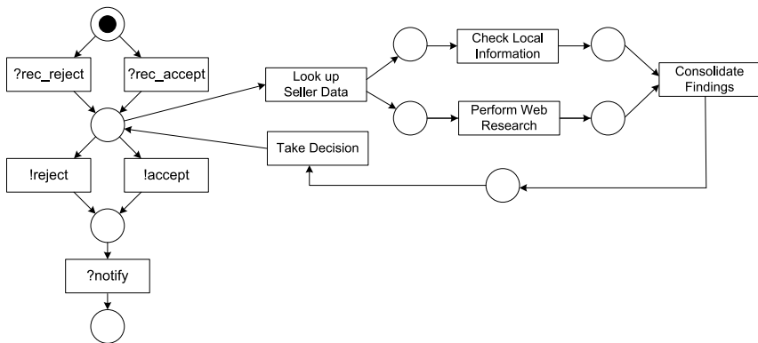
Fig. 5.18. Loop transformation operation of the public-to-private approach
