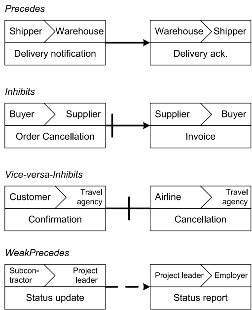
Fig. 5.32. Basic control flow structures relating interactions
