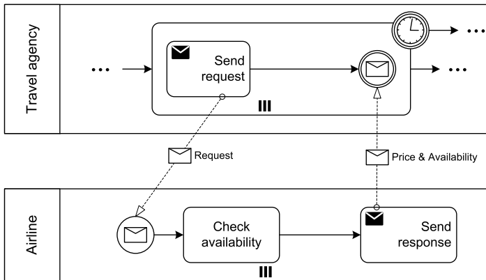
Fig. 5.28. One-to-many send/receive pattern
