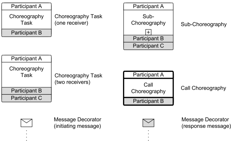
Fig. 5.38. Notational elements used in BPMN Choreography diagrams
