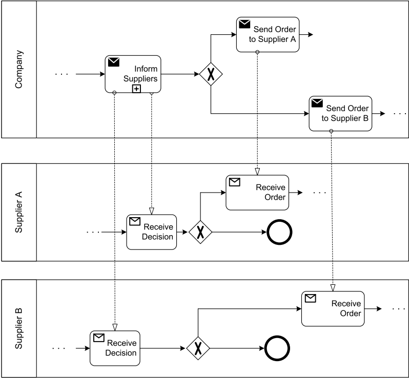
Fig. 5.46. Collaboration diagram with process orchestrations, implementing the choreography defined in Figure 5.45
