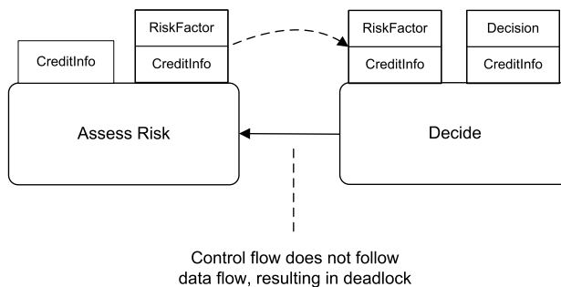
Fig. 6.2. Data flow violated by control flow, resulting in deadlock
