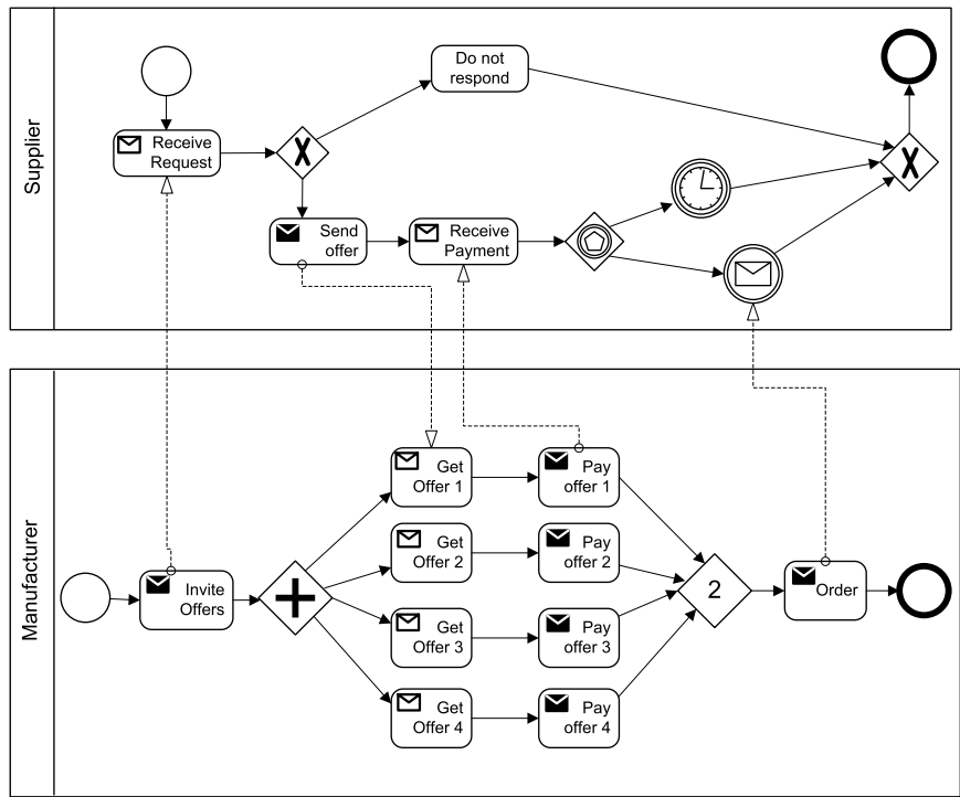
Fig. 6.26. Ordering process with N-out-of-M join
