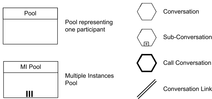
Fig. 5.36. Elements used in BPMN conversation diagrams
