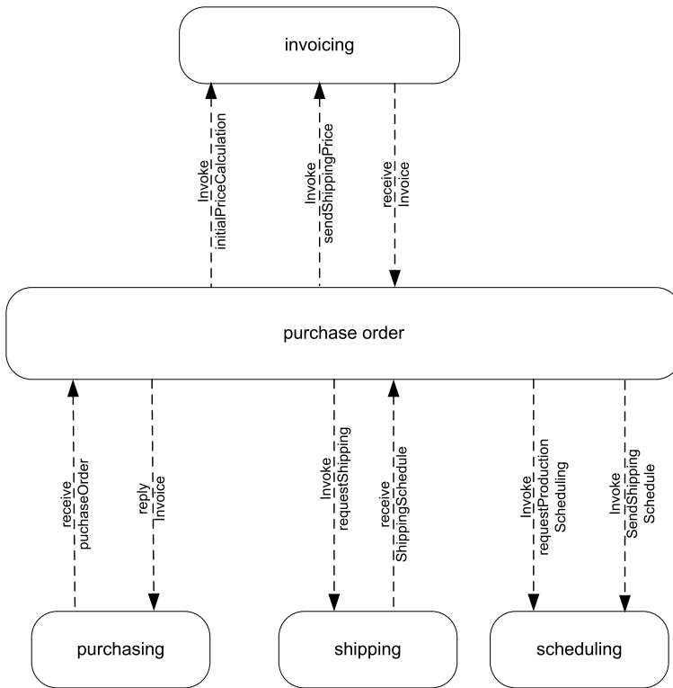
Fig. 7.12. Communication behaviour of purchase order WS-BPEL process
