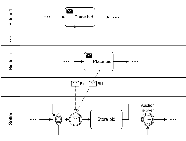
Fig. 5.27. One-from-many receive pattern
