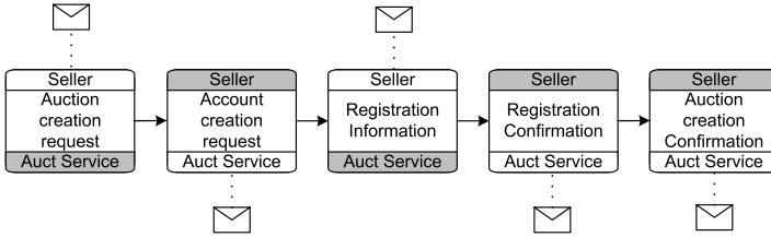
Fig. 5.40. Collaboration scenario, described by BPMN Choreography Diagrams
