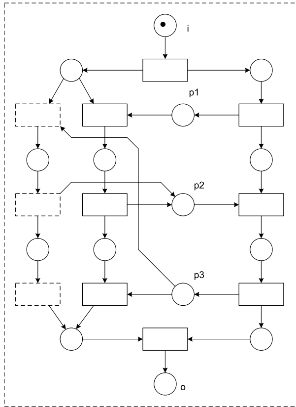
Fig. 6.24. Example of weak sound workflow net
