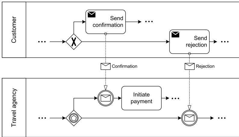
Fig. 5.25. Racing incoming messages pattern
