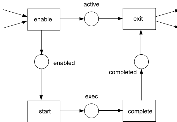
Fig. 4.57. State transition diagram for YAWL tasks with static number of instances
