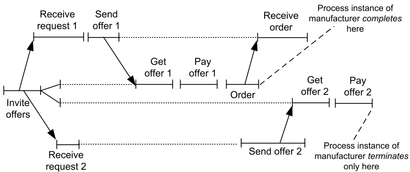
Fig. 6.28. Process instance, illustrating lazy soundness
