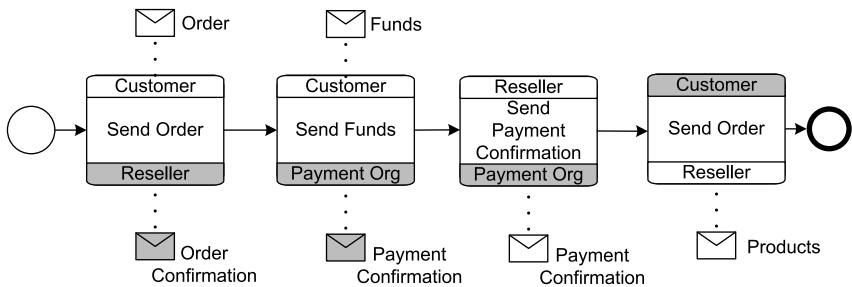
Fig. 5.43. Choreography diagram that is enforceable
