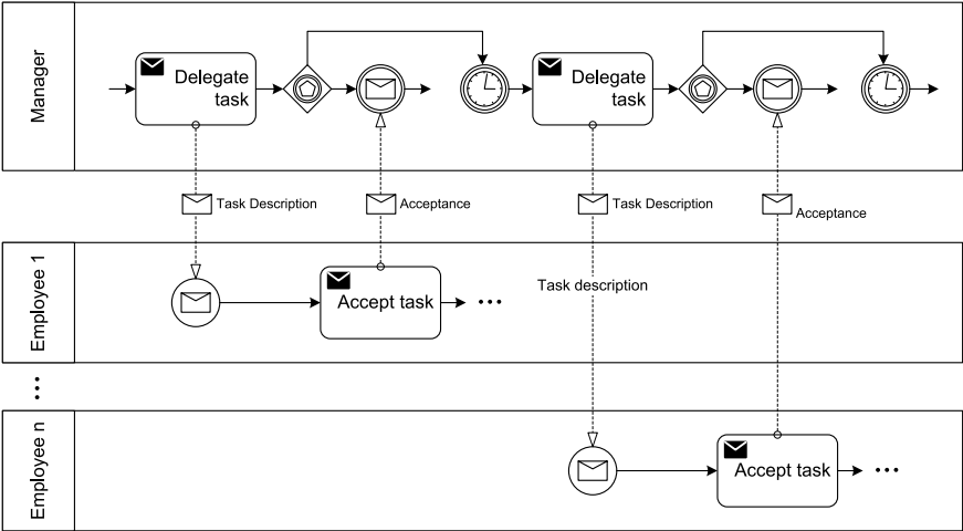
Fig. 5.29. Contingent requests pattern
