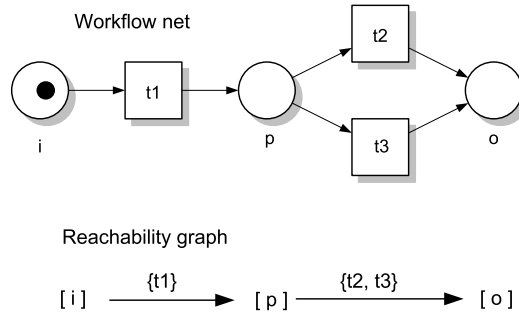
Fig. 6.10. Workflow net and corresponding reachability graph
