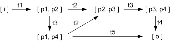
Fig. 6.15. Reachability graph of non-free-choice workflow net in Figure 6.14, showing its soundness
