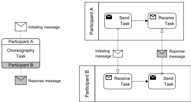
Fig. 5.39. Choreography task and corresponding process diagram
