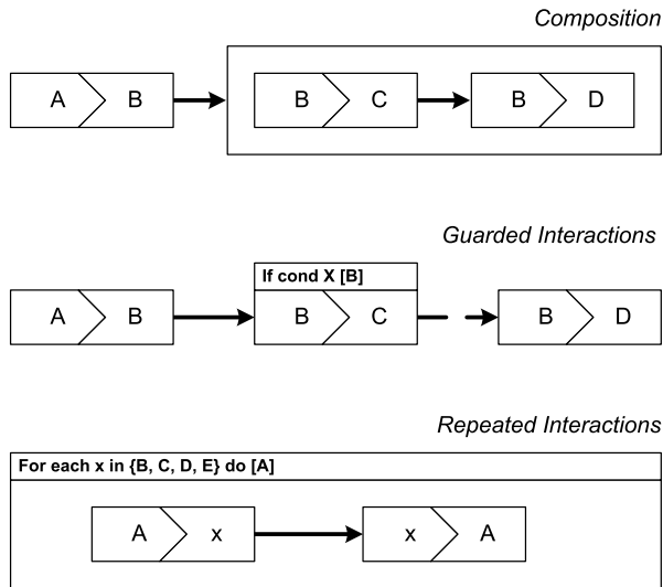
Fig. 5.35. Advanced control flow constructs
