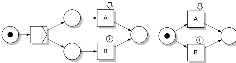
(a) Explicit xor split does not enable A and B concurrently
