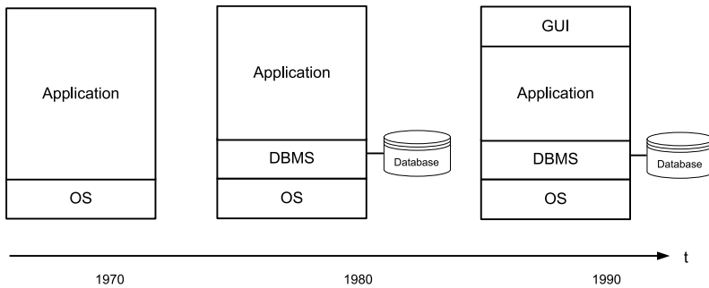
Fig. 2.1. Early systems architectures
