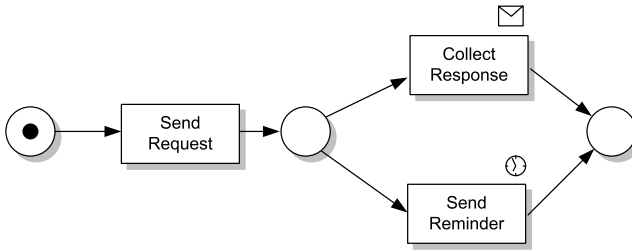
Fig. 4.48. Sample workflow net with external trigger and time trigger
