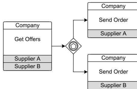
Fig. 5.47. Choreography diagram with event-based gateway
