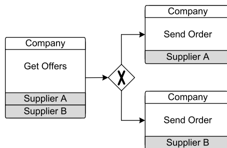
Fig. 5.44. Choreography diagram with exclusive gateway
