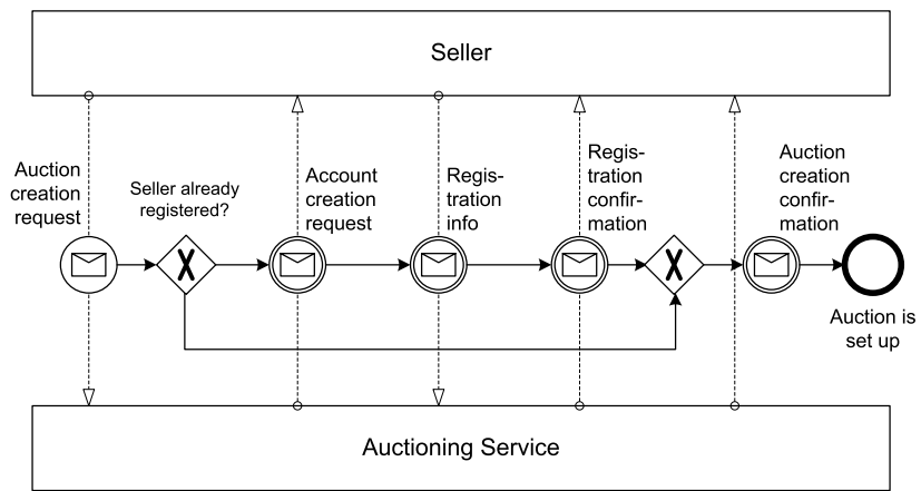
Fig. 5.8. Collaboration scenario: reaching milestones through interactions
