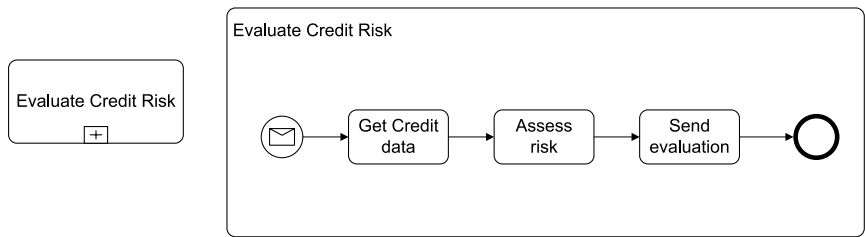
Fig. 4.80. Collapsed and expanded subprocess
