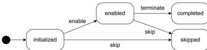
Fig. 5.33. Interaction instance lifecycle
