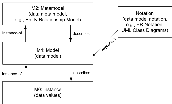
Fig. 3.22. MOF levels of modelling data
