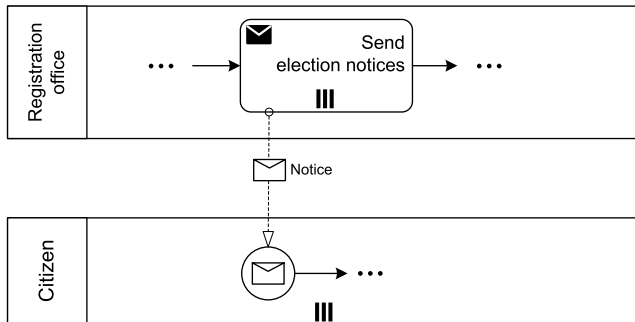
Fig. 5.26. One-to-many send pattern
