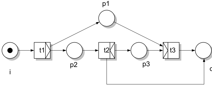
Fig. 6.9. Workflow net with deadlock/remaining tokens
