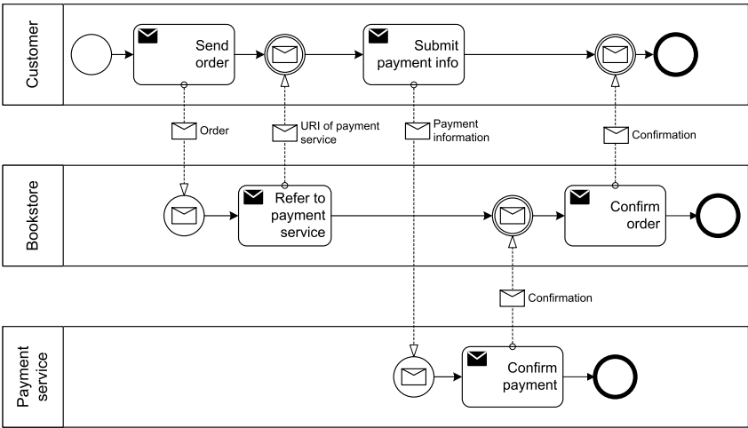
Fig. 5.30. Example involving request with referral pattern
