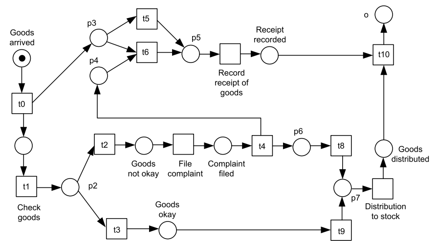
Fig. 6.19. Relaxed sound workflow net
