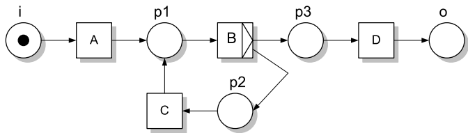
Fig. 6.11. Workflow net with loop
