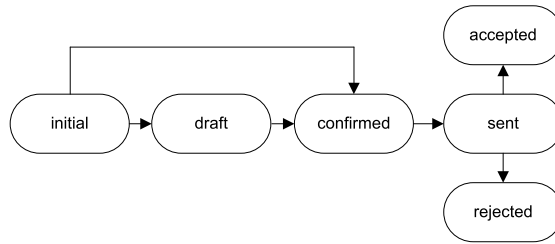
Fig. 6.3. Object lifecycle of quote object
