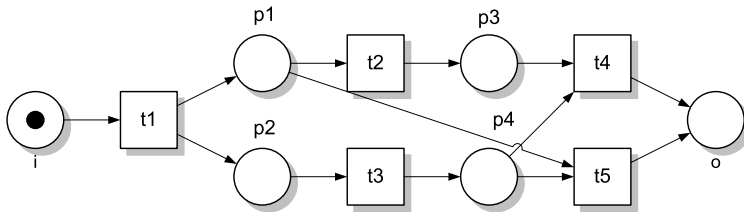
Fig. 6.14. Non-free-choice workflow net
