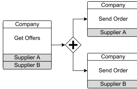
Fig. 5.49. Choreography diagram using parallel gateway
