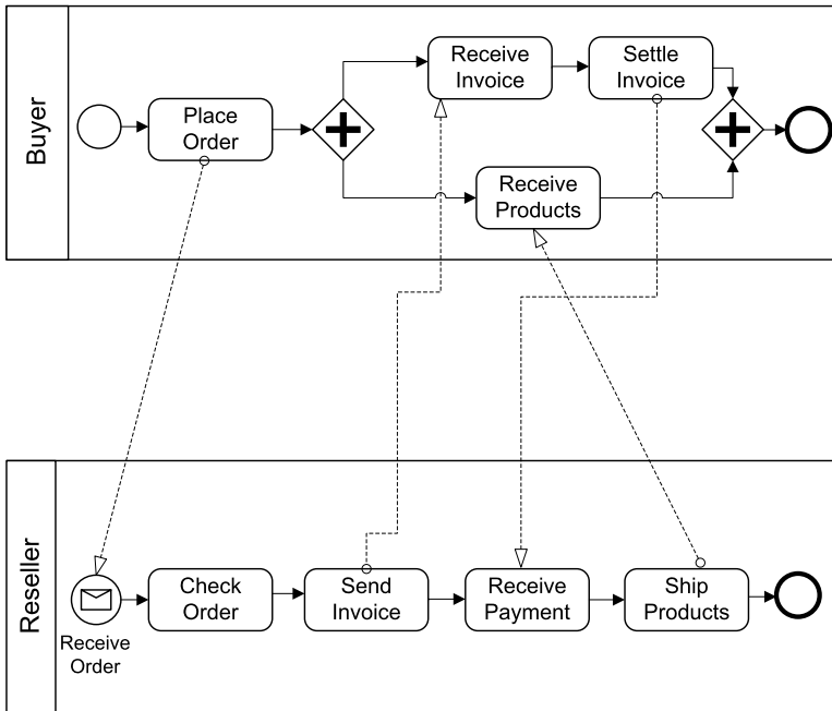
Fig. 3.20. Interacting business processes involving buyer and reseller
