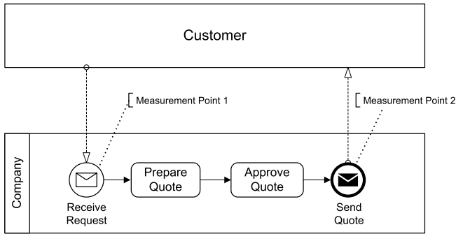
Fig. 8.7. Process diagram containing measurement points for key performance indicator IssueQuoteTime
