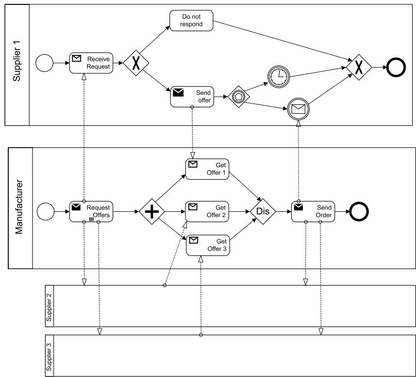
Fig. 6.25. Ordering process with discriminator pattern
