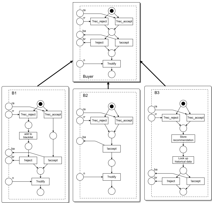
Fig. 5.17. Alternative implementations for buyer role
