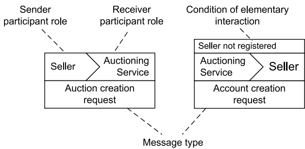
Fig. 5.31. Elementary interaction and conditional elementary interaction
