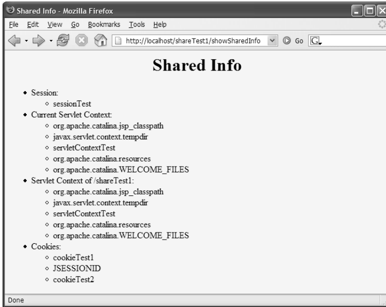
Figure 1–9 Result of visiting the SetSharedInfo and ShowSharedInfo servlets from within the same Web application.
