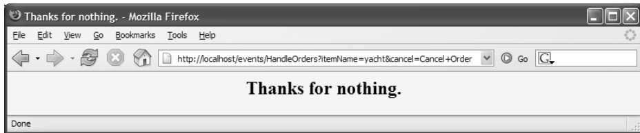
Figure 6-17 Result of cancelling an order. If the user had previously reserved an order for a yacht, the yacht-watching listener makes an entry in the log file (Listing 6.29) saying that a customer replaced a yacht order with something else.
