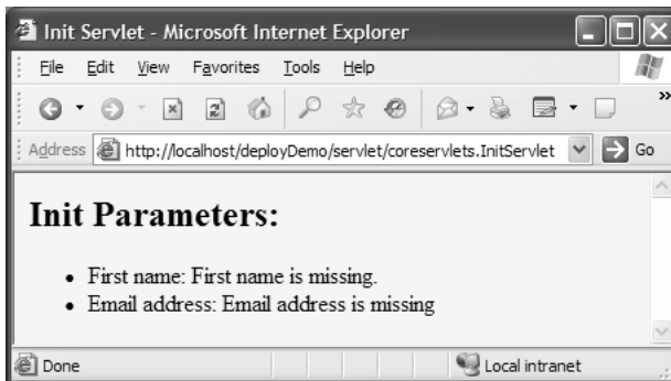
Figure 2-13 The InitServlet when incorrectly accessed with the default URL. Disable the invoker servlet to avoid this problem.
