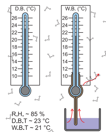
Figure 20.3 The wet-bulb reading is lower than the dry-bulb temperature when the relative humidity is less than 100%. The lower the humidity, the bigger the temperature difference.
