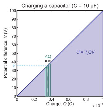
Figure 26.5 The energy stored in a 10 \mu\text{F} capacitor can be found from the area under the QV plot. As the capacitance is a constant, this plot is a straight line and the area is given by U = \frac{1}{2} QV .
