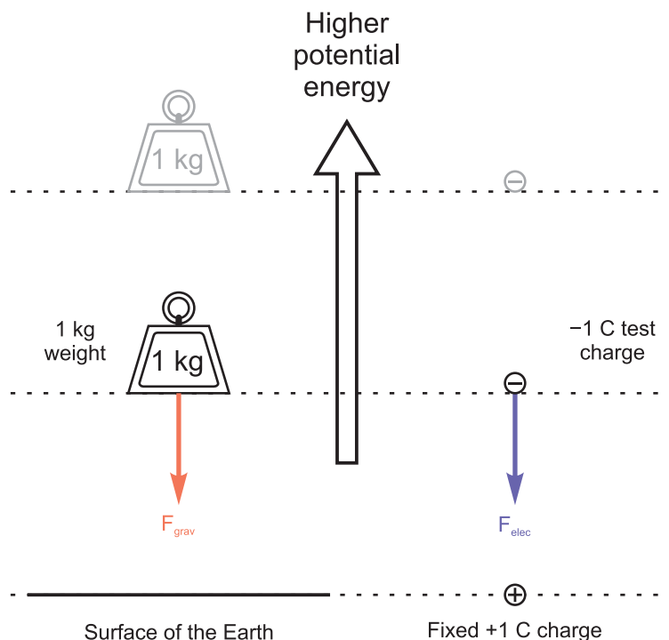
Figure 25.2 A useful analogy can be drawn between the concept of gravitational potential energy and electrical potential energy. Like most analogies it is imperfect, however. When considering electrical potential energy, we have both positive and negative charges which means both attractive and repulsive forces are possible, unlike gravitational potential energy, when all forces are attractive.
