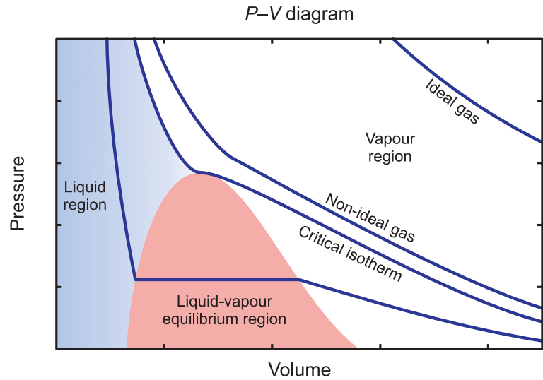
Figure 19.7 A typical P - V diagram, showing isotherms. In the region where the gas behaves like an ideal gas, the isotherms are hyperbolic in shape. At lower temperatures, the isotherms deviate from this behaviour. The critical isotherm has zero slope at the critical point.
