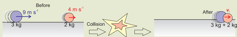
Figure 6.5 An example of a sticky inelastic collision.
