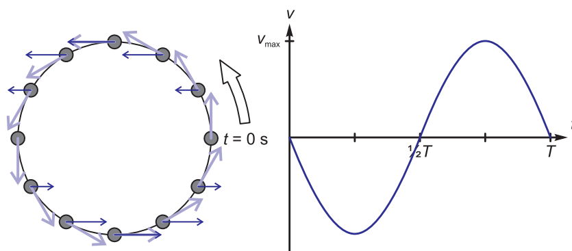
Figure 7.6 Plotting the x -component of the velocity (blue vector) on an object moving in a circle traces a sine graph that is 90^\circ out of phase with the position graph (see Fig. 7.4). In other words the velocity is at the maximum when the displacement from equilibrium is zero.
