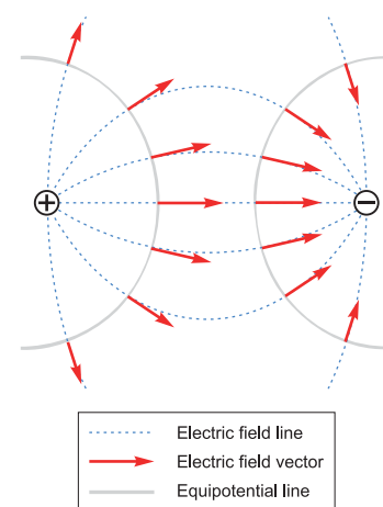
Figure 25.7 Electric field lines, electric field vectors, and equipotentials around an electric dipole. The electric field vector is perpendicular to the equipotential line that it lies upon. Note that the electric field strength is not the same at all points on a single equipotential line.
