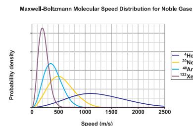
Figure 18.10 The Maxwell–Boltzmann distribution. This plot shows the distribution of speeds for some of the noble gases at 25 °C. [Public domain image from Wikipedia.]
