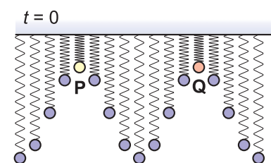
Figure 8.1 The relationship between SHM and wave propagation. The oscillators at P and Q are spaced one wavelength apart and are exactly in phase.
