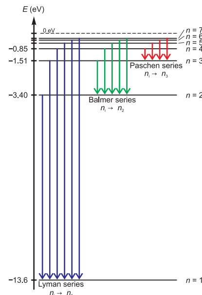
Figure 33.5 The electronic transitions which give rise to the hydrogen emission lines shown in Figure (33.4).
