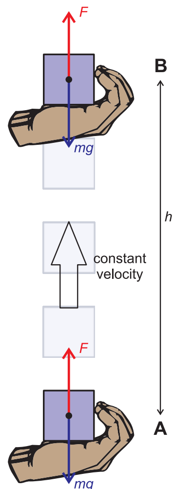
Figure 5.5 Derivation of gravitational potential energy
