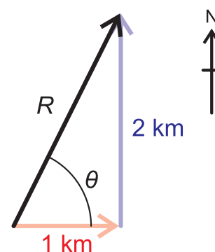
Figure B.6 A car travels 1 km due east and then 2 km due north. Adding a two vectros representing each part of the journey will enable us to find how far away and in what direction the car ends up.
