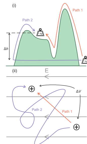
Figure 25.13 The work done by an external force to move (i) a mass up a hill and (ii) a charge in a uniform electric field depends only upon the start and end points. In the case of the mass, the work done on the weight must be W = mg\Delta h for either path, while for the charge it must be W = -q\Delta V .
