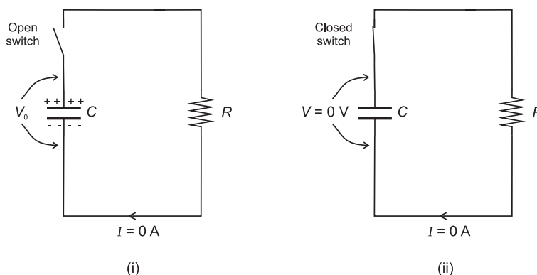
Figure 28.2 (i) The potential difference across the charged capacitor will cause a current to flow around the circuit. The current is proportional to the potential difference across the resistor (which is the same as that across the capacitor at all times). As current flows it reduces the potential difference across this resistor, which reduces the current and so on. (ii) After some time all of the charge on the capacitor is gone (there is zero potential difference across the capacitor) and there is no longer a current flowing around the circuit.
