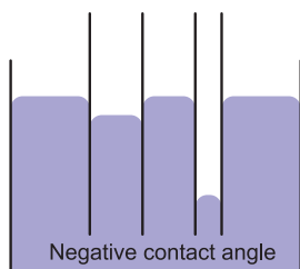
Figure 13.7 The distance the liquid travels up or down the tube is inversely proportional to the radius. In the case where the contact angle is greater than 90^\circ , the liquid surface is depressed.
