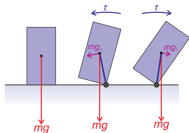
Figure 4.10 Illustrations of objects displaying static stability.
