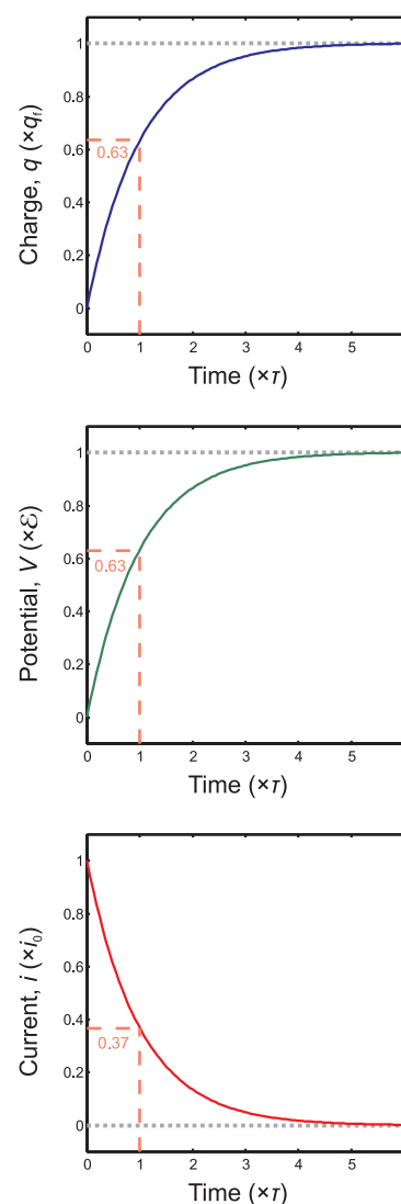
Figure 28.4 The charge on the capacitor, the electrical potential difference across the capacitor, and the current in the RC circuit as a function of time for a charging capacitor.
