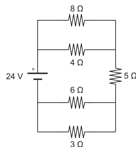
Figure 27.18 A circuit with 5 resistors in both series and parallel.
