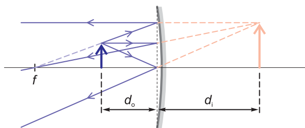
Figure 30.10 A virtual image formed by a converging mirror. Notice that the rays leaving the mirror are diverging as if coming from a point 'behind' the mirror. This image cannot be seen on a screen because at no point do the rays actually pass through that position.
