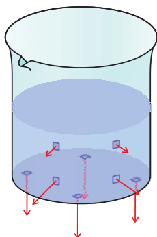
Figure 11.2 Fluid in a beaker exerts both sideways force on the vertical sides of the beaker and downwards force on the bottom of the beaker. The deeper the level of fluid, the larger the force exerted on adjacent small elements of the beaker. The force exerted on each small element is perpendicular to the surface of the beaker.
