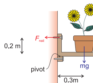
Figure 4.12 A vase sits on a shelf. The lower block acts like a pivot.
