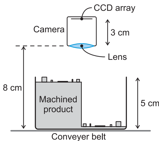
Figure 31.12 A machined product passing underneath an automated camera. The camera needs to be able to focus on all parts of the object (although not necessarily at the same time).
