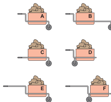
Figure 4.13 Six different ways of arranging a wheelbarrow.
