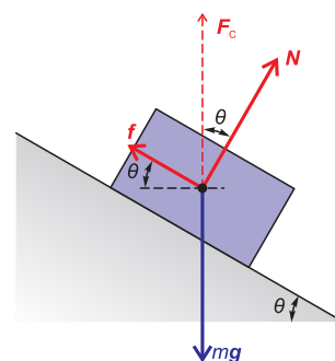
Figure 2.10 Surface contact force resolved into components perpendicular and parallel to the surface.
