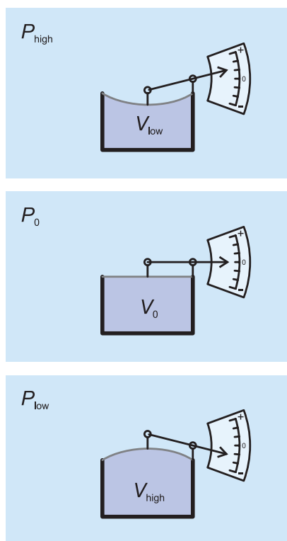
Figure 11.8 A simple mechanical diaphragm pressure meter. A sealed container holds some fixed amount of a gas. The container has at least one flexible surface, the diaphragm, which means that the pressure inside is always the same as that outside the container. As the pressure changes the volume of the gas inside the sealed container also changes (see the section on the Ideal Gas Law in Chapter 18 for an explanation of this) and the diaphragm bends. The degree and direction of the bending of the diaphragm indicate changes in pressure.
