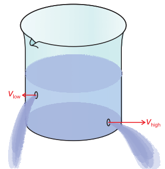
Figure 14.5 Two holes in a beaker full of fluid. The difference in pressure between surface and outlet creates a force that accelerates the fluid out of the hole. The greater the pressure difference, the higher the resultant velocity of the stream of fluid.
