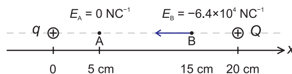
Figure 24.13 Two charges are placed 20 \text{ cm} apart. The magnitude of the electric field at point A is zero, while the electric field at point B is non-zero.
