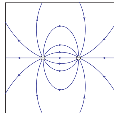
Figure 24.9 Electric field lines produced by equal magnitude positive and negative charges (electric dipole field). The Coulomb force on a positive charge placed on a electric field line always points along the line.
