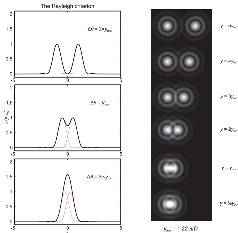
Figure 32.18 As the angular separation of two point-like objects viewed through some sort of circular aperture, be it a telescope or the human eye, gets smaller, the Airy patterns of the objects start to overlap. Eventually this results in an inability to definitively say that the two objects are separate from one another. (Left) Airy profile functions. (Right) Simulated Airy patterns through two small circular holes.
