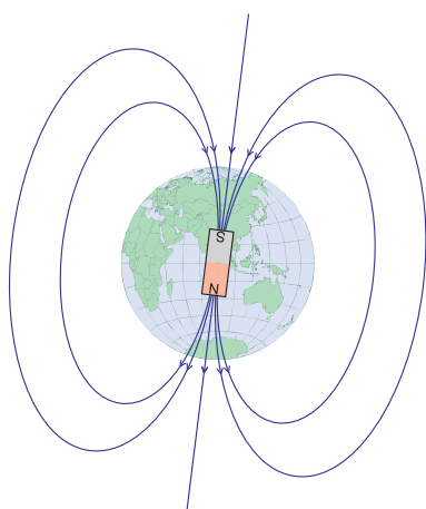
Figure 39.1 The Earth has a magnetic field that is shaped as though the Earth contained a giant bar magnet with its north pole somewhere under Antarctica. This is caused by currents in the Earth's iron core. This field is very important for protecting us from charged particles streaming in from space.
