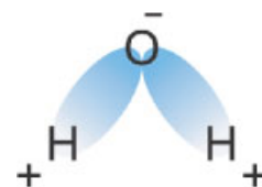
Figure 23.6 A simple representation of a very common permanently polarised molecule – the water molecule.
