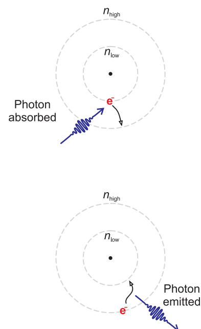
Figure 33.2 (Top) An atom can absorb the energy of a photon that strikes it by elevating one of its electrons to a higher energy level. (Bottom) Likewise an excited atom can lose energy by emitting a photon as an electron jumps to a lower energy level.
