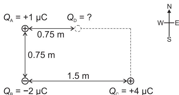
Figure 24.11 Three charges are arranged in 2 dimensions. What fourth charge will ensure that the net electrostatic force on charge B is zero?
