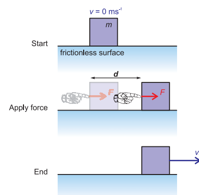
Figure 5.2 System used for derivation of kinetic energy formula.
