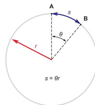
Figure 3.1 The relationship between the subtended angle and arc length.
