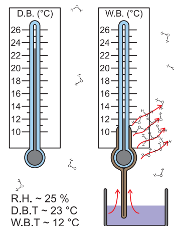
Figure 20.4 At lower humidity, the wet-bulb temperature is much lower than the dry-bulb temperature.
