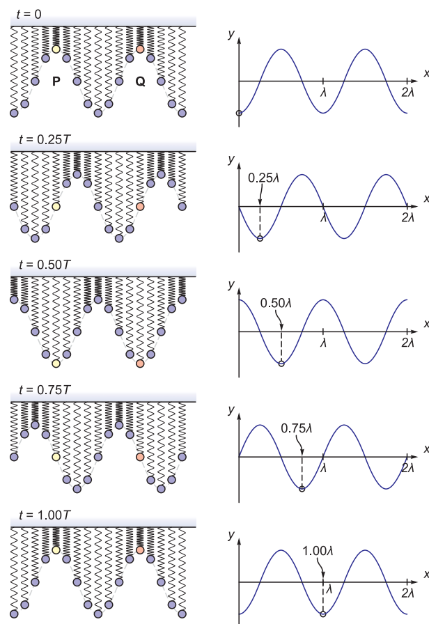
Figure 8.2 The propagation of a wave in a mass-spring system.
