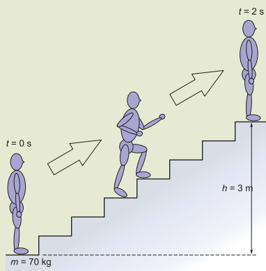
Figure 5.8 A man runs up a flight of stairs and gains 3 m of elevation in 2 s.
