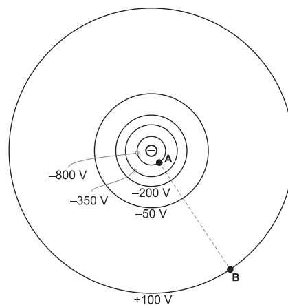
Figure 25.23 Equipotentials around an isolated point charge.
