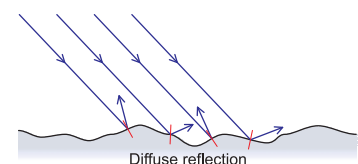
Figure 29.3 Specular reflection is when parallel light rays remain parallel after reflection. Smooth surfaces reflect in this manner. Diffuse reflection results is when parallel light rays are reflected at different, usually random, angles. Rough surfaces reflect in this manner.
