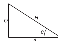
Figure B.2 A simple right-angled triangle. The longest side of the triangle (the hypotenuse) is labeled H . The side of the triangle opposite the corner labeled with the angle \theta is O , and the side adjacent to this angle is labeled A . The angle between the sides O and A must always be 90^\circ in a right-angled triangle.
