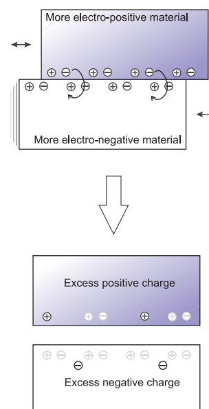
Figure 23.2 Rubbing two objects made of unlike materials together can result in charge transfer, leaving the object made of the most electropositive material with a net positive charge and the object made of the most electronegative material with a net negative charge. The total charge is conserved in this process; the two objects end up with equal and opposite charges.
