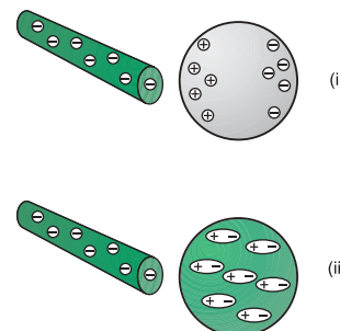
Figure 23.7 (i) Conductor: charges can move throughout the conductor and opposite charges accumulate on end of the conductor. (ii) Insulator: charges are still bound to a particular location in the insulator, but may spend more time on one side or other of a molecule.
