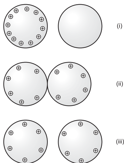
Figure 23.3 (i) A neutral conducting sphere (right) is brought close to an identical sphere with an excess positive charge (left). (ii) The two spheres are touched and the mobile charges redistribute over the surfaces of both, leaving both with an excess positive charge. (iii) The two spheres are separated, and each sphere has an excess positive charge of half the magnitude of the original excess charge on the left sphere.
