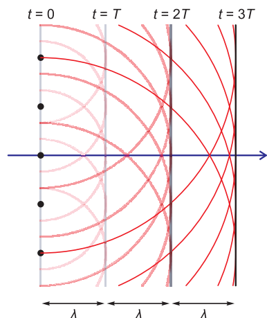
Figure 32.3 The application of Huygens' principle to the propagation of a plane wave in an isotropic medium. After one time period, T = 1/f , each wavelet has advanced radially by a distance equal to the wavelength of the wave, \lambda . Each wavelet will interfere constructively only along the straight line representing the translated wave front.
