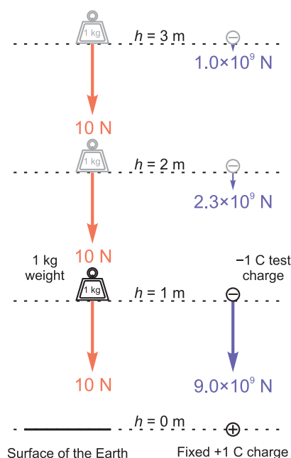
Figure 25.3 The gravitational force acting upon an object can be considered constant when one object is much more massive than the other and only is moved over a short distance. In most cases such a simplification cannot be made for the electrostatic force between two charges, so we will restrict ourselves mostly to the simple case of a uniform electric field.
