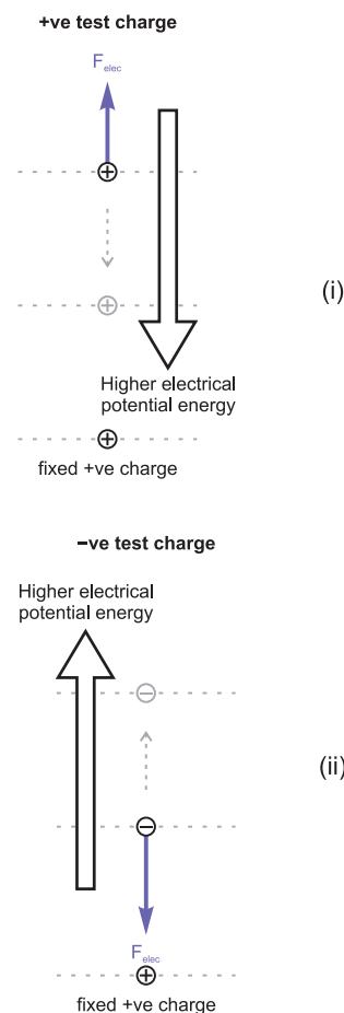
Figure 25.1 (i) Moving two 'like' charges closer together increases the electrical potential energy of each charge. (ii) Moving two 'unlike' charges further apart increases the electrical potential energy of each charge
