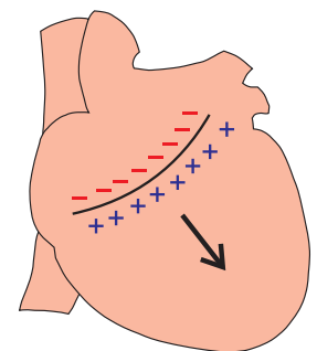
Figure 25.17 The depolarisation wave sweeps down the heart.
