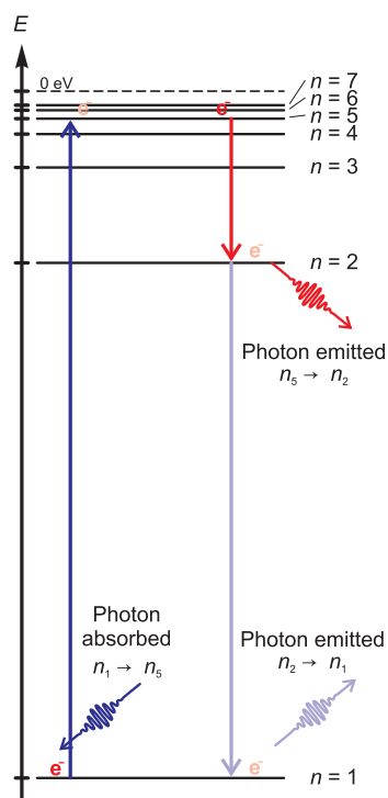
Figure 33.3 Atomic electrons make transitions up or down the energy level structure of an atom by emitting or absorbing photons of the appropriate energy.
