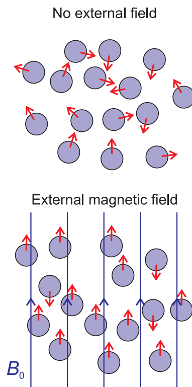
Figure 39.14 In the presence of a static magnetic field, more protons align with the field than against it.
