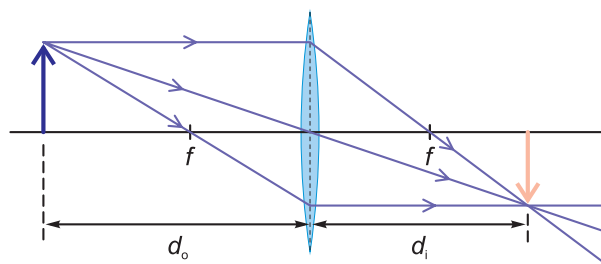
Figure 30.14 A real image formed by a converging lens. Notice that the rays leaving the lens are converging towards a point. If a screen were placed here, an image of the object could be seen on it.
