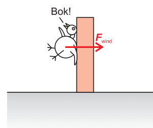
Figure 2.13 A chicken is blown into a wall.
