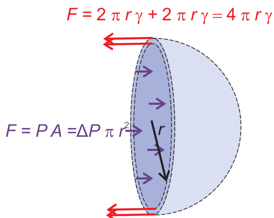
Figure 13.3 The pressure inside a hollow bubble. The total force pulling on the surfaces is twice the circumference times the surface tension. The net force over the hemispherical surface is the pressure times the cross-sectional area.
