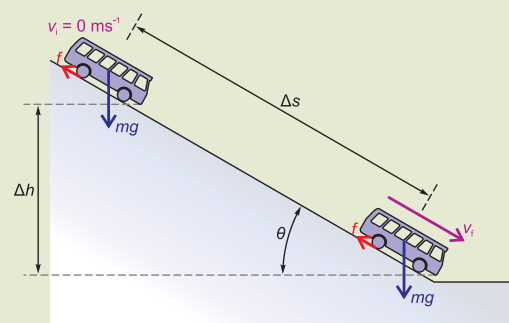
Figure 5.7 The effect of friction in energy calculations.
