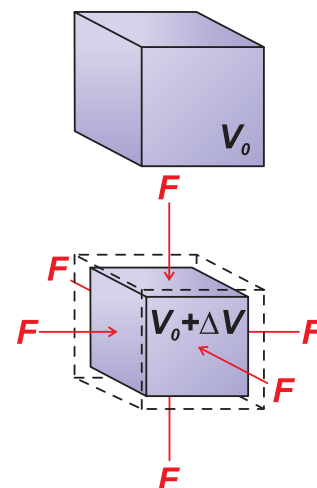
Figure 10.5 A compressive (or tensile) force acting in three dimensions can cause a change in volume of an object. In this example, a positive pressure change produces a negative bulk stress, and a negative volume strain, hence the decrease in volume ( \Delta V is negative).
