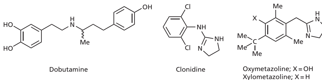
FIGURE 23.15 Adrenergic agonists.
