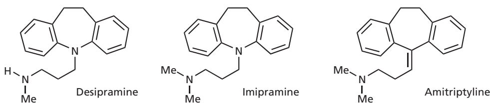
FIGURE 23.36 Tricyclic antidepressants.
