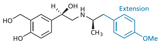
FIGURE 23.18 (R)- Salmefamol.
