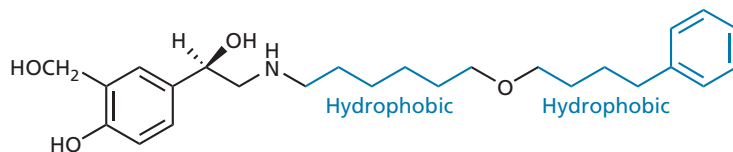
FIGURE 23.19 (R)- Salmeterol.
